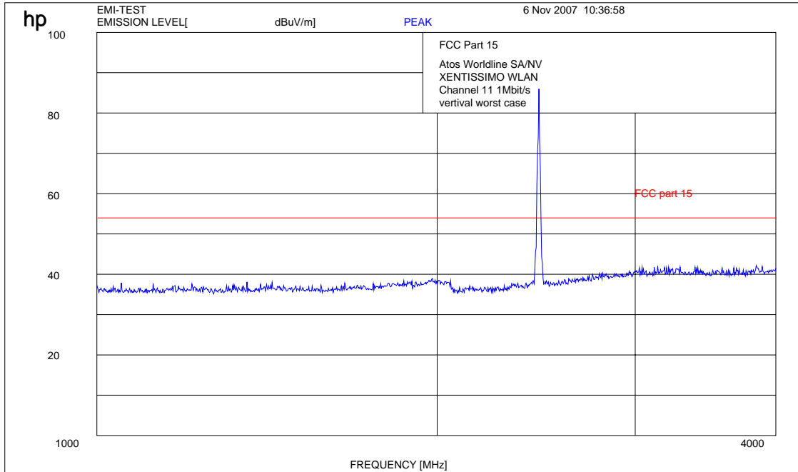
Plot 9: 1- 4 GHz (highest channel)
