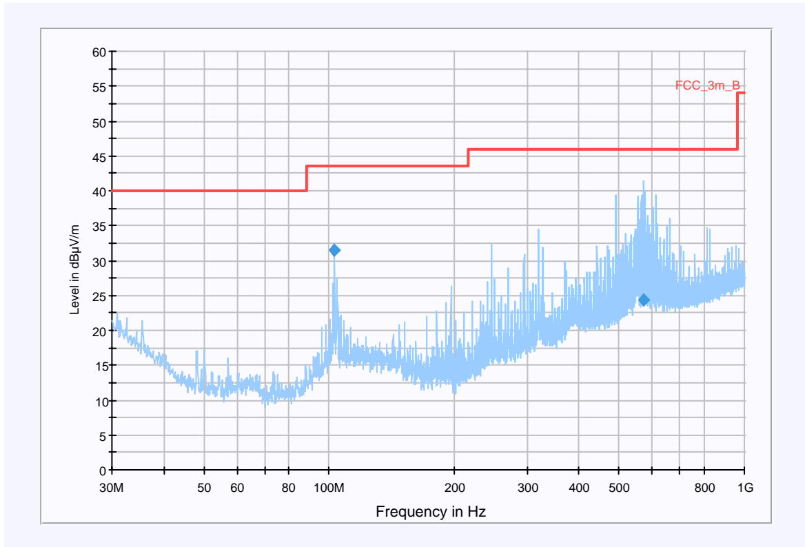
Plot 5: 0.03 - 1 GHz vertical / horizontal (middle channel)
