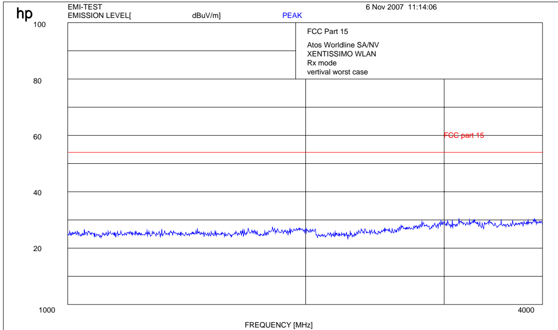
Plot 2: 1 - 4 GHz vertical / horizontal (receiver)
