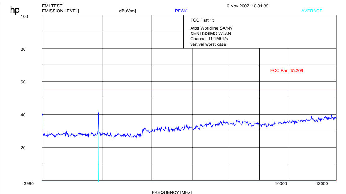
Plot 10: 4- 12 GHz (highest channel)
