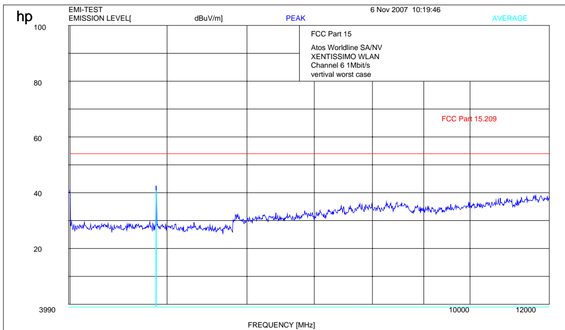
Plot 7: 4- 12 GHz (middle channel)
