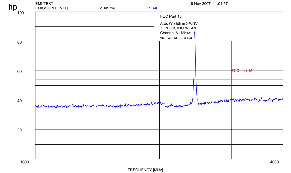
Plot 6: 1- 4 GHz (middle channel)
