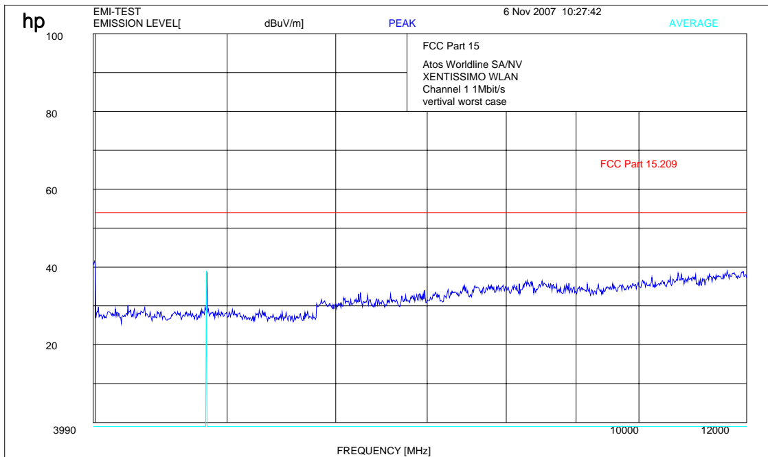
Plot 3: 4- 12 GHz (lowest channel)
