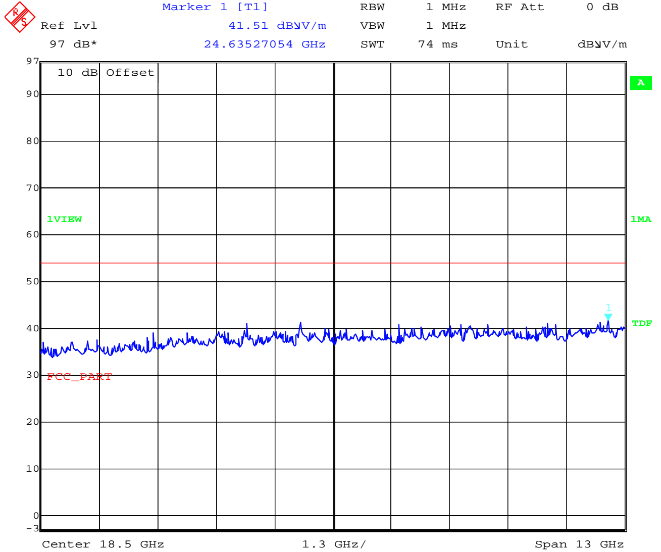
Plot 4: 12- 25 GHz (receiver)
