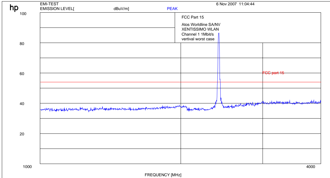
Plot 2: 1- 4 GHz (lowest channel)
