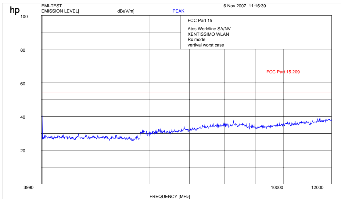
Plot 3: 4- 12 GHz (receiver)
