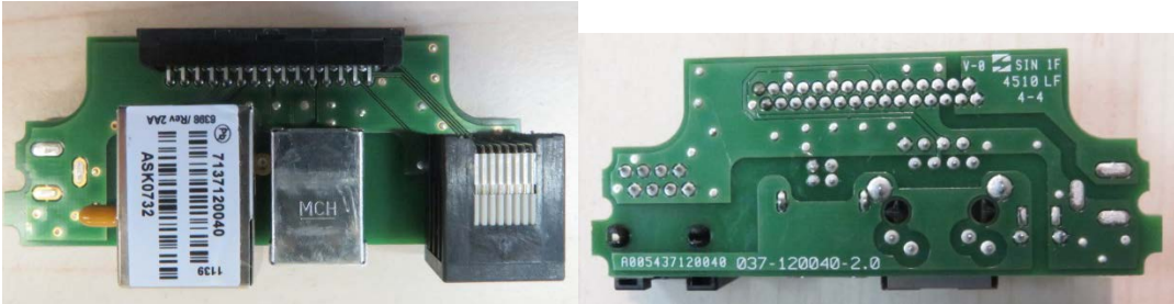
YOMANI TOUCH/ML I/O connector 037-120040
