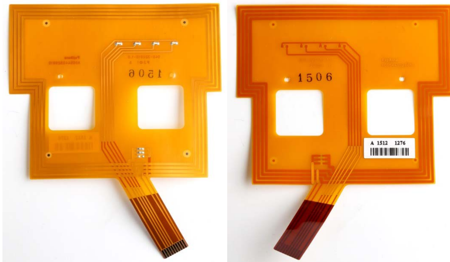
YOMANI ML/XR/TOUCH NFC Antenna 040_320010
