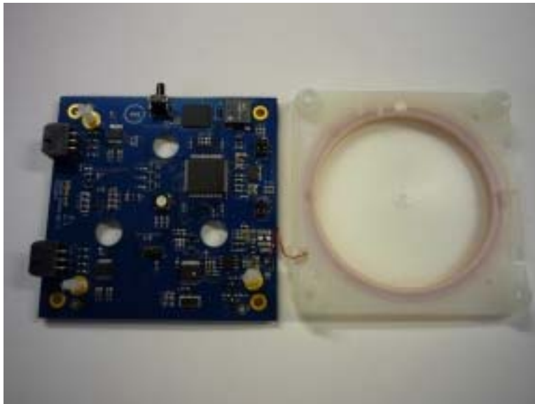
Figure 2 ZpassV2 w/antenna unmounted
