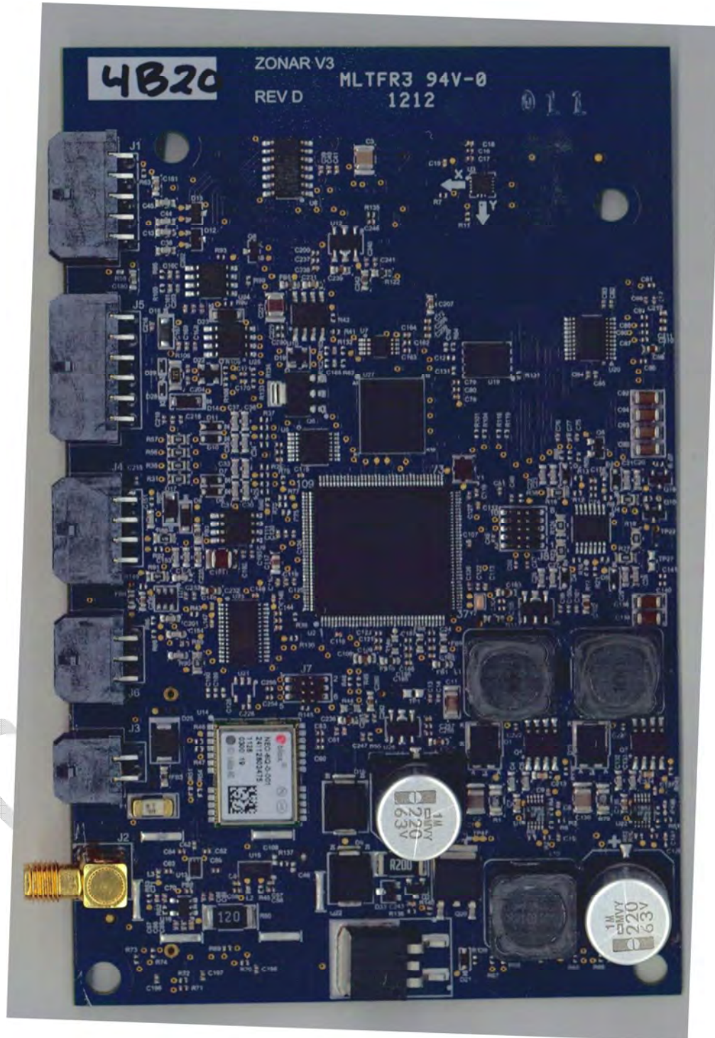
Figure 1 V3 Component/Bottom Side
