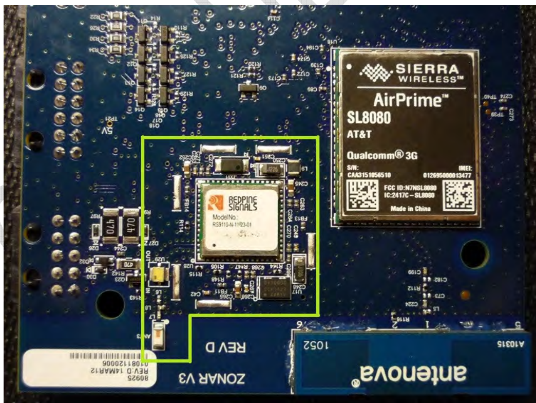
Figure 4 V3 WiFi radio Sub-Circuit
