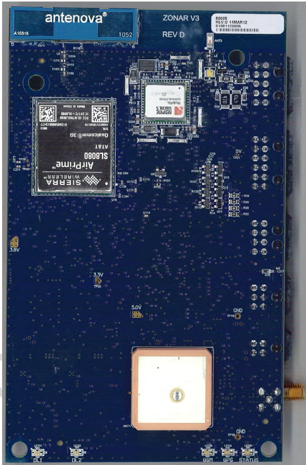
Figure 2 V3 Antenna/Top Side
