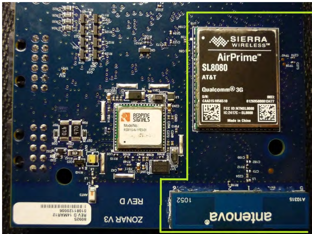
Figure 3 V3 GSM Radio Sub-Circuit
