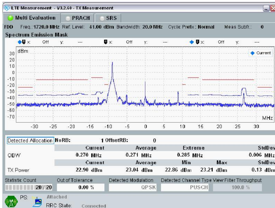
20MHz Band Width: Ch 20050, RB Size=1; RB Offset = 0
