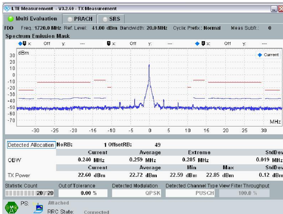
20MHz Band Width: Ch 20050, RB Size=1; RB Offset = 49
