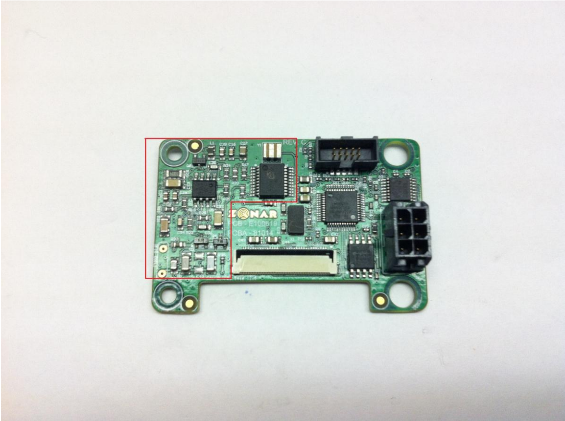
Figure 3 Virtual Trainer PCB top. Radio section bounded in RED
