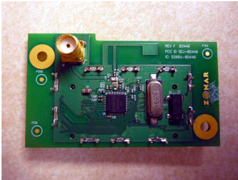
Figure 3 80446A shield removed
