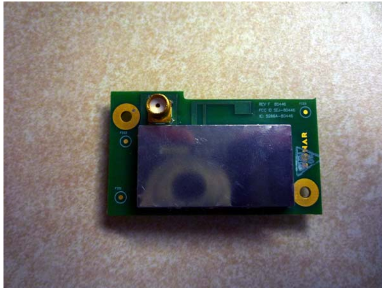
Figure 1 80446 with unique antenna connector and trace antenna
