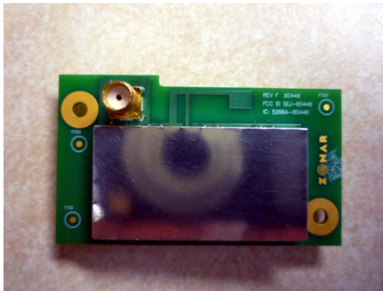
Figure 1 80446 Radio Module Front
