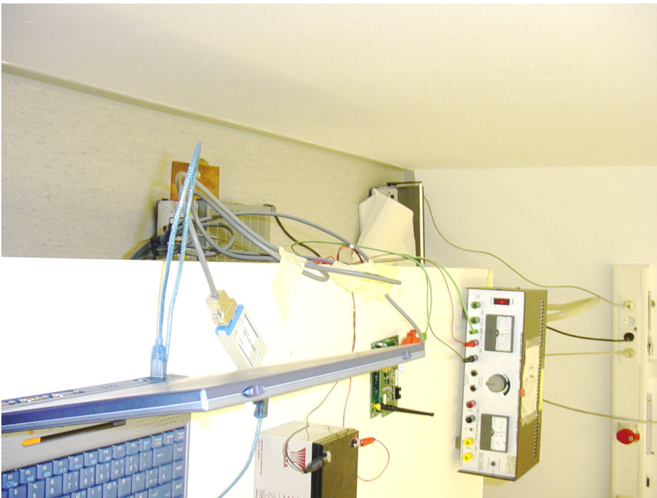
Photo 2.2 Conducted emissions test set-up; side view
