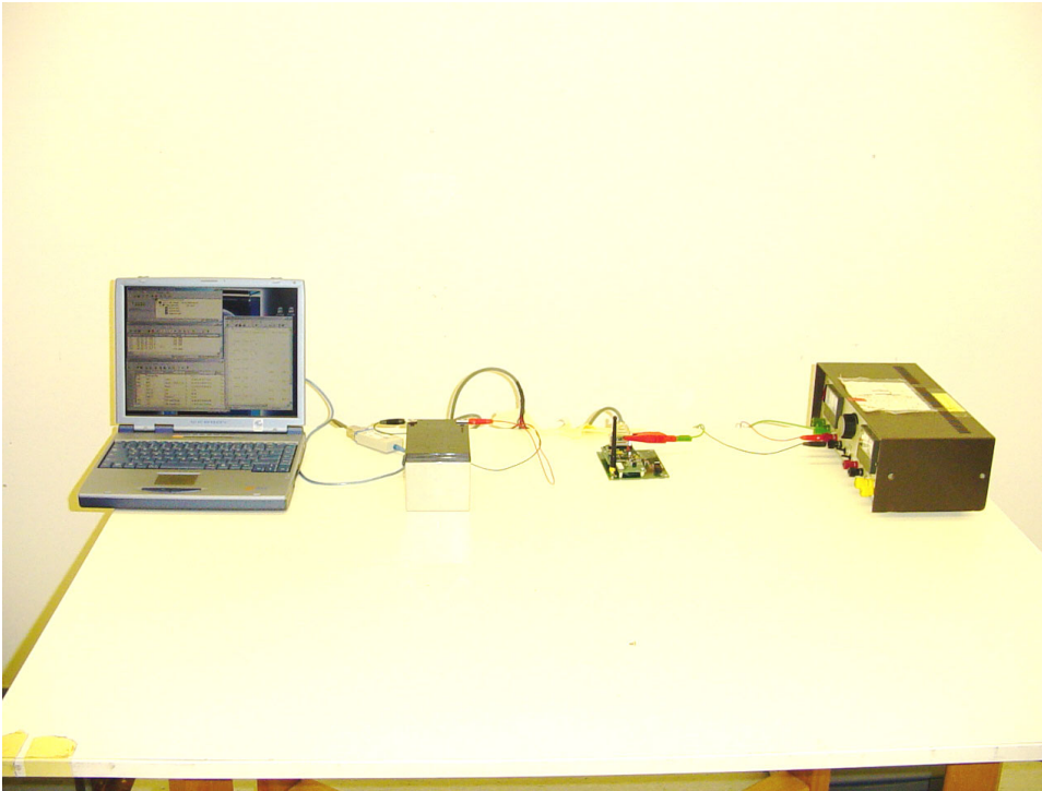
Photo 2.1 Conducted emissions test set-up; front view
