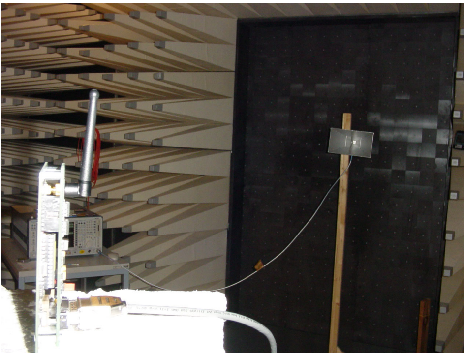
Photo 1.2 Radiated emissions test above 1 GHz; example set-up with Rod Antenna: Emissions test 1 – 18 GHz
