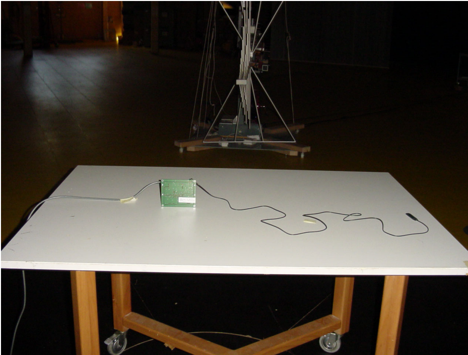
Photo 1.1 Radiated emissions test below 1 GHz; example set-up with Blade Antenna
