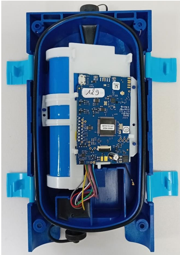
Device without communication daughter board
