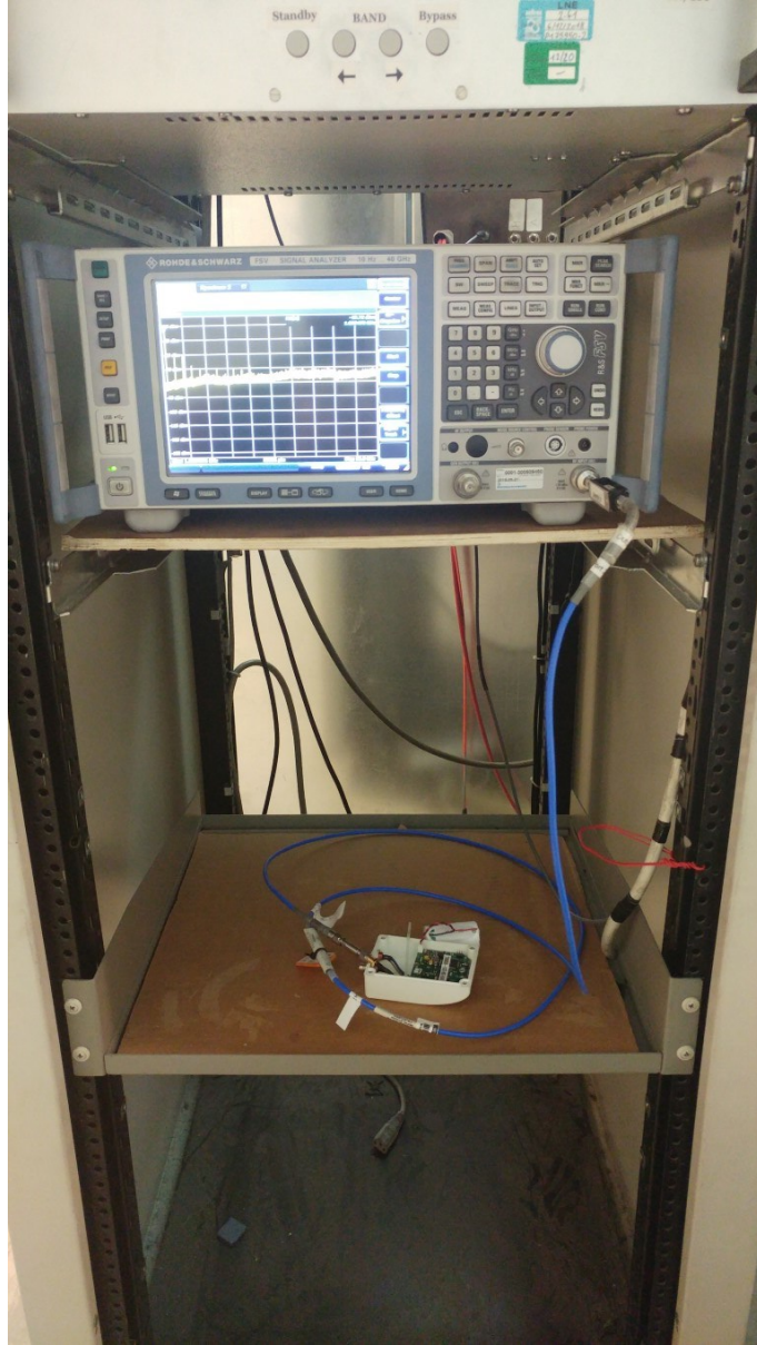
Photograph for Unwanted Emission into non-restricted frequency bands
