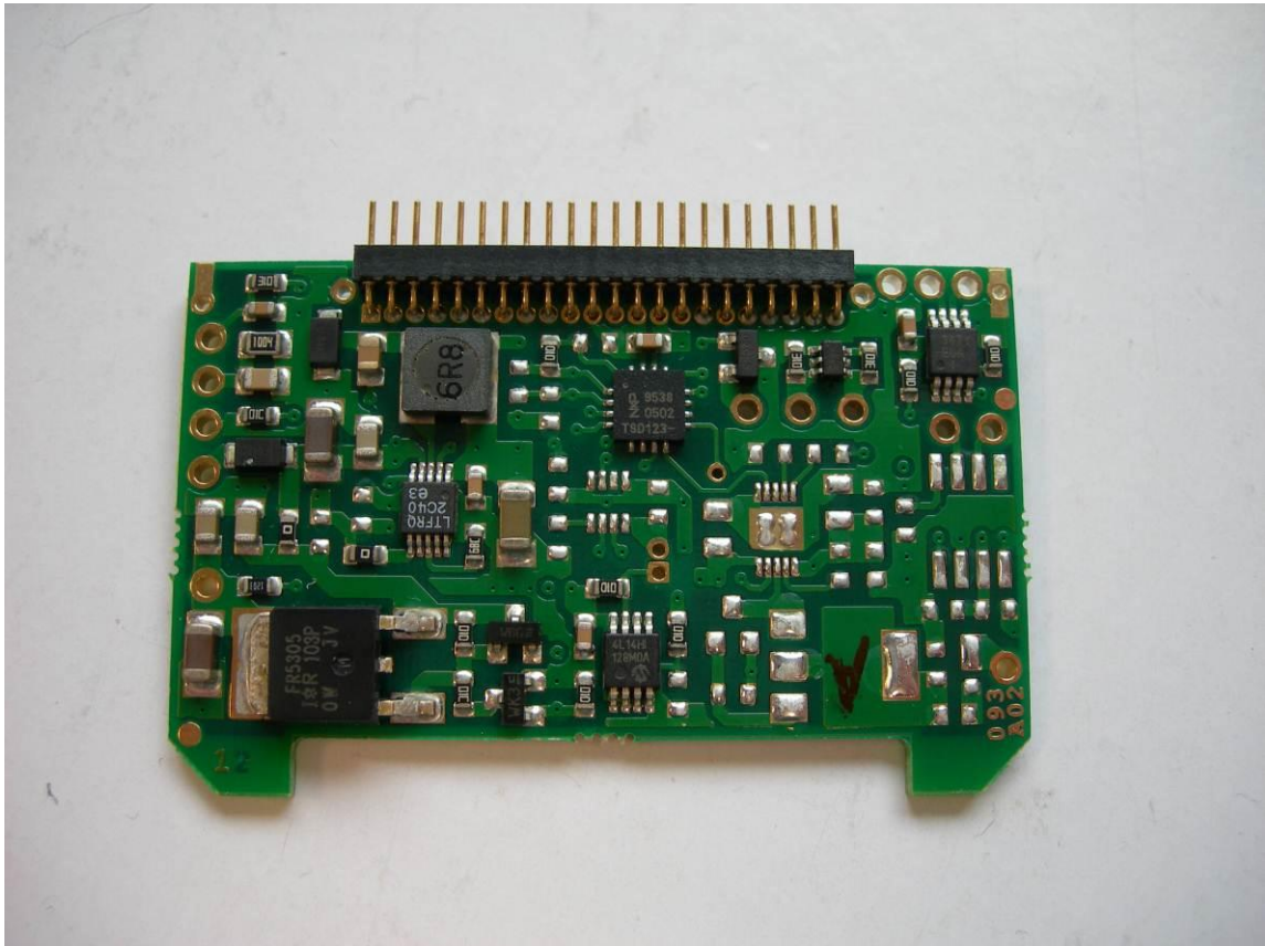
Modbus daughterboard
