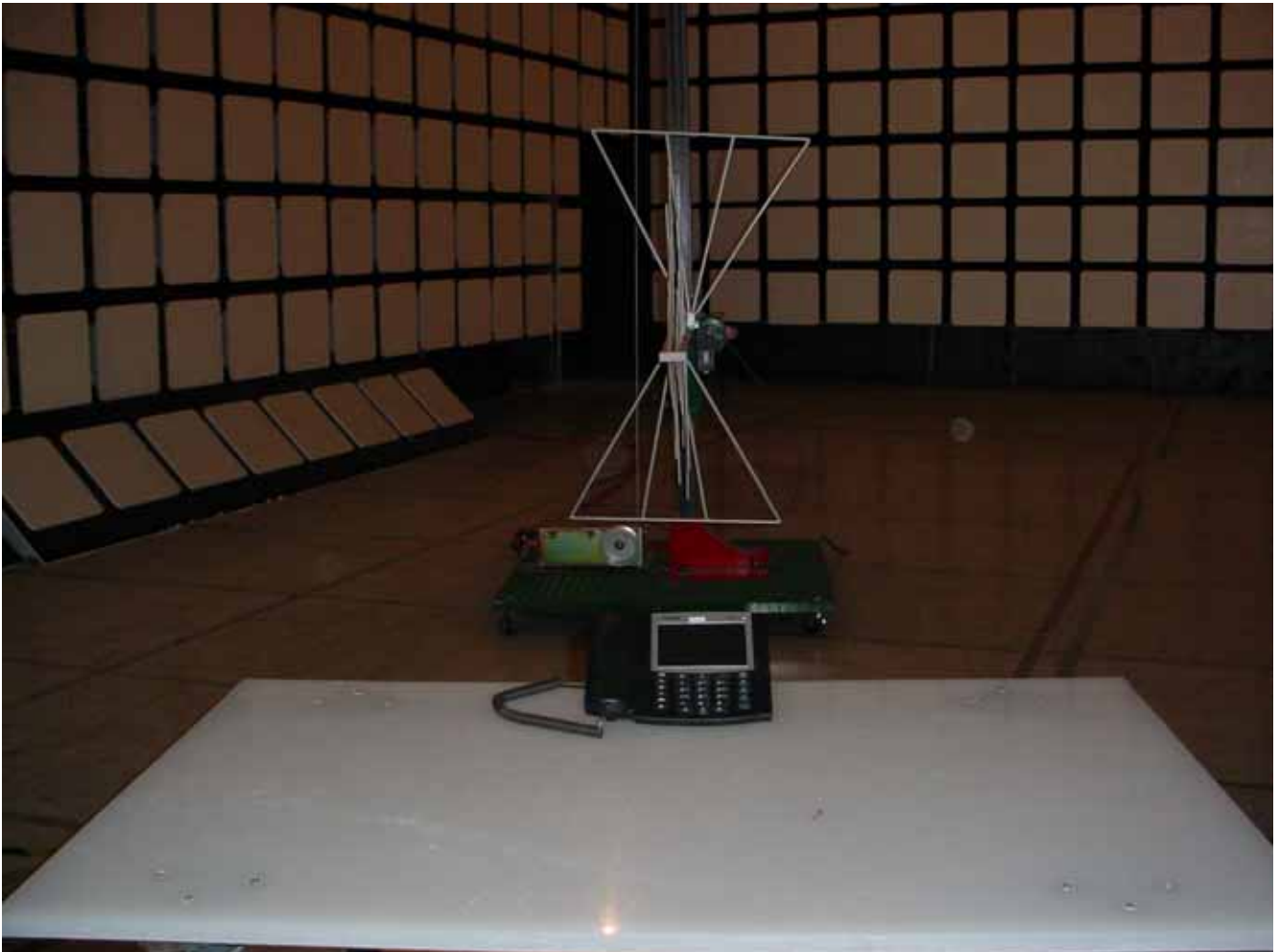
< Radiated Emissions Test >
