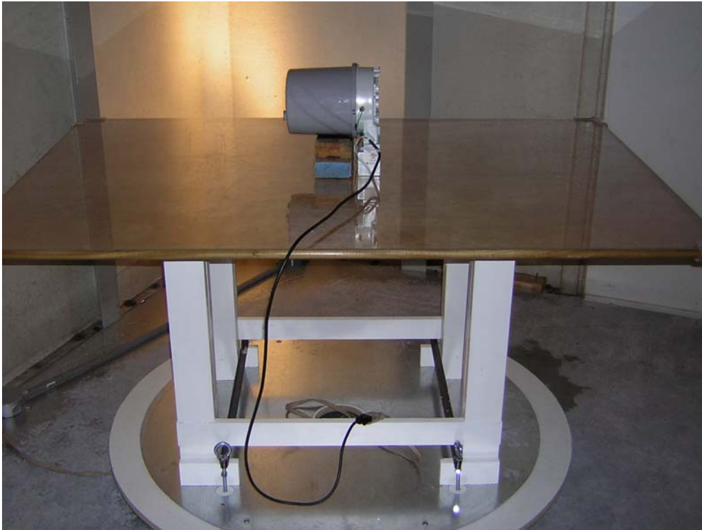
Radiated Emissions
