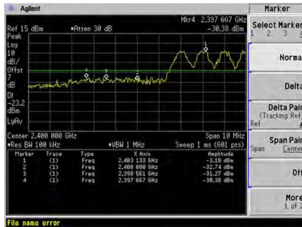
GFSK Hopping BAND EDGE (LOW)
