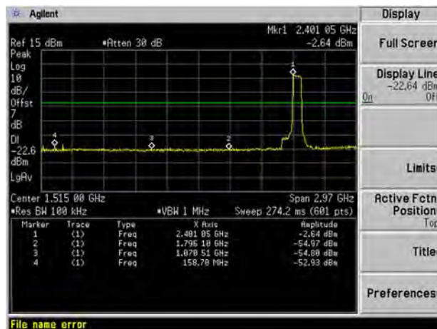
GFSK Hopping Mode, SPURIOUS 30 MHz ~ 3 GHz
