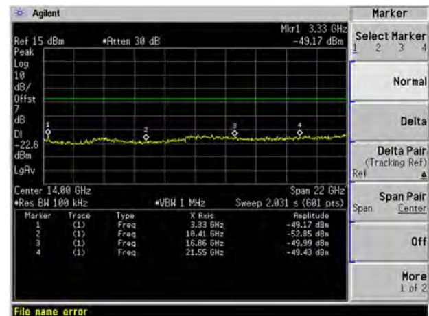
GFSK Hopping Mode, SPURIOUS 30 3GHz ~ 25 GHz
