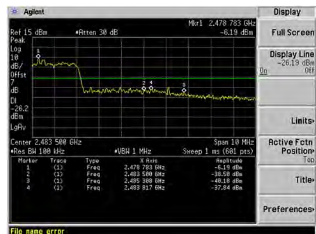
II/4-DQPSK Hopping BAND EDGE (HIGH)
