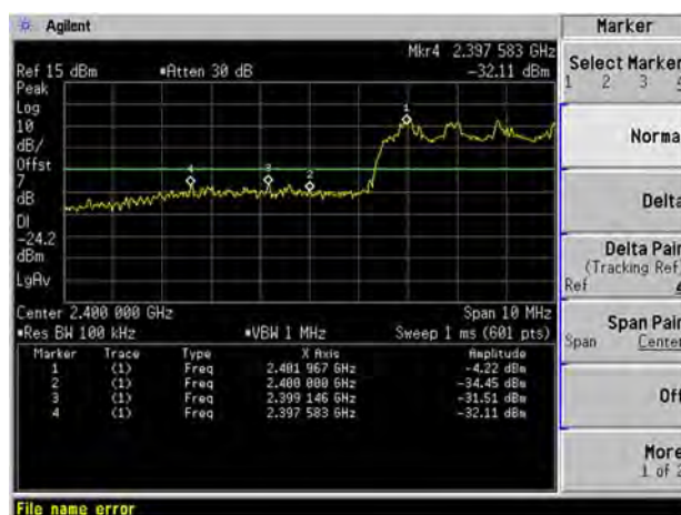
II/4-DQPSK Hopping BAND EDGE (LOW)
