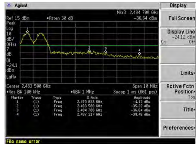
GFSK Hopping BAND EDGE (HIGH)
