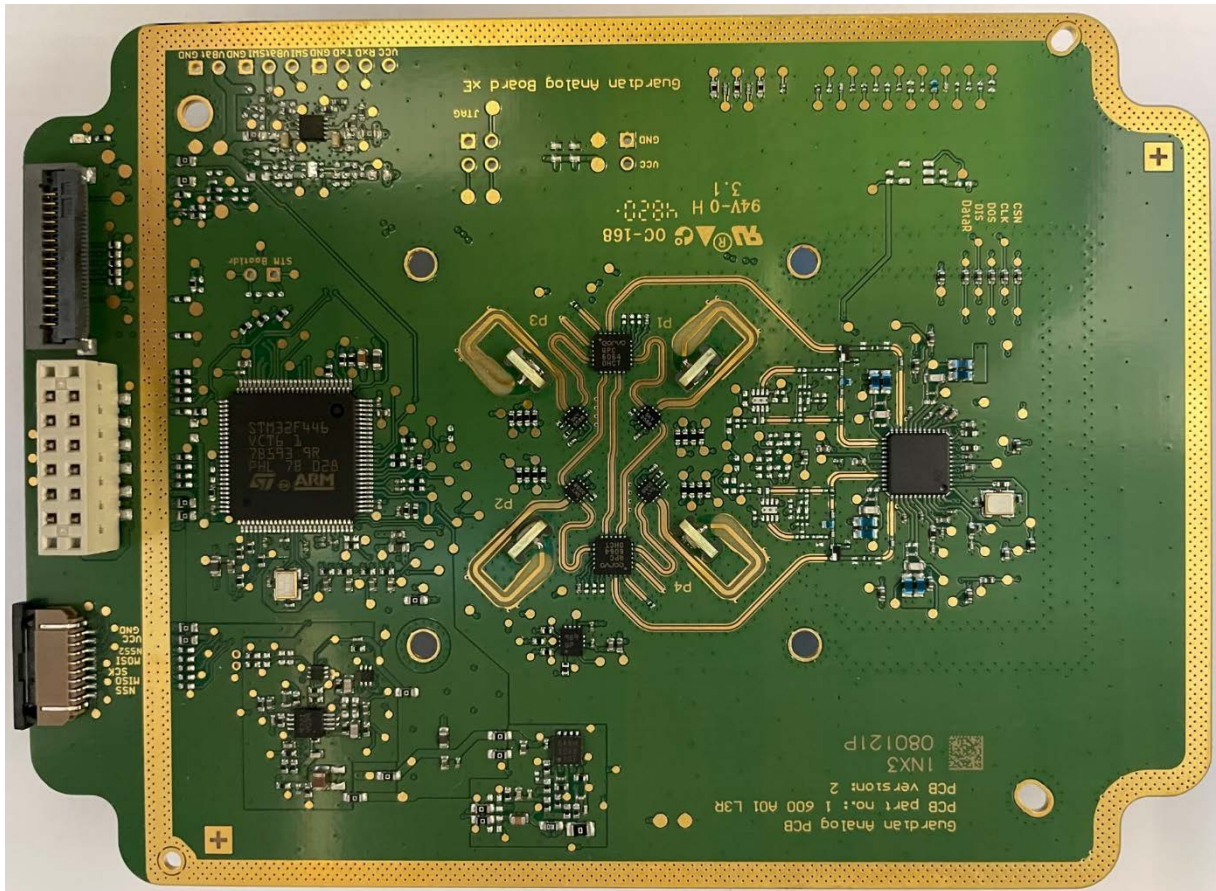
Analog Signal PCBA
