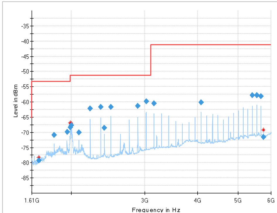
Plot 2: Fundamental emissions (EUT2): RMS
