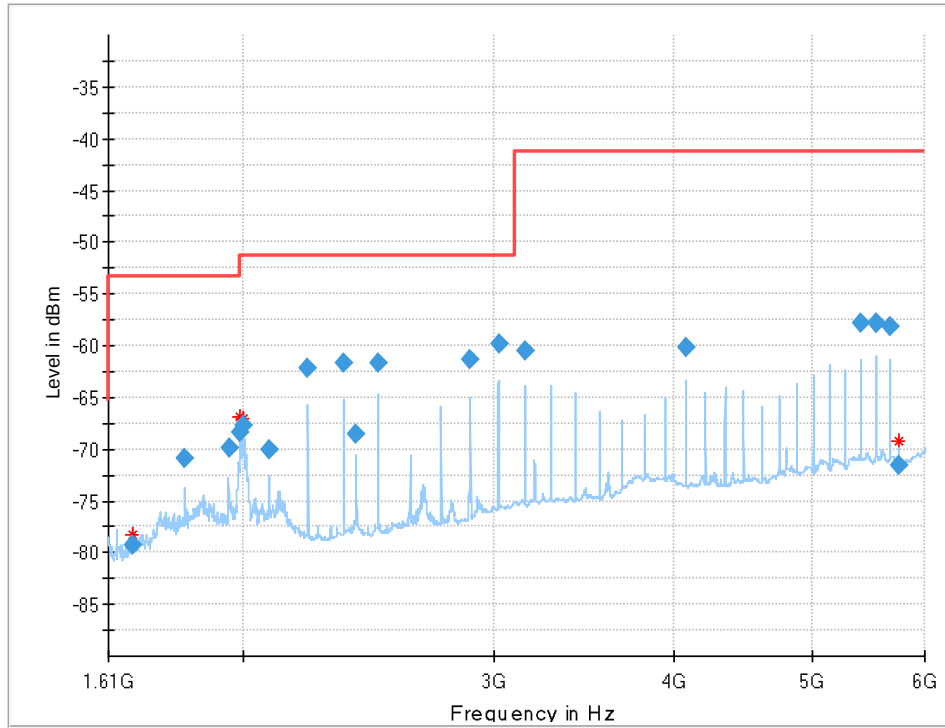
Plot 7: 1.61 GHz to 6 GHz, EUT2
