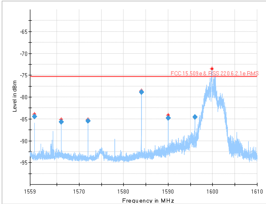
Plot 13: 1559 MHz to 1610 MHz (§15.509 (e), RSS-220 6.2.1(e)), EUT2
