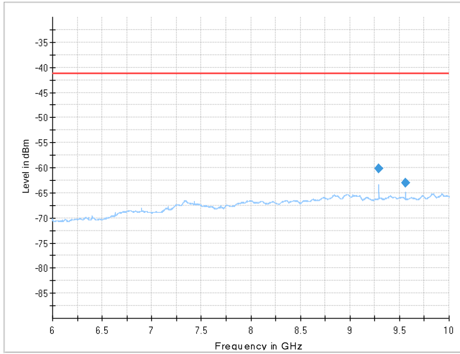
Plot 8: 6 GHz to 10 GHz, EUT2
