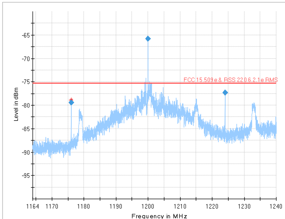
Plot 15: 1164 MHz to 1240 MHz (§15.509 (e), RSS-220 6.2.1(e)), EUT 3 (UWB off)
