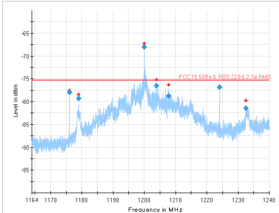
Plot 12: 1164 MHz to 1240 MHz (§15.509 (e), RSS-220 6.2.1(e)), EUT2
