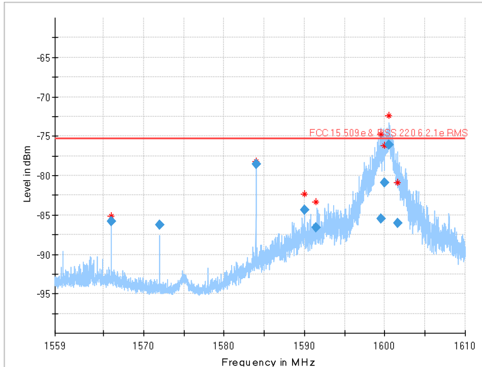
Plot 16: 1559 MHz to 1610 MHz (§15.509 (e), RSS-220 6.2.1(e)), EUT 3 (UWB off)
