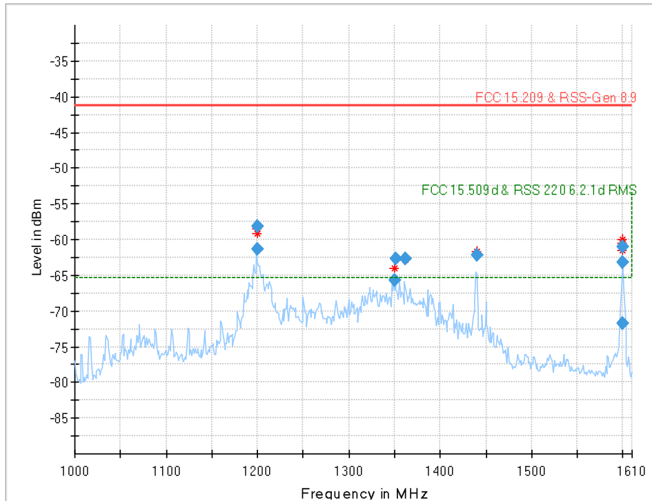
Plot 6: 1 GHz to 1.61 GHz, EUT2
