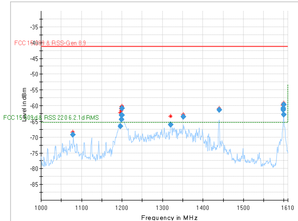
Plot 14: 1000 MHz to 1610 MHz, EUT 3 (UWB off)
