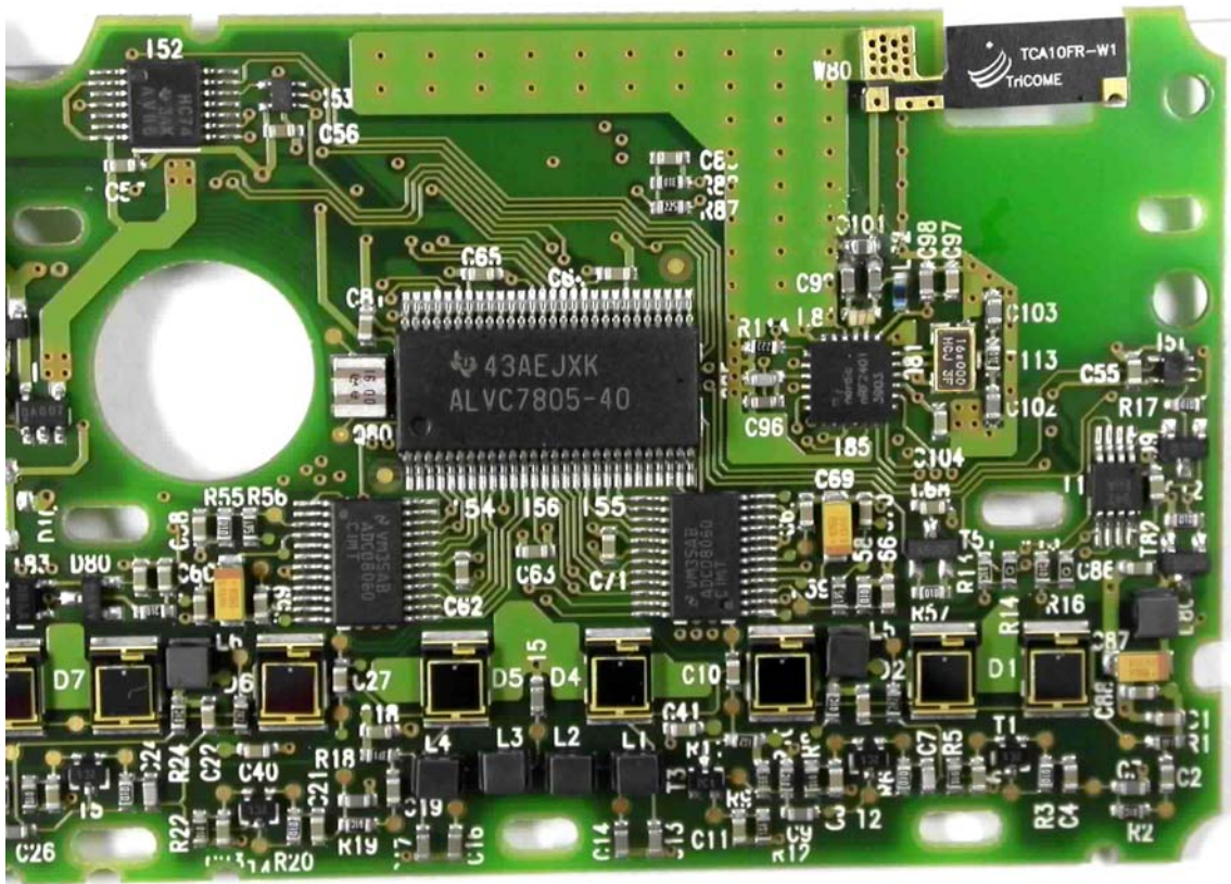
Internal Photo Part of Front view PCB
