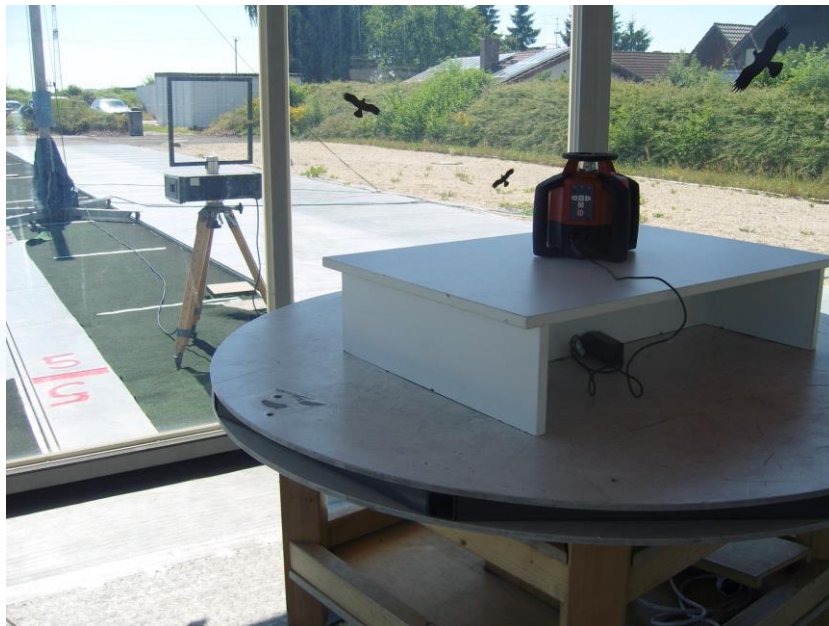
OATS1 (30 - 1000 MHz)
