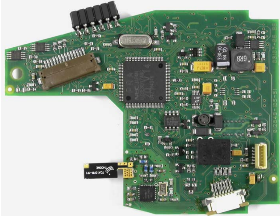
Internal Photo Front view PCB
