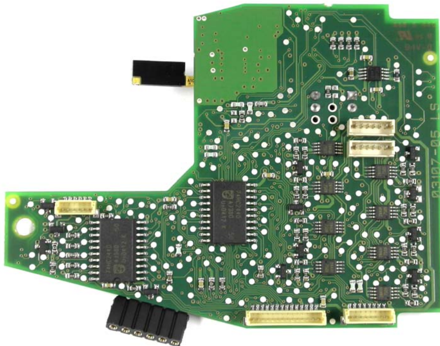
Internal Photo Rear view PCB
