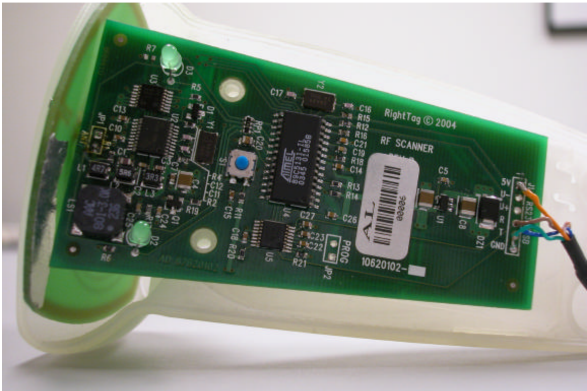
Top of casing removed
