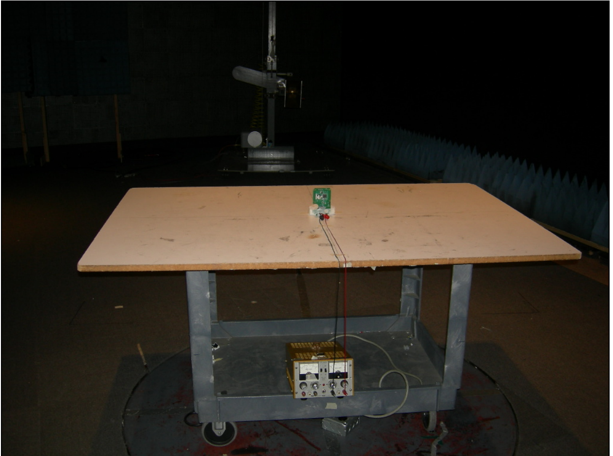
Figure 2: Radiated Emissions
