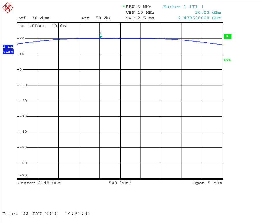
Figure 7.5.2-3: Output power – High Channel
