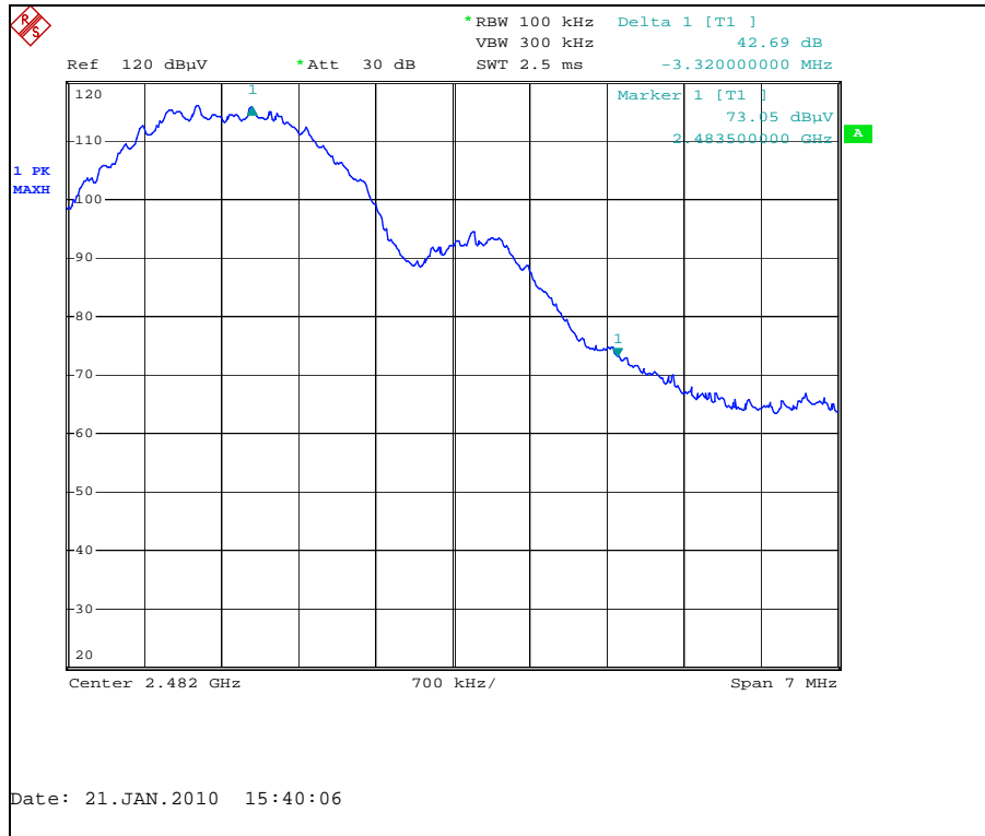
Figure 7.6.1.2-2: Upper Band-edge– Vpol
