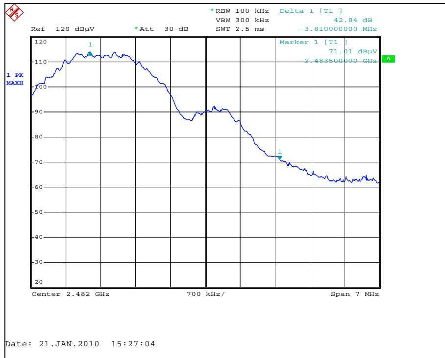
Figure 7.6.1.2-1: Upper Band-edge – Hpol
