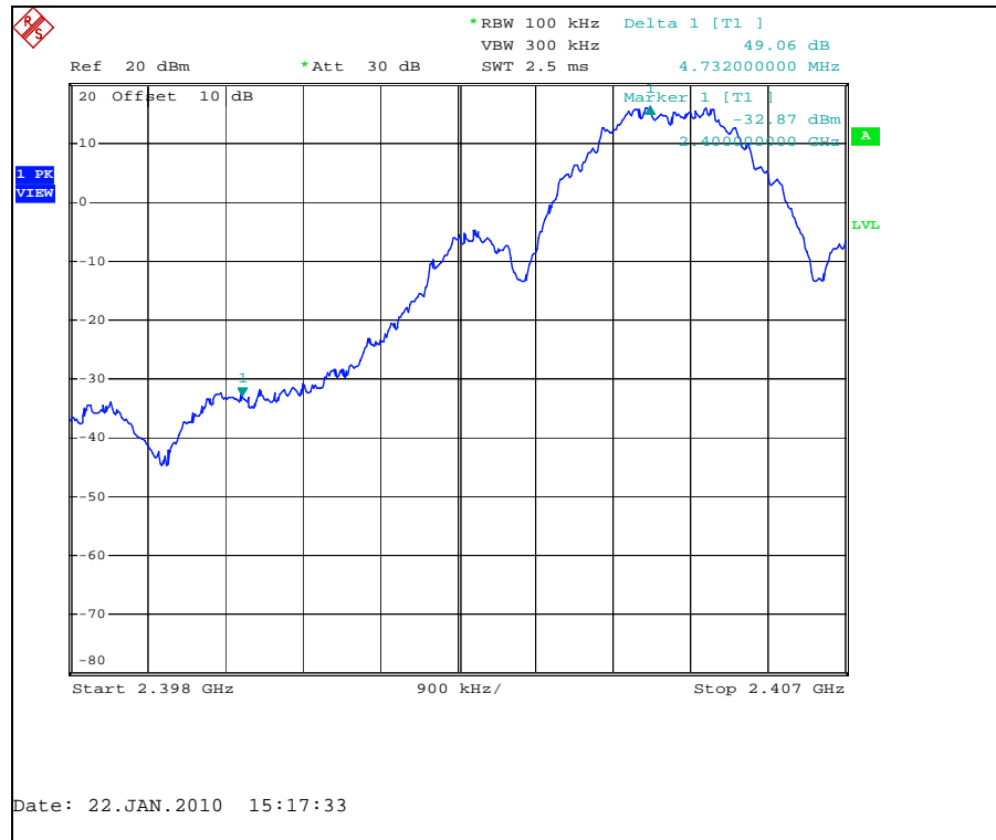
Figure 7.6.1.2-3: Lower Band-edge (Conducted)
