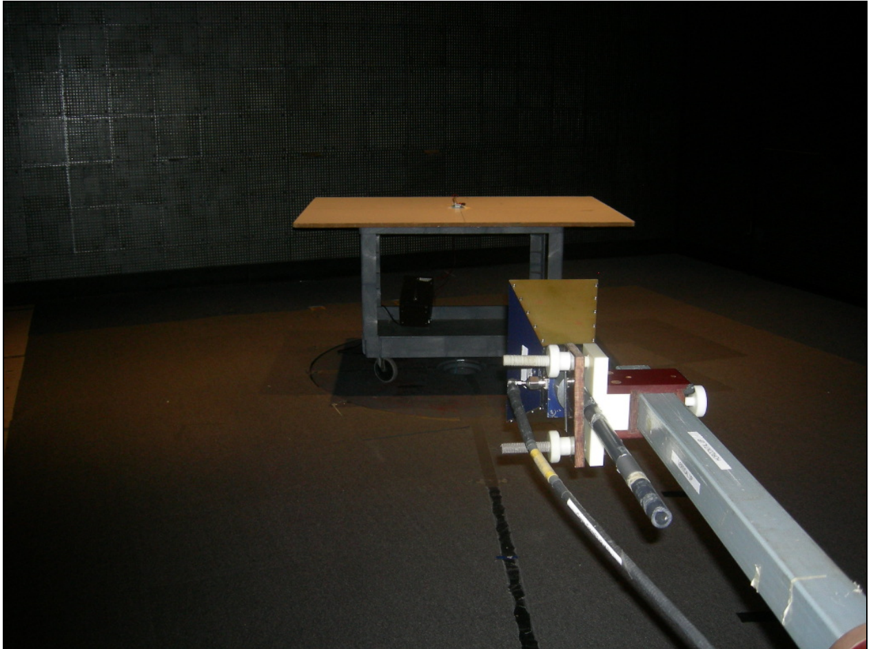
Figure 3: Radiated Emissions
