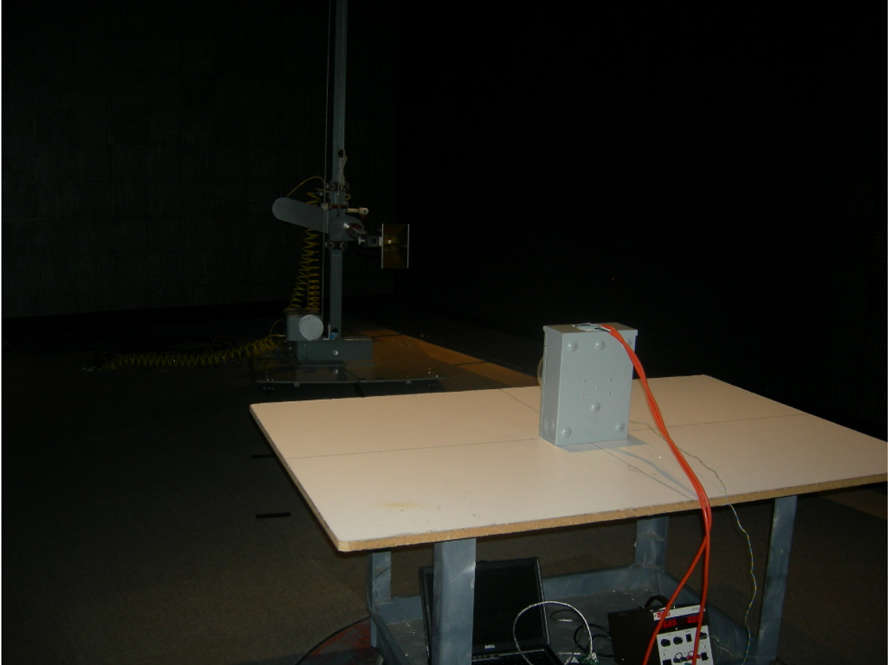
Figure 5: Radiated Emissions (Collocated with FCC ID: SDBIDTB002, IC: 2220A-IDTB002)
