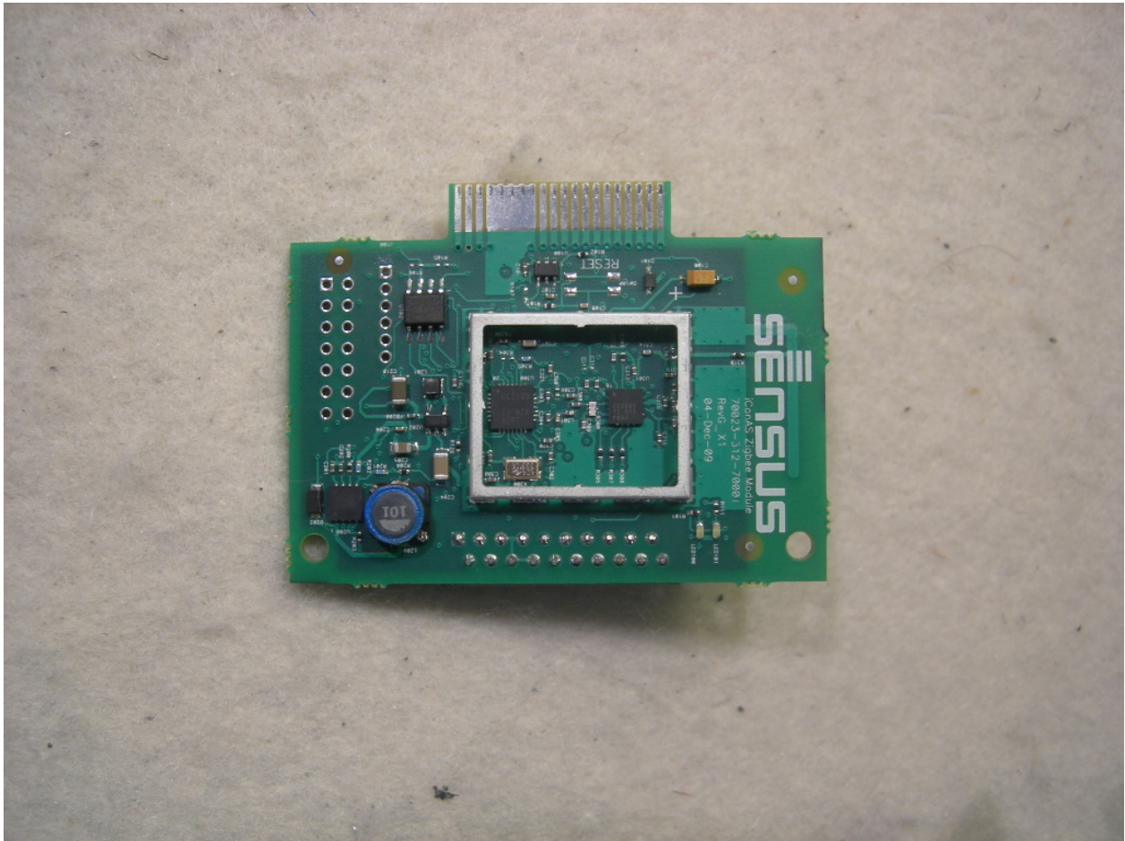
Figure 2: Front View – No Shields
