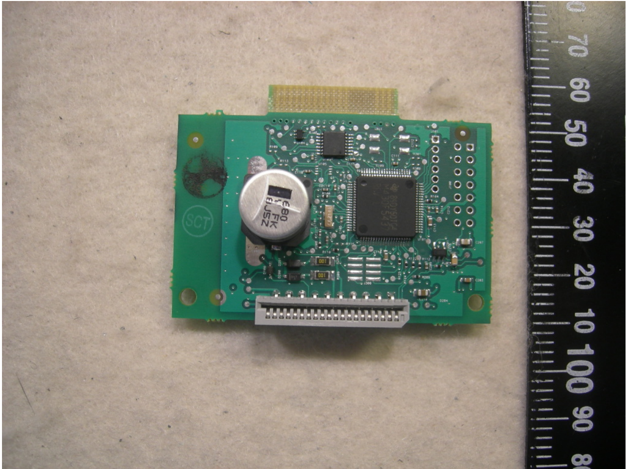
Figure 3: Back View
