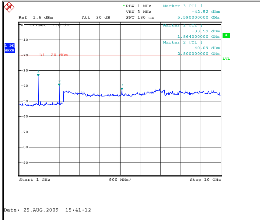
Figure 7.3.2-12: 932.25 MHz – 1GHz to 10GHz
