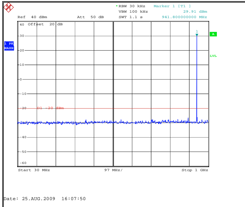
Figure 7.3.2-13: 941.4875 MHz – 30MHz to 1GHz
