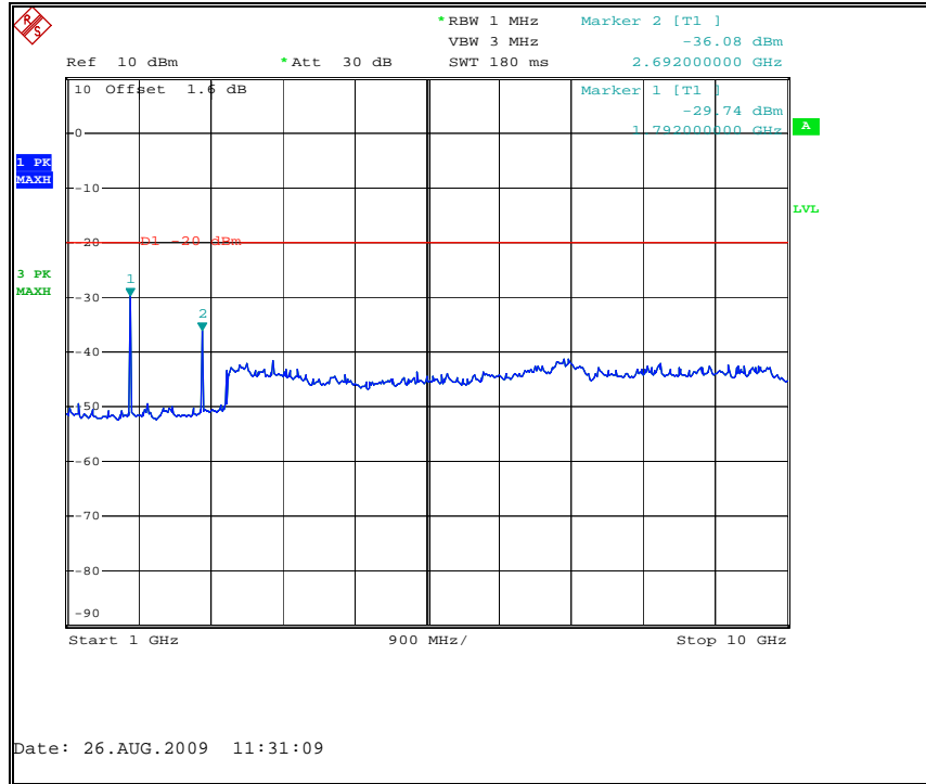
Figure 7.3.2-6: 896.0125 MHz – 1GHz to 10GHz
