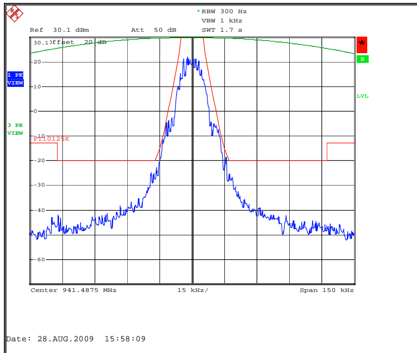
Figure 7.2.2-33: MPass Mode (12.5k) – 941.4875 MHz
