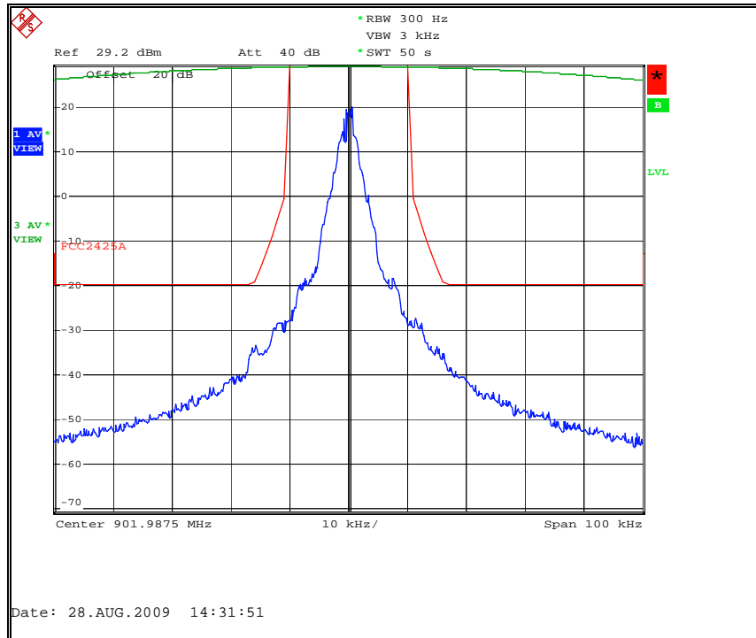
Figure 7.2.2-5: Priority Mode – 901.9875 MHz – 25 kHz Channel
