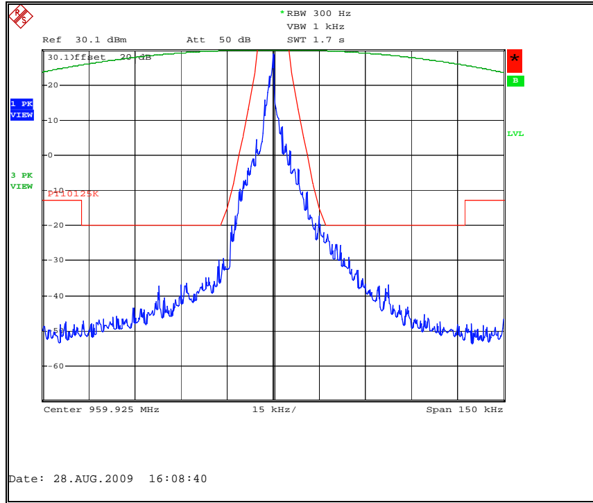
Figure 7.2.2-38: Amplitude Shift Keying Mode (ASK)– 959.925 MHz
