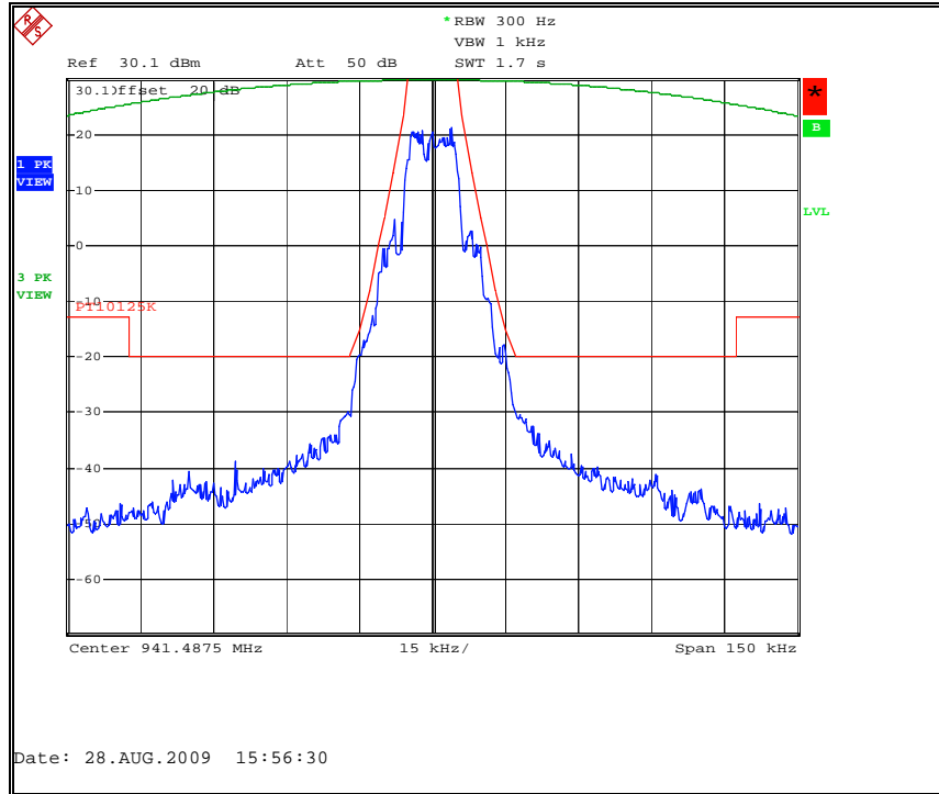
Figure 7.2.2-32: MPass Mode (10k) – 941.4875 MHz
