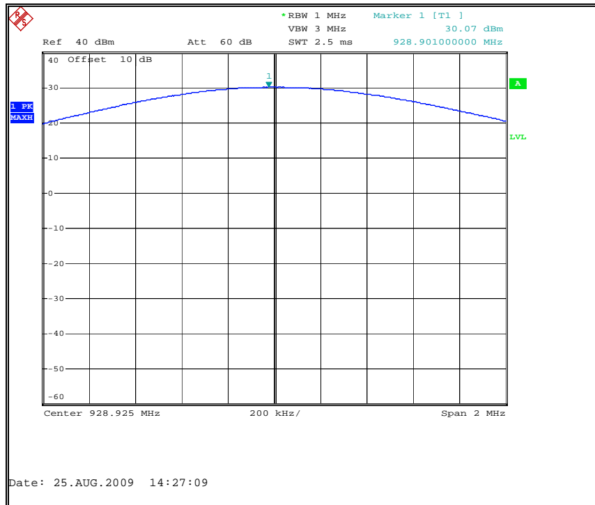
Figure 7.1.2-5: Peak Output Power 928.925 MHz
