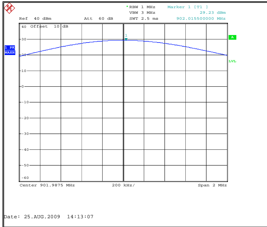
Figure 7.1.2-1: Peak Output Power 901.9875 MHz
