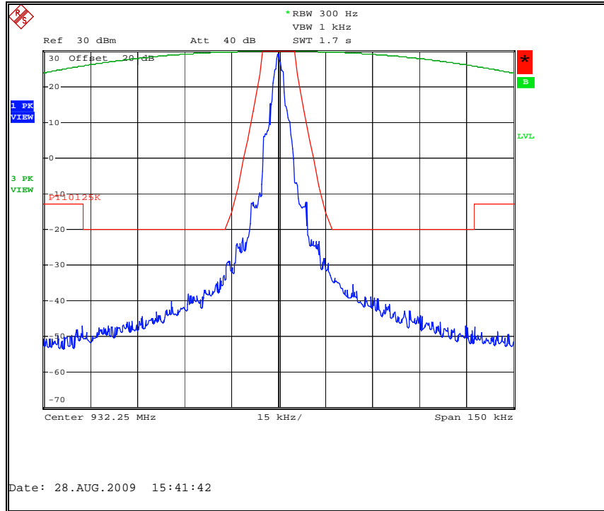
Figure 7.2.2-30: Priority Mode – 932.25 MHz
