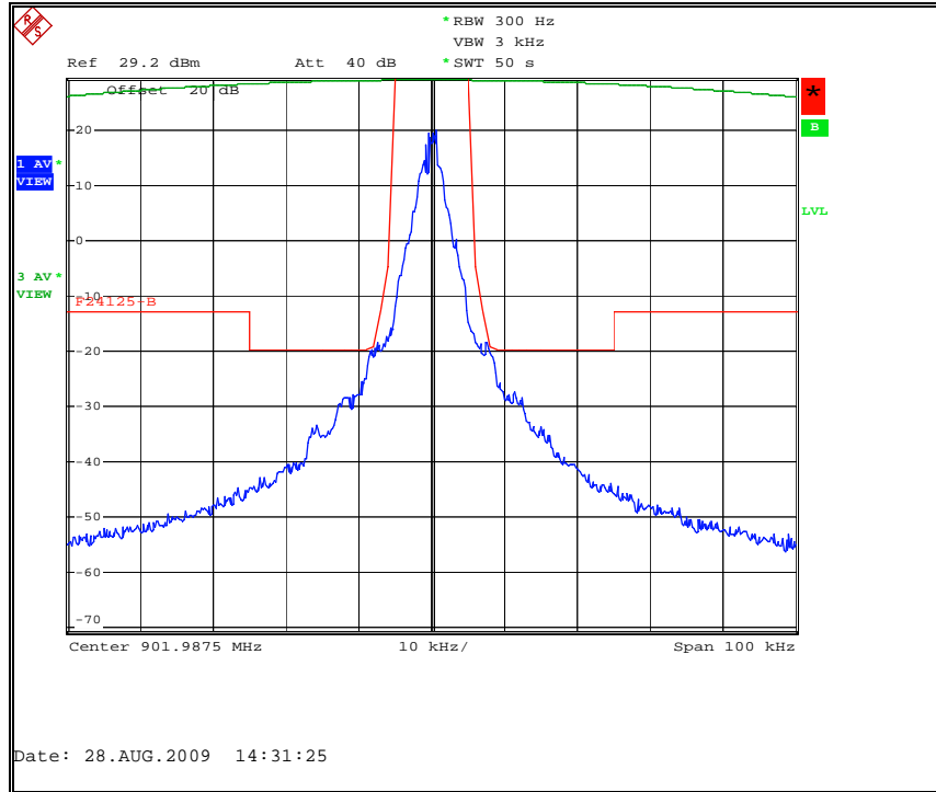
Figure 7.2.2-8: Priority Mode – 901.9875 MHz – 12.5 kHz Channel
