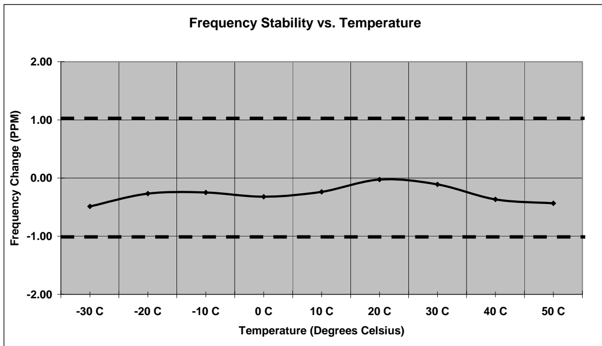
Figure 7.5.2-2: Frequency Stability – 896.01875MHz
