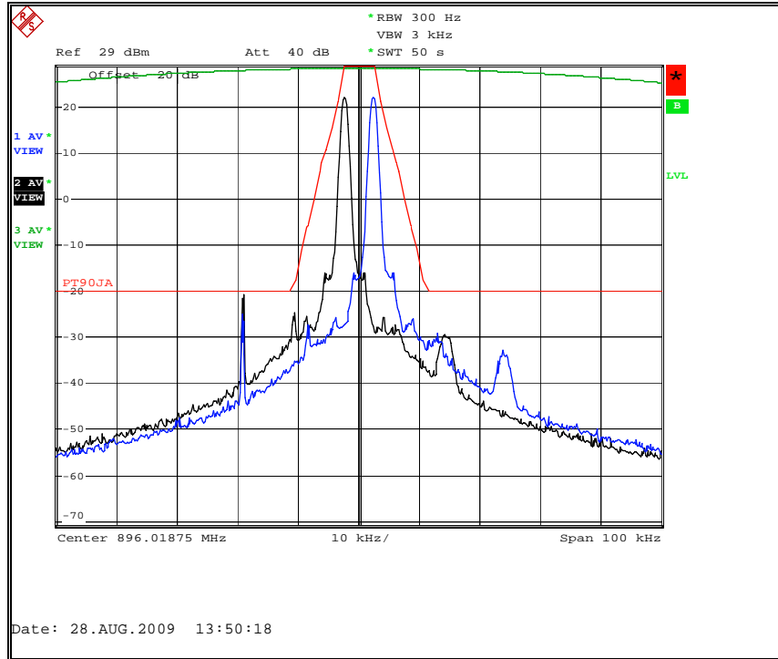
Figure 7.2.2-16: Boost Mode – 896.01875 MHz Offset Channel of +/- 4 (+/- 2400 Hz)
