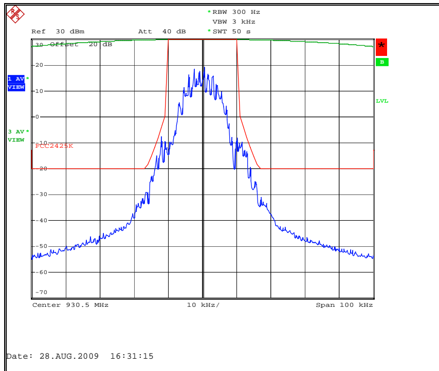
Figure 7.2.2-11: MPass Mode (12.5k) – 930.5 MHz – 25 kHz Channel
