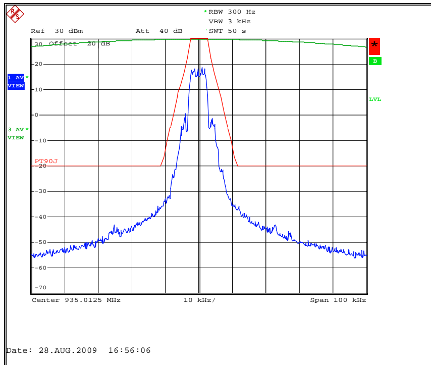
Figure 7.2.2-19: MPass Mode (5k) – 935.0125 MHz
