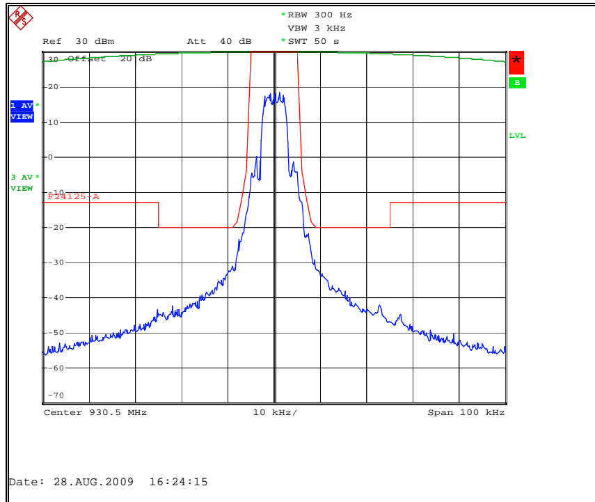
Figure 7.2.2-13: MPass Mode (5K)– 930.5 MHz – 12.5 kHz Channel
