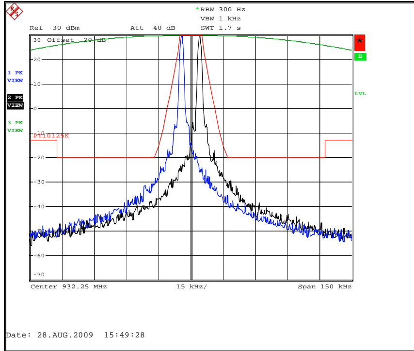
Figure 7.2.2-28: Boost Mode – 932.25 MHz Offset Channel of +/- 7 (+/- 4200 Hz)
