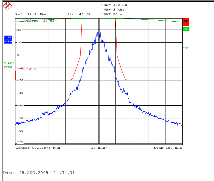
Figure 7.2.2-4: Double Density Mode – 901.9875 MHz – 25 kHz Channel
