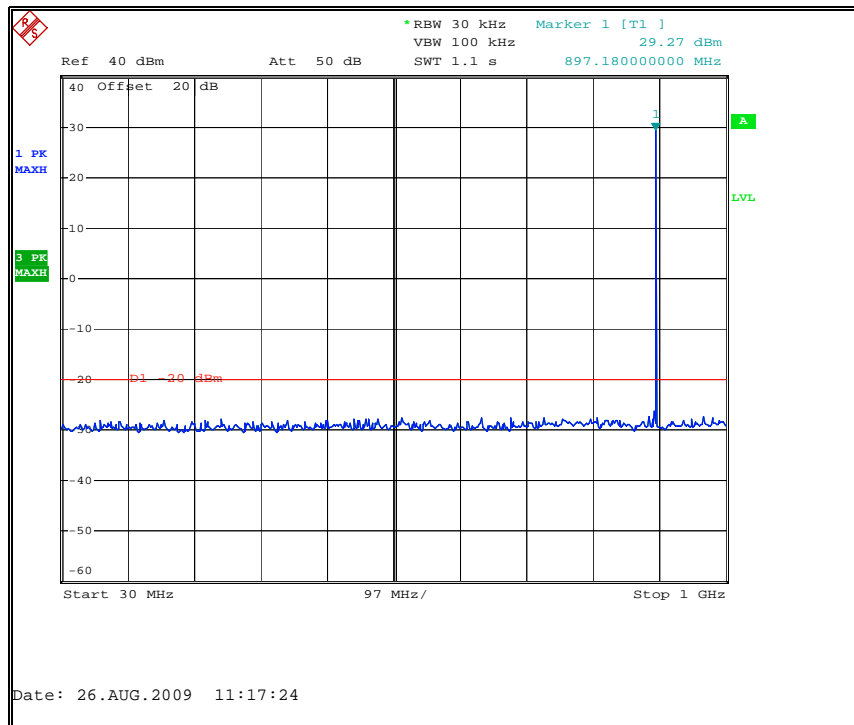
Figure 7.3.2-5: 896.0125 MHz – 30MHz to 1GHz
