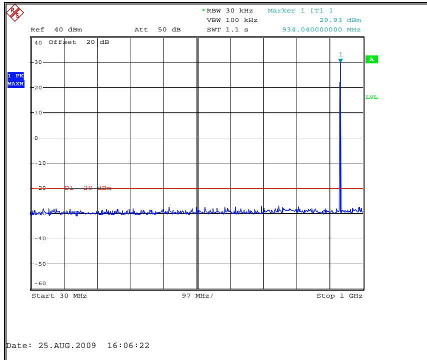
Figure 7.3.2-11: 932.25 MHz – 30MHz to 1GHz
