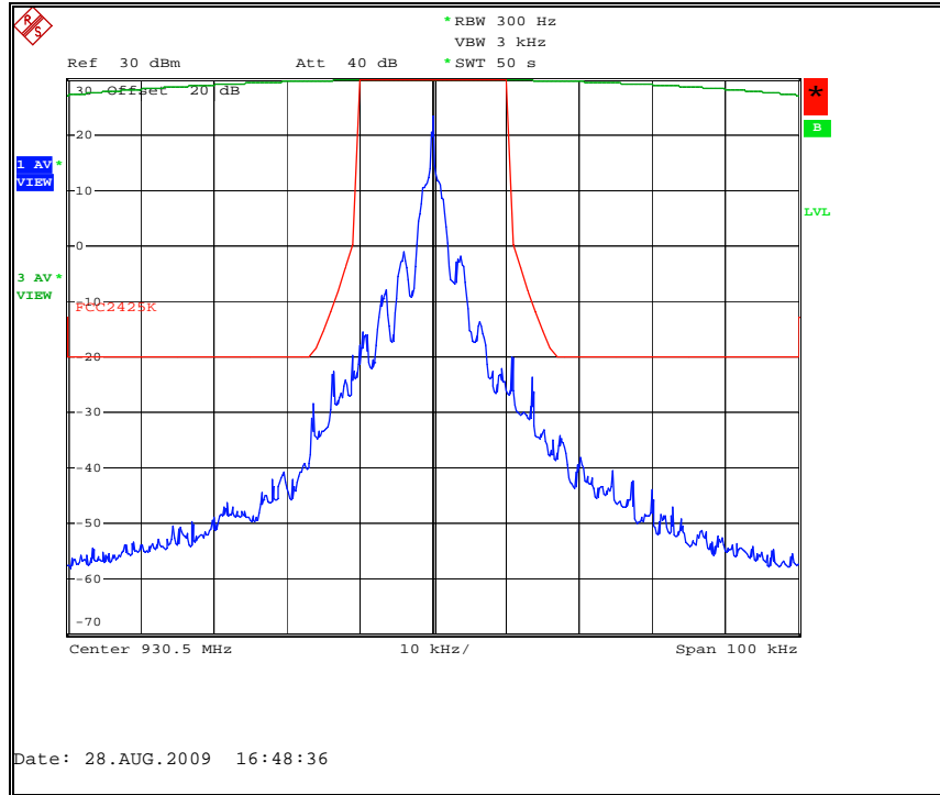
Figure 7.2.2-12: Amplitude Shift Keying Mode (ASK) – 930.5 MHz
