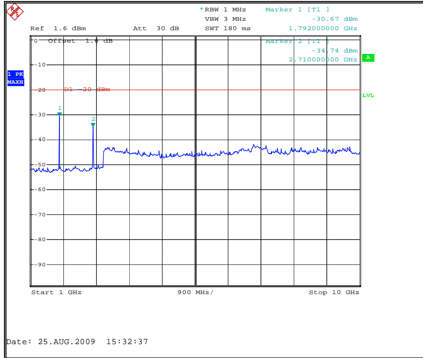
Figure 7.3.2-2: 901.9875 MHz – 1GHz to 10GHz
