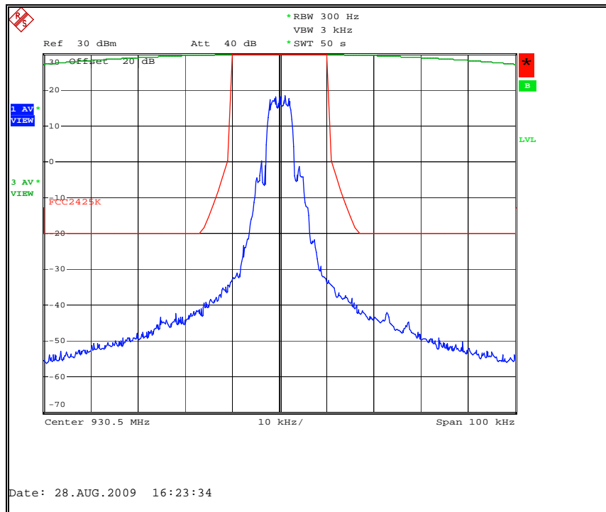
Figure 7.2.2-9: MPass Mode (5k) – 930.5 MHz – 25 kHz Channel
