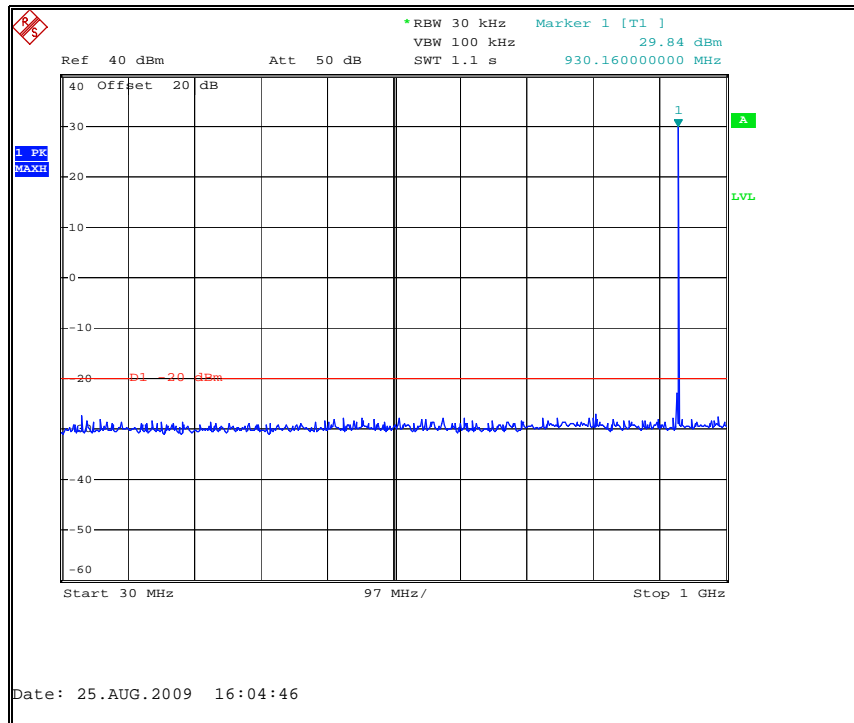
Figure 7.3.2-9: 928.925 MHz – 30MHz to 1GHz
