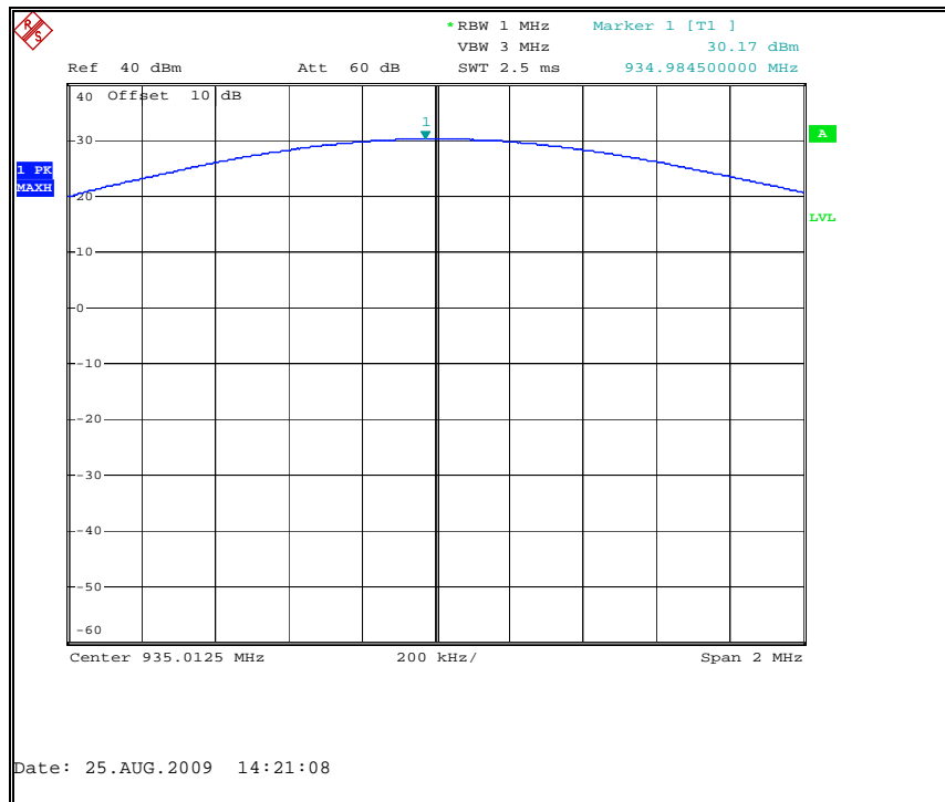
Figure 7.1.2-4: Peak Output Power 935.0125 MHz
