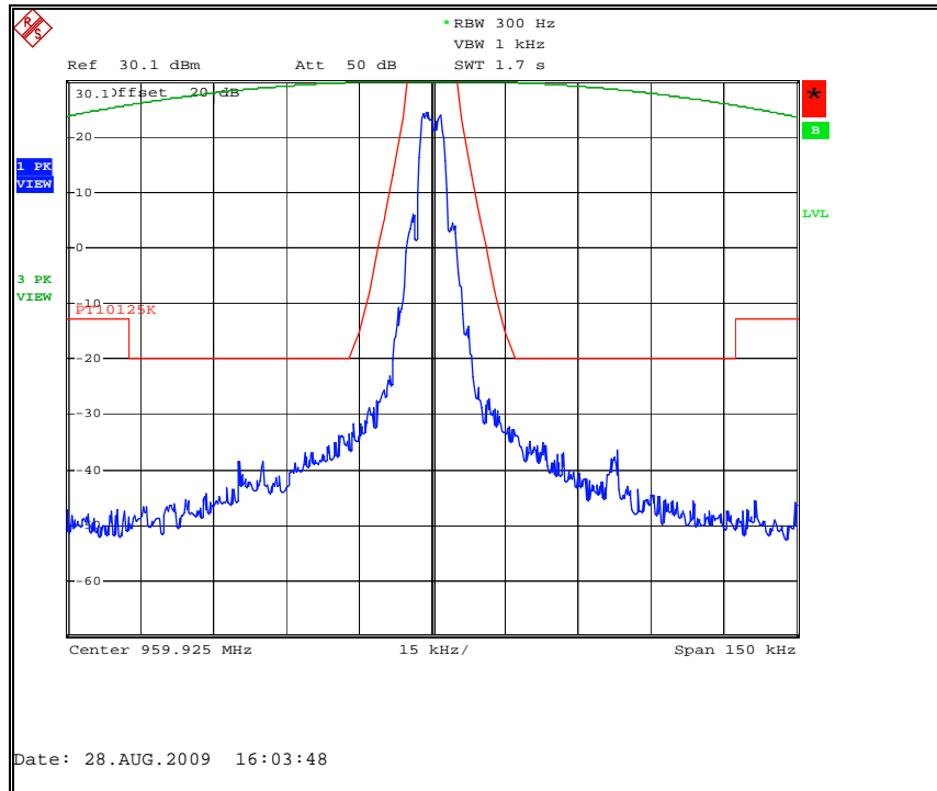
Figure 7.2.2-35: MPass Mode (5k) – 959.925 MHz
