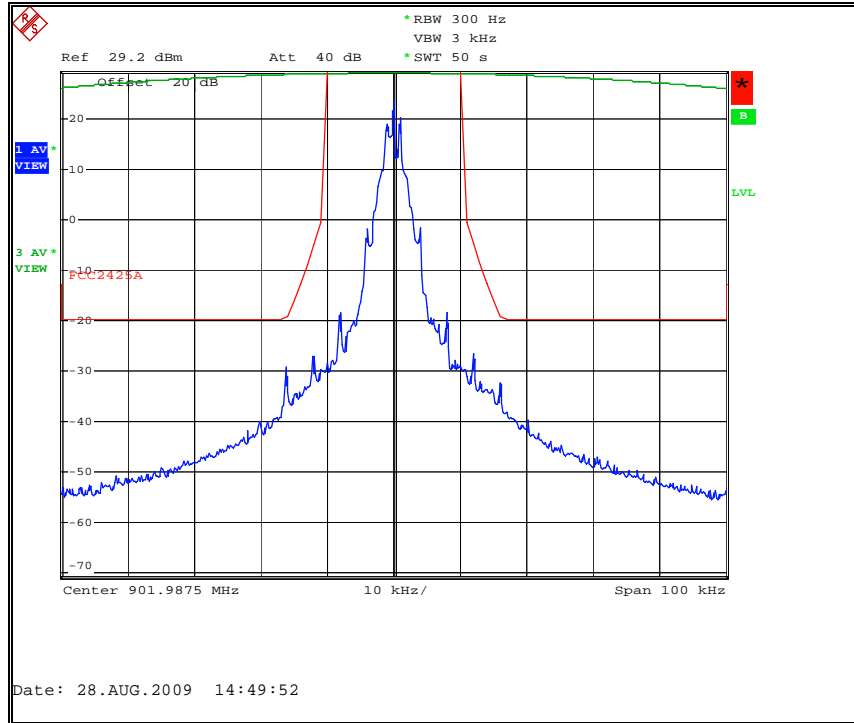
Figure 7.2.2-2: C&I Mode – 901.9875 MHz – 25 kHz Channel
