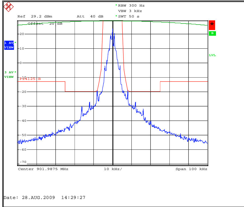
Figure 7.2.2-6: C&I Mode – 901.9875 MHz – 12.5 kHz Channel
