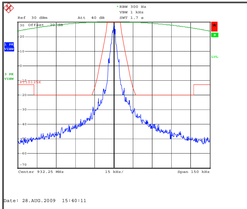
Figure 7.2.2-27: C&I Mode – 932.25 MHz
