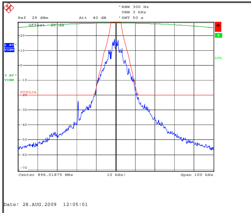
Figure 7.2.2-17: Double Density Mode – 896.01875 MHz
