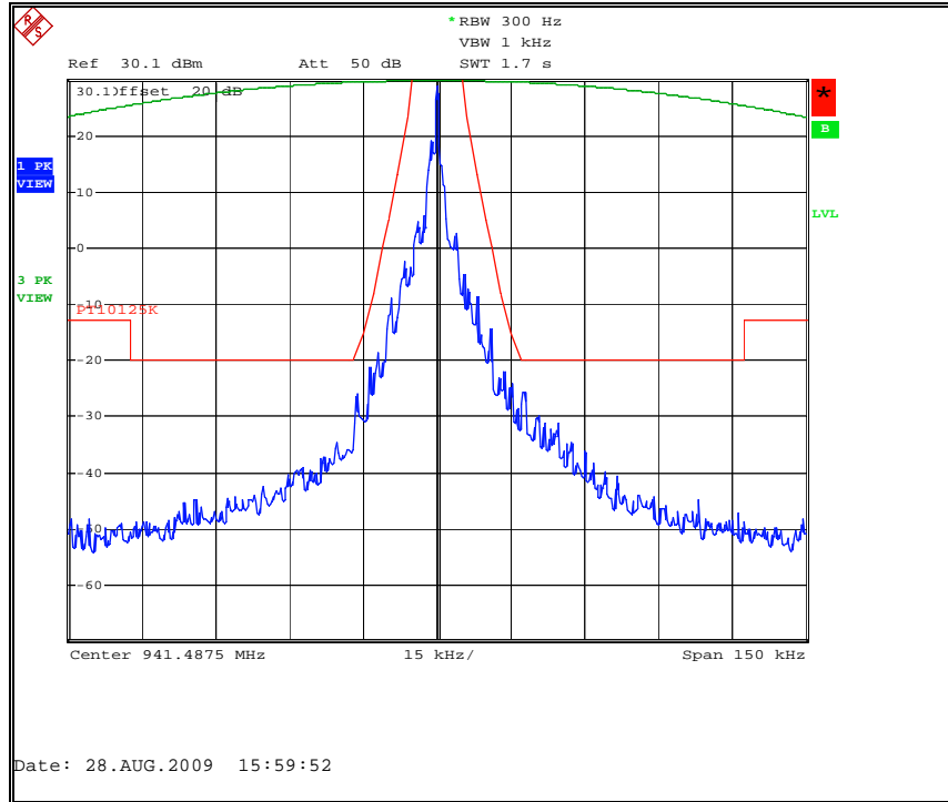
Figure 7.2.2-34: Amplitude Shift Keying Mode (ASK)– 941.4875 MHz
