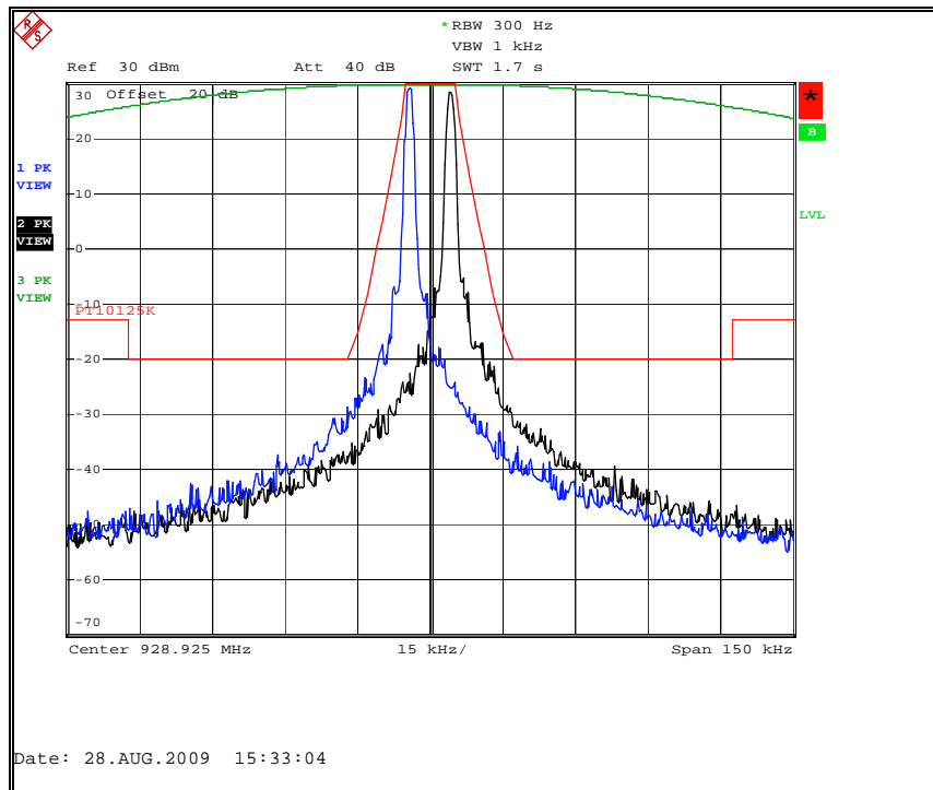
Figure 7.2.2-23: Boost Mode – 928.925 MHz Offset Channel of +/- 7 (+/- 4200 Hz)
