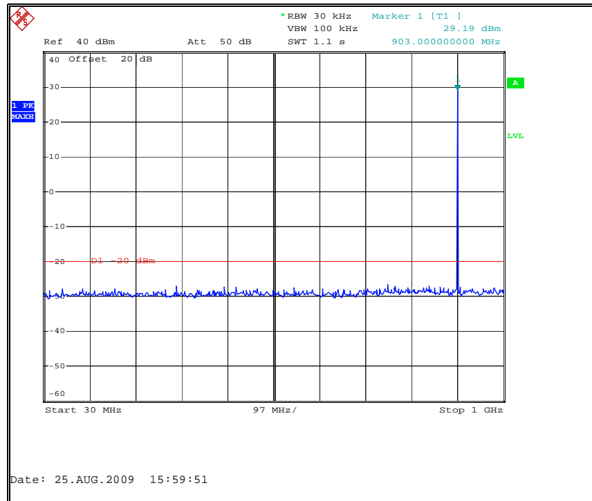
Figure 7.3.2-1: 901.9875 MHz – 30MHz to 1GHz
