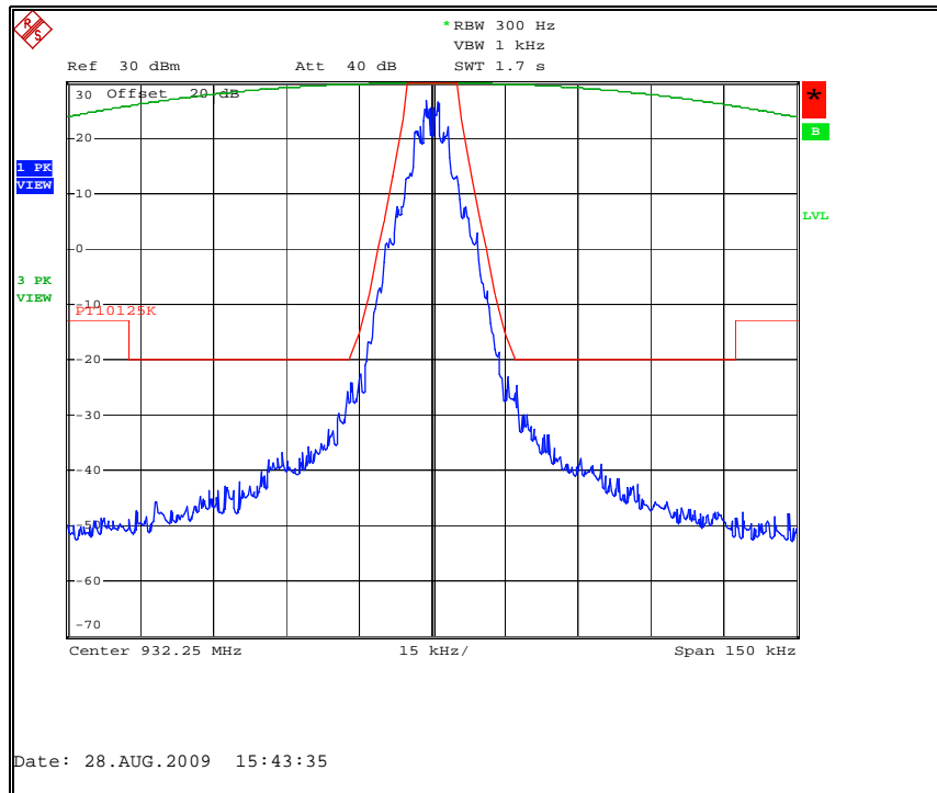
Figure 7.2.2-29: Double Density Mode – 932.25 MHz
