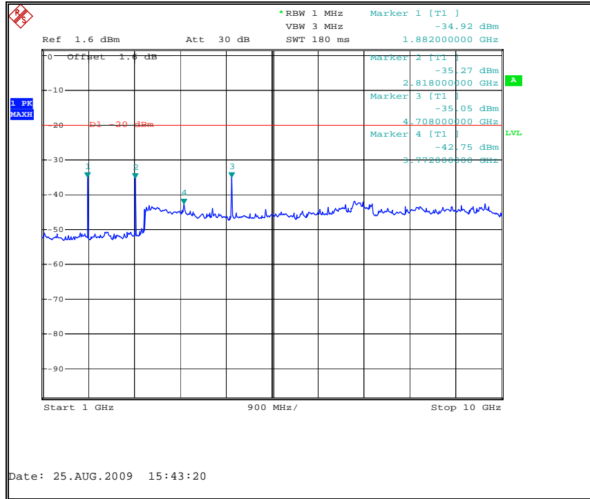
Figure 7.3.2-14: 941.4875 MHz – 1GHz to 10GHz
