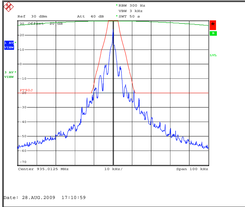
Figure 7.2.2-20: Amplitude Shift Keying Mode (ASK)– 935.0125 MHz
