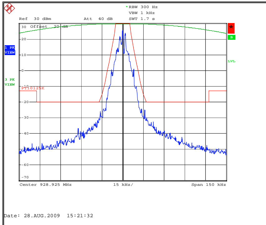
Figure 7.2.2-21: Normal Mode – 928.925 MHz
