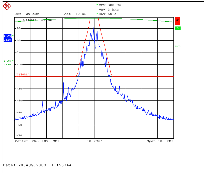
Figure 7.2.2-14: Normal Mode – 896.01875 MHz
