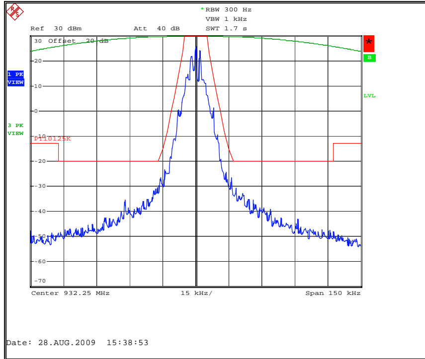
Figure 7.2.2-26: Normal Mode – 932.25 MHz
