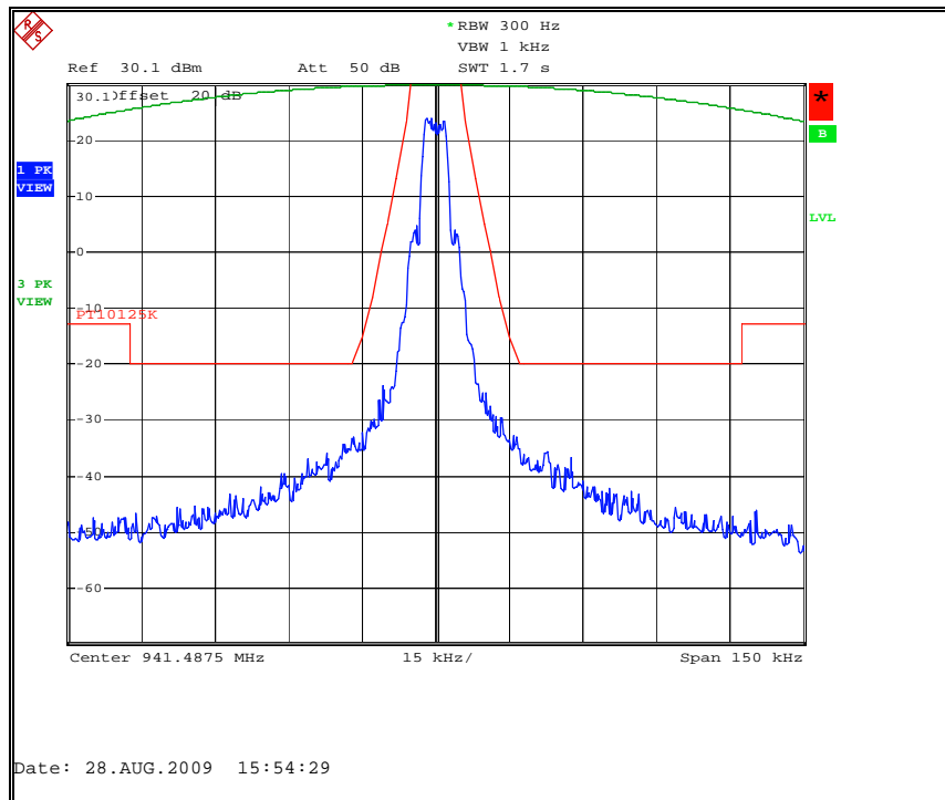
Figure 7.2.2-31: MPass Mode (5k) – 941.4875 MHz
