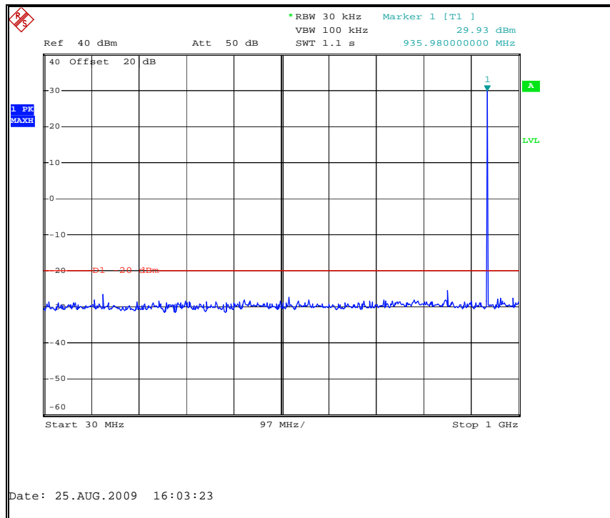
Figure 7.3.2-7: 935.0125 MHz – 30MHz to 1GHz
