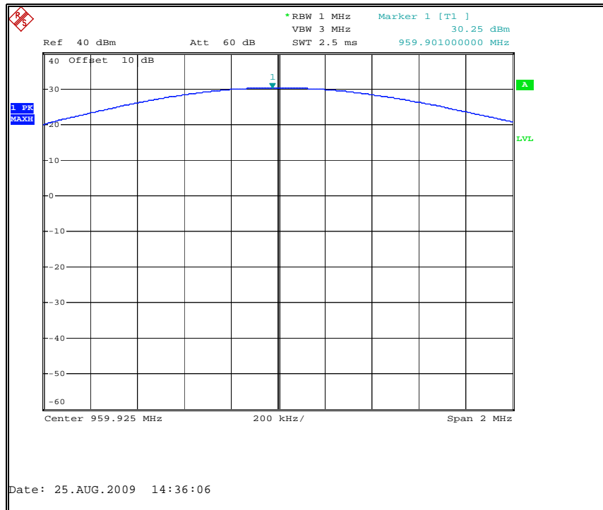
Figure 7.1.2-8: Peak Output Power 959.925 MHz
