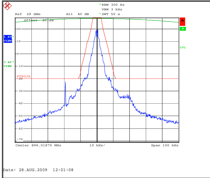
Figure 7.2.2-18: Priority Mode – 896.01875 MHz
