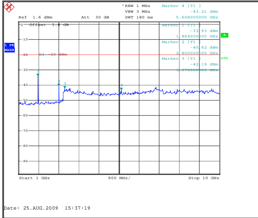
Figure 7.3.2-8: 935.0125 MHz – 1GHz to 10GHz
