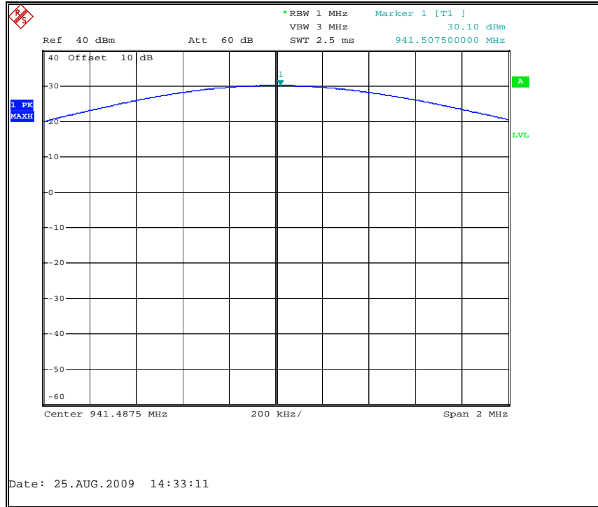
Figure 7.1.2-7: Peak Output Power 941.4875 MHz
