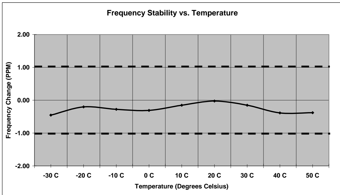
Figure 7.5.2-3: Frequency Stability – 959.9250MHz
