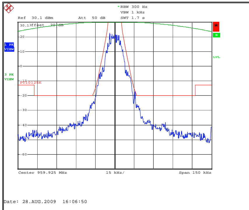
Figure 7.2.2-37: MPass Mode (12.5k) – 959.925 MHz
