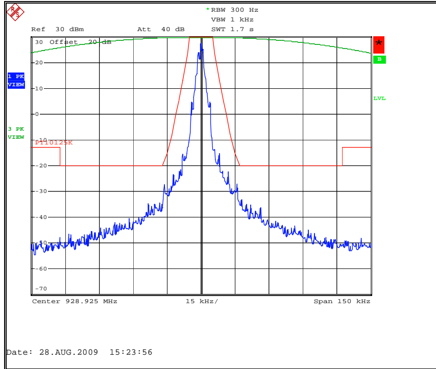
Figure 7.2.2-22: C&I Mode – 928.925 MHz
