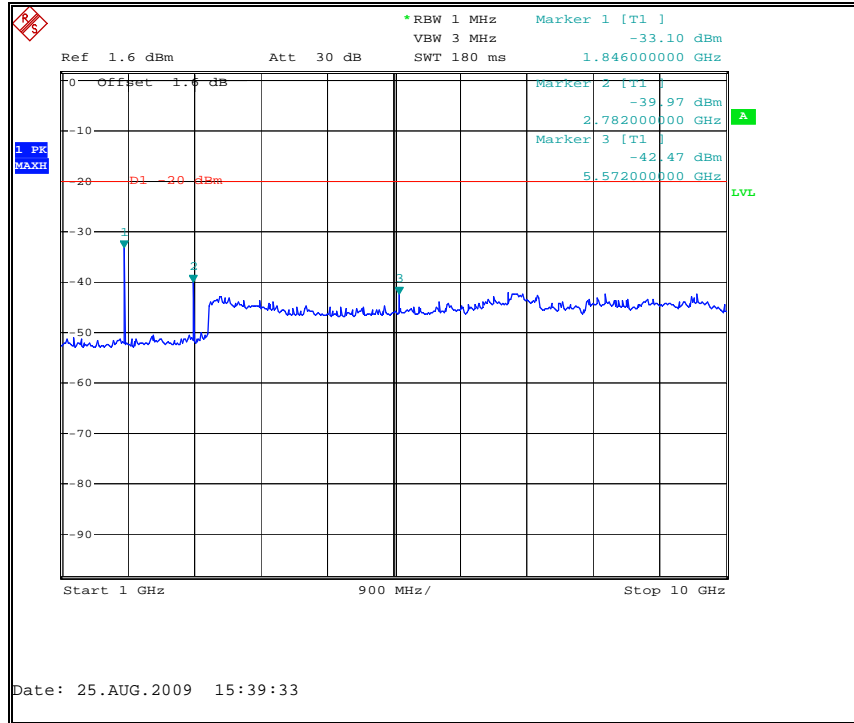
Figure 7.3.2-10: 928.925 MHz – 1GHz to 10GHz
