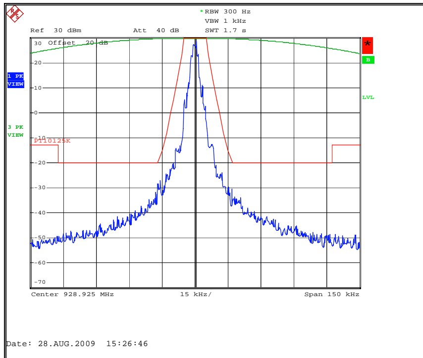
Figure 7.2.2-25: Priority Mode – 928.925 MHz
