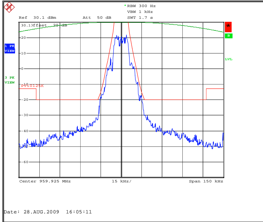
Figure 7.2.2-36: MPass Mode (10k) – 959.925 MHz
