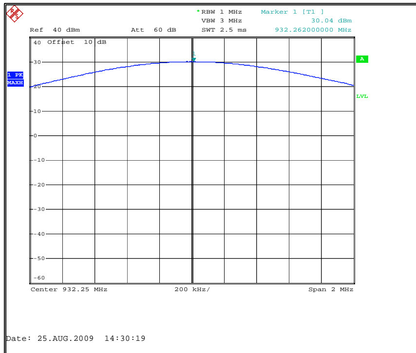
Figure 7.1.2-6: Peak Output Power 932.25 MHz
