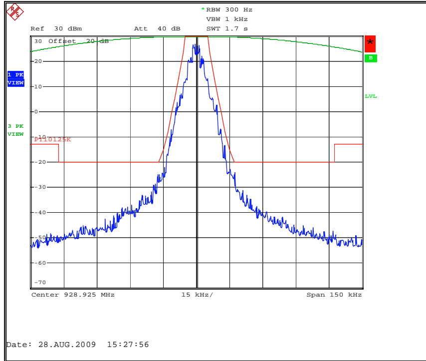
Figure 7.2.2-24: Double Density Mode – 928.925 MHz
