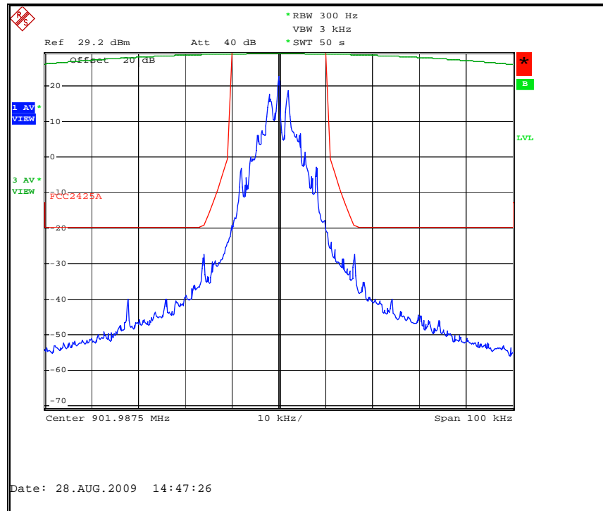
Figure 7.2.2-1: Normal Mode – 901.9875 MHz – 25 kHz Channel
