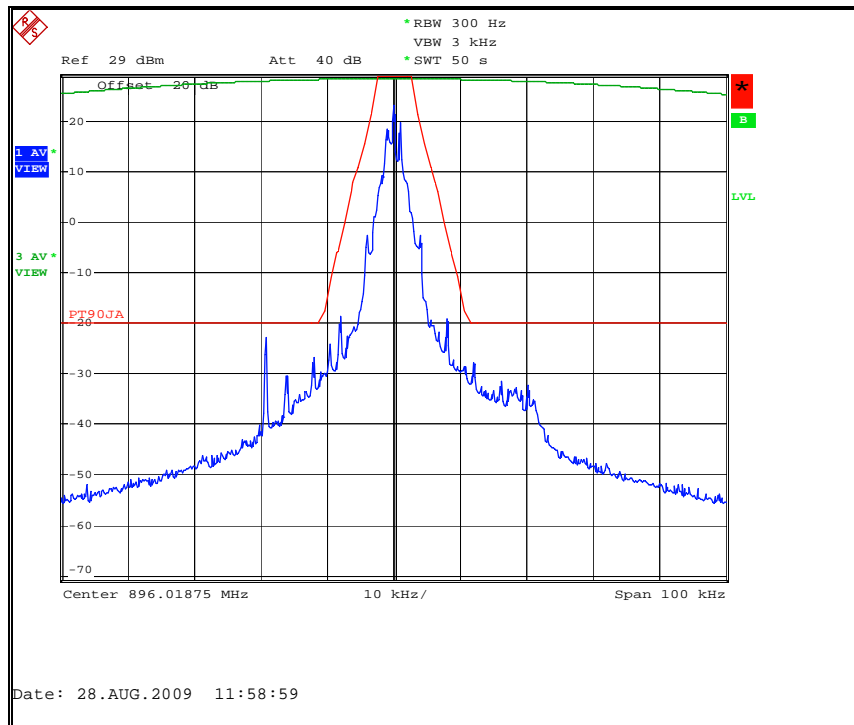
Figure 7.2.2-15: C&I Mode – 896.01875 MHz
