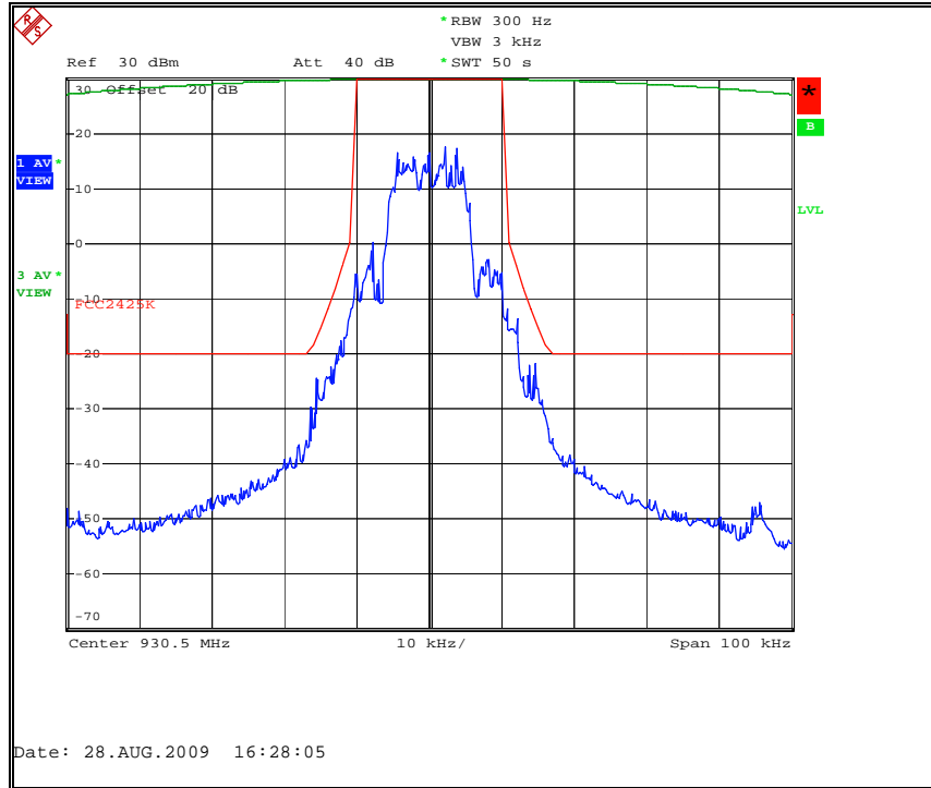
Figure 7.2.2-10: MPass Mode (10k) – 930.5 MHz – 25 kHz Channel
