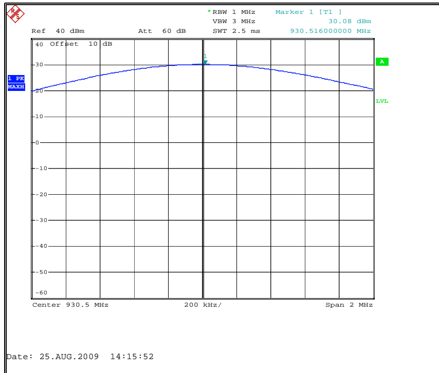
Figure 7.1.2-2: Peak Output Power 930.5 MHz
