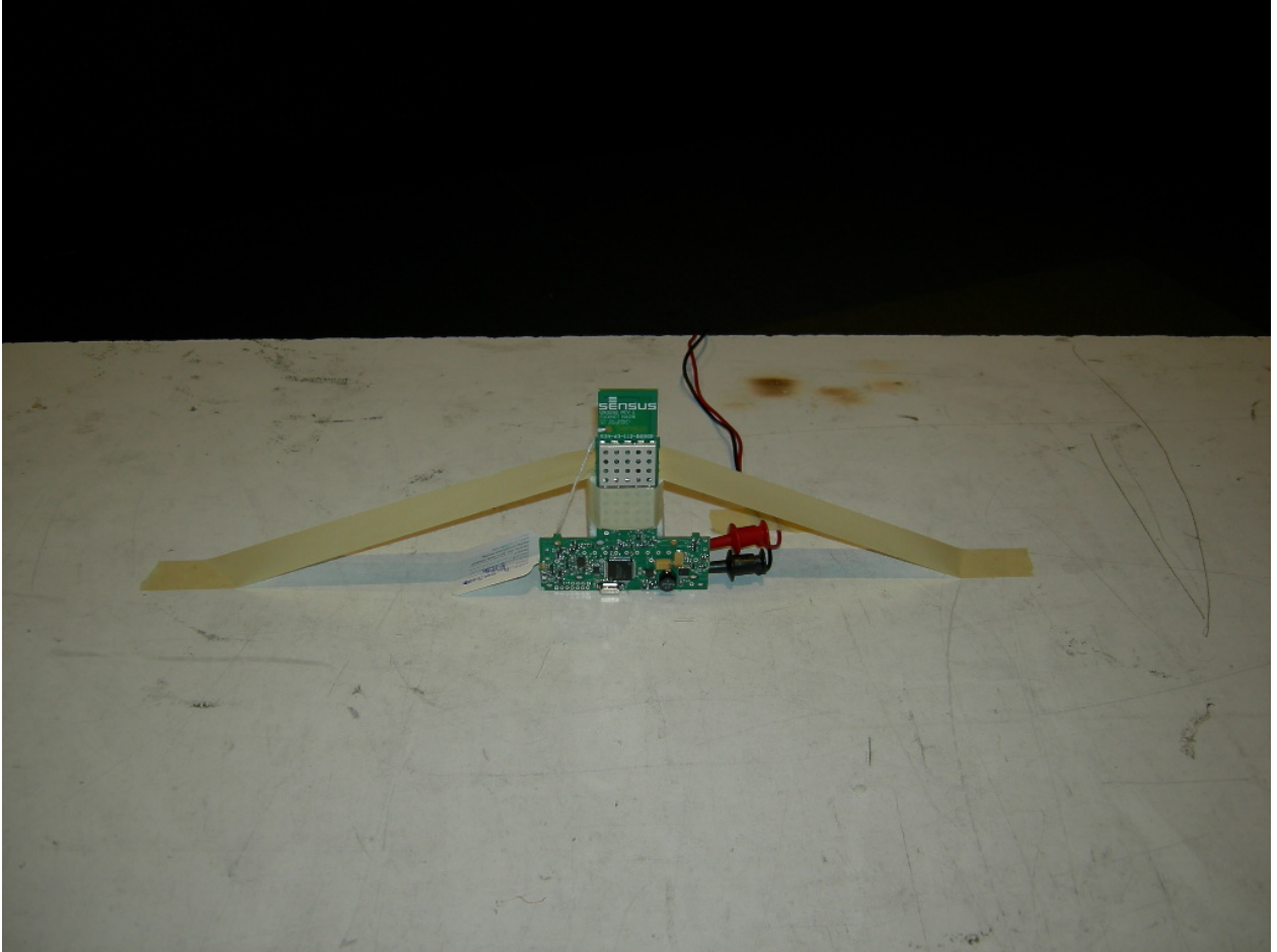
Figure 1: Radiated Emissions (520x "T" Board)
