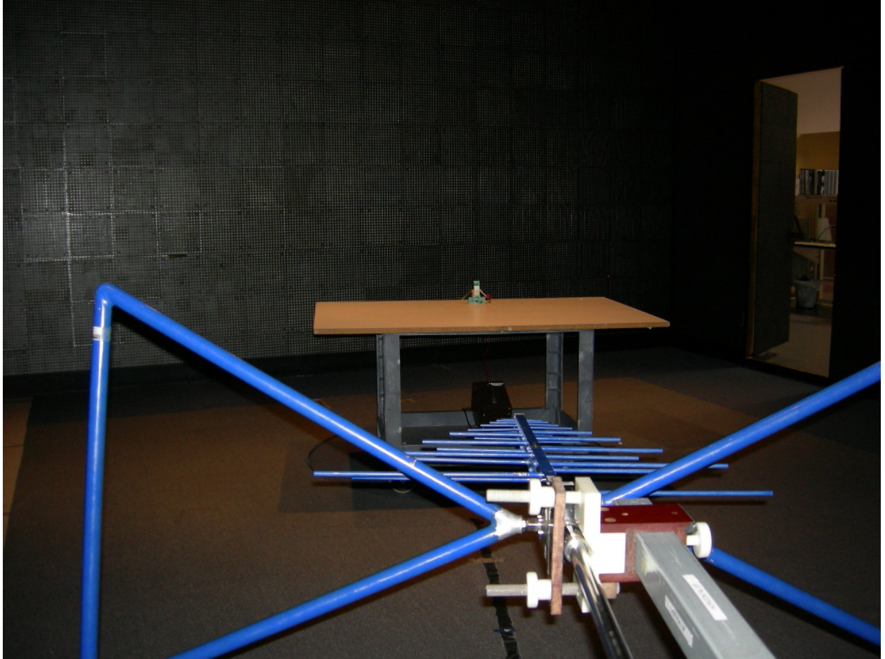
Figure 3: Radiated Emissions (520x "T" Board)
