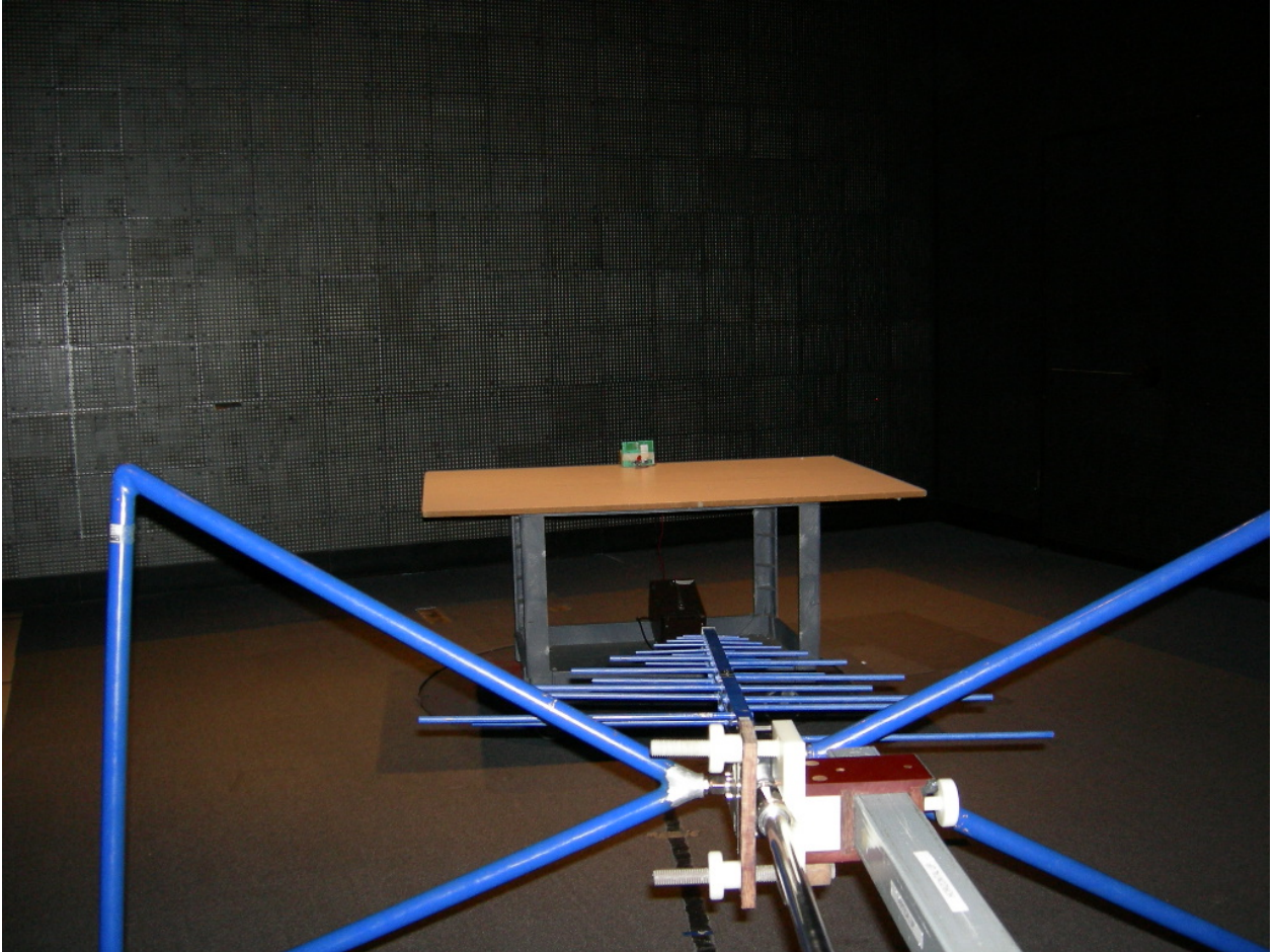
Figure 6: Radiated Emissions (510x SOH Board)
