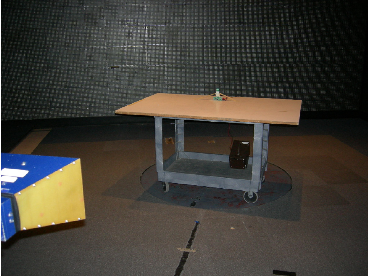
Figure 2: Radiated Emissions (520x "T" Board)
