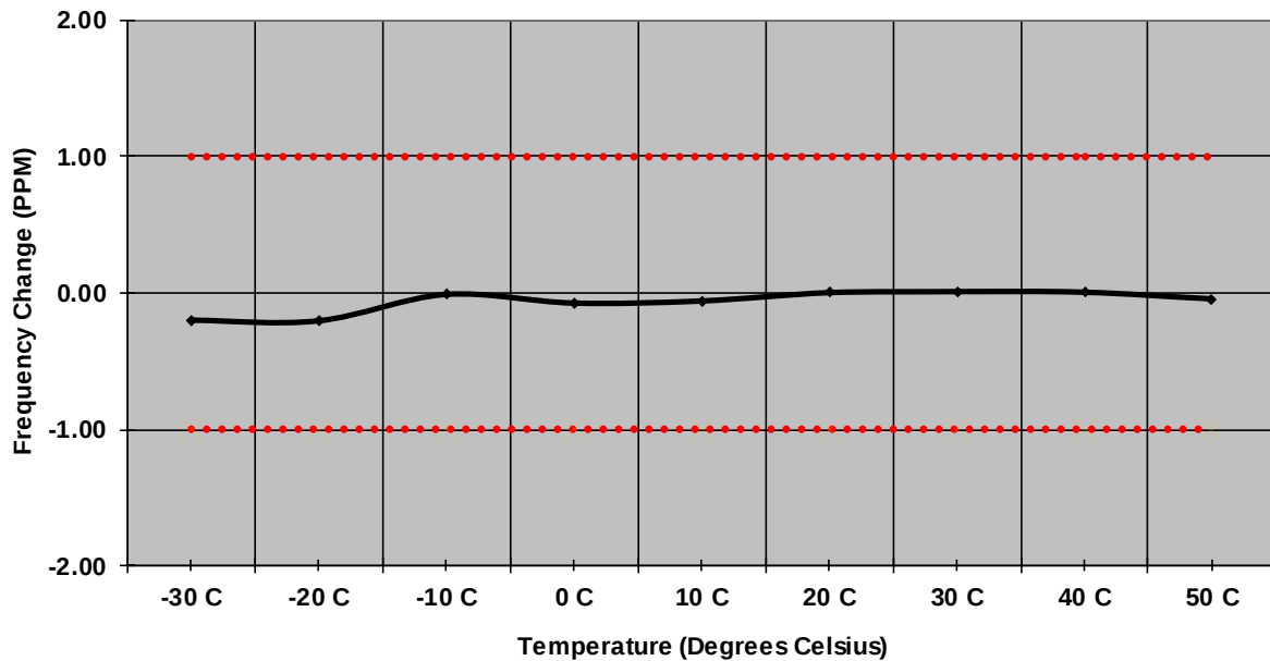
Figure 7.6.2-3: Frequency Stability – 941.25 MHz
