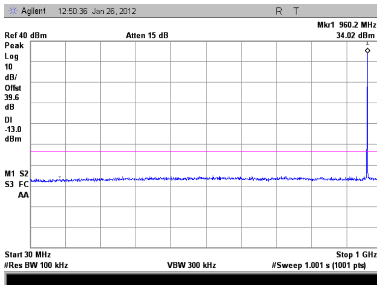
Figure 7.3.2-1: 959.925 MHz – 30MHz to 1GHz
