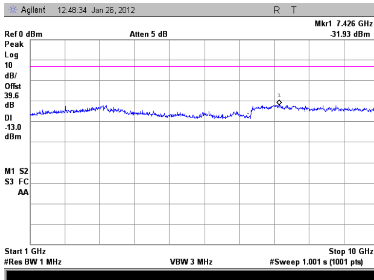
Figure 7.3.2-2: 959.925 MHz – 1GHz to 10GHz
