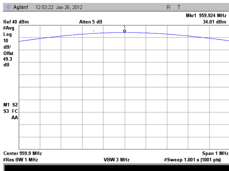
Figure 7.1.2-1: Peak Output Power 959.925 MHz
