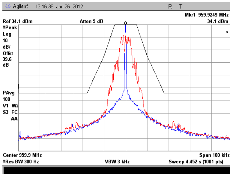
Figure 7.2.2-1: 959.925 MHz – MPass 5k Mode
