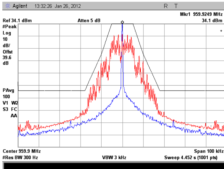
Figure 7.2.2-2: 959.925 MHz – MPass 10k Mode
