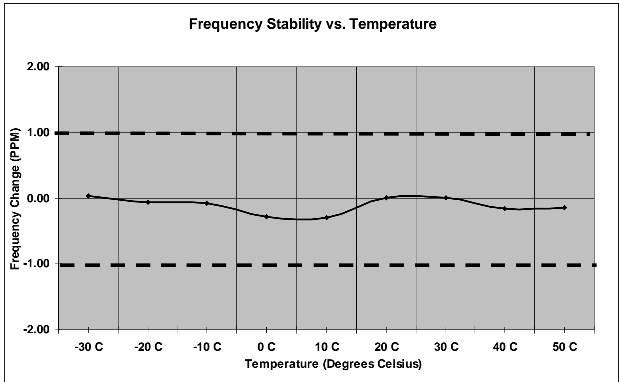
Figure 7.5.2-1: Frequency Stability – 959.925 MHz
