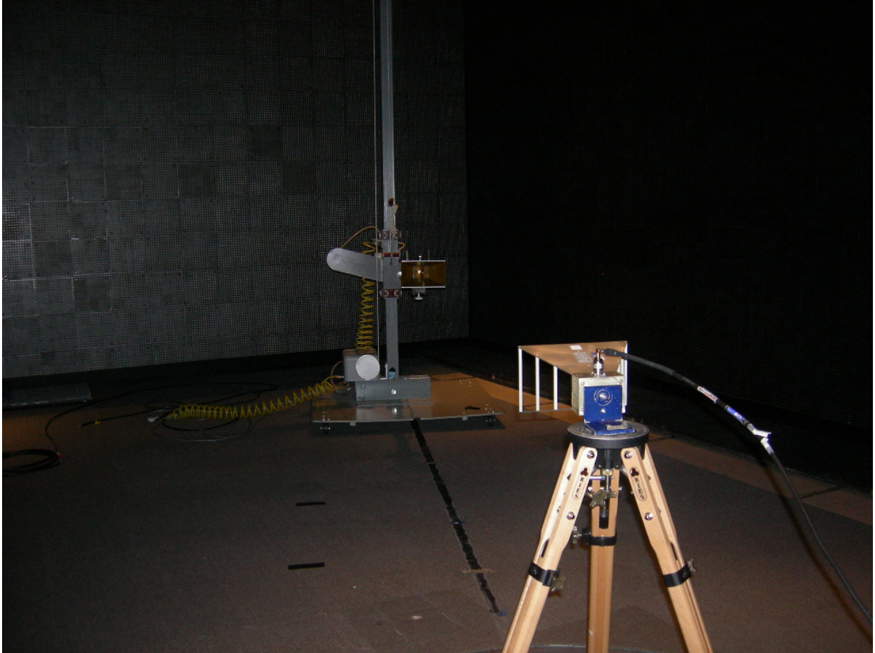
Figure 6: Radiated Emissions - Substitution
