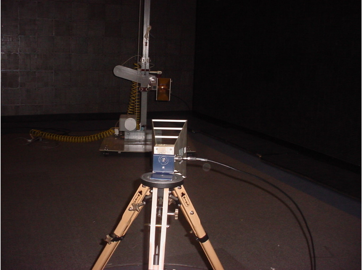
Figure 3: Radiated Emissions (Substitution Method)
