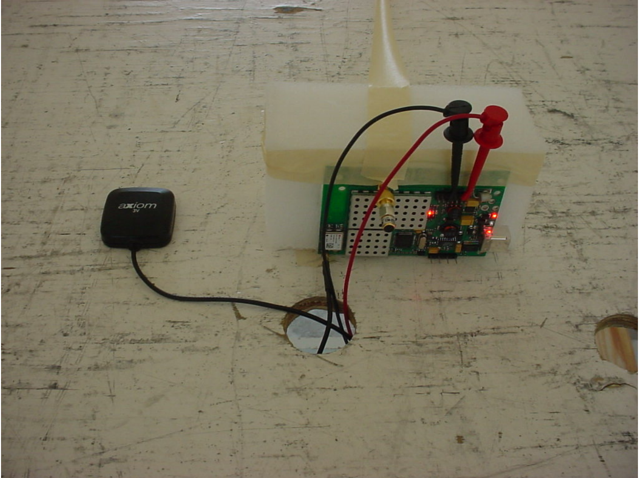
Figure 3: Radiated Emissions – GPS Option
