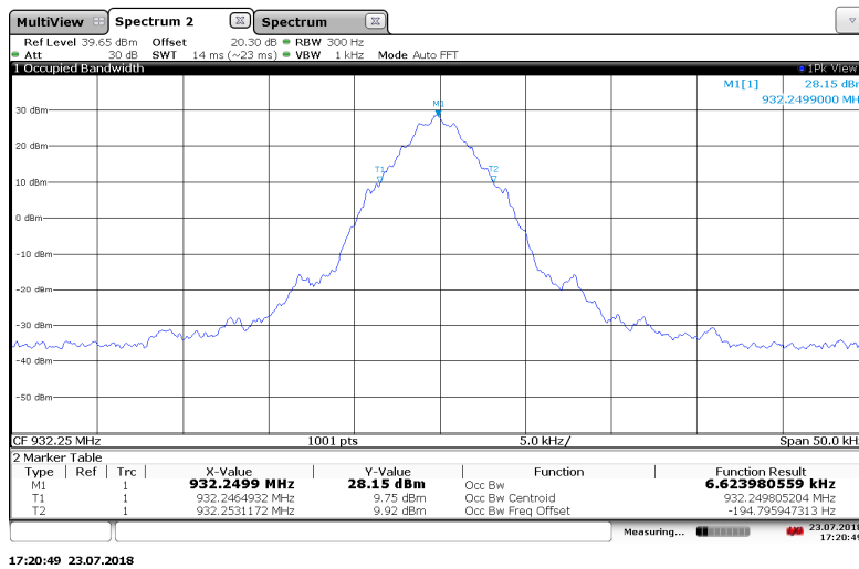
Figure 7.3.2-15: 932.25 MHz – C&I (Half Baud) Mode
