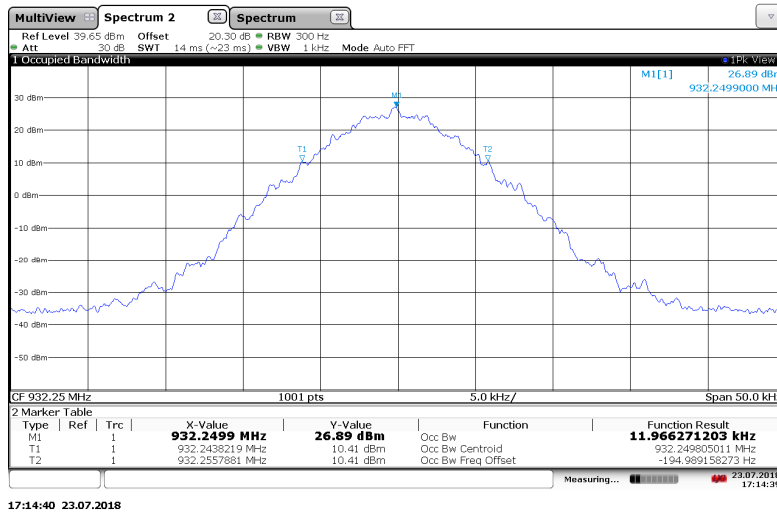
Figure 7.3.2-17: 932.25 MHz – Normal Mode
