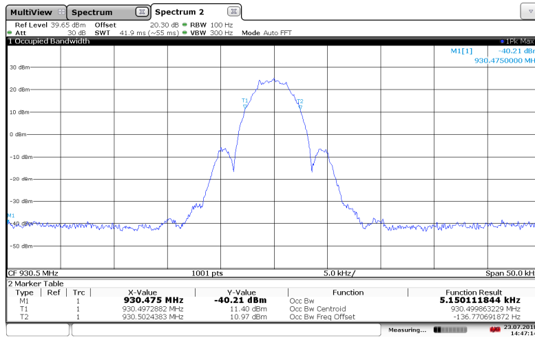
Figure 7.3.2-6: 930.5 MHz – MPass 5k Mode
