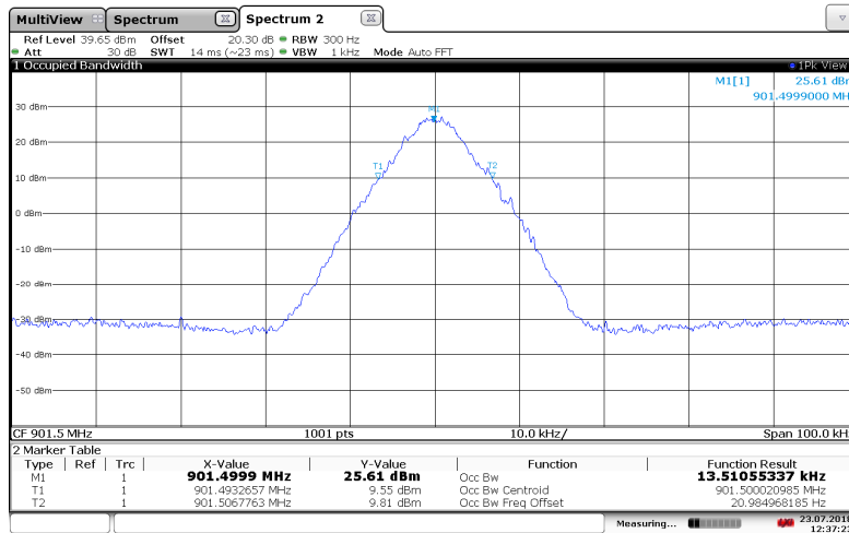
Figure 7.3.2-2: 901.5 MHz – Double Density Mode
