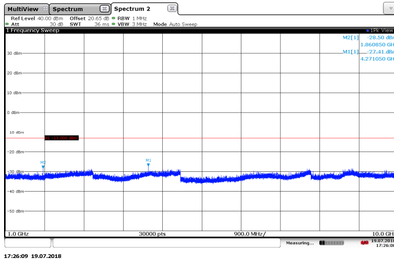
17:26:09 19.07.2018 Figure 7.4.2-4: 930.5 MHz – 1GHz to 10GHz – Mpass 5k mode
