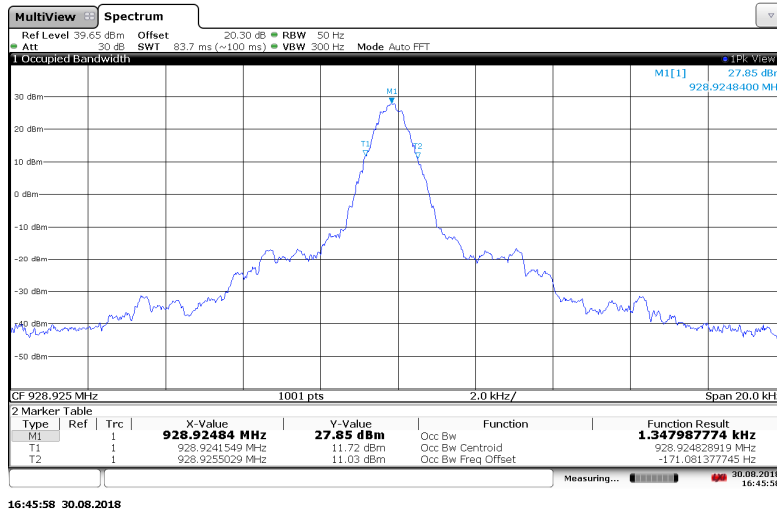
Figure 7.3.2-14: 928.925 MHz – Boost Mode
