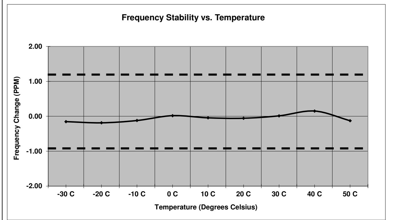
Figure 7.6.2-1: Frequency Stability – 901.5 MHz – KDS
