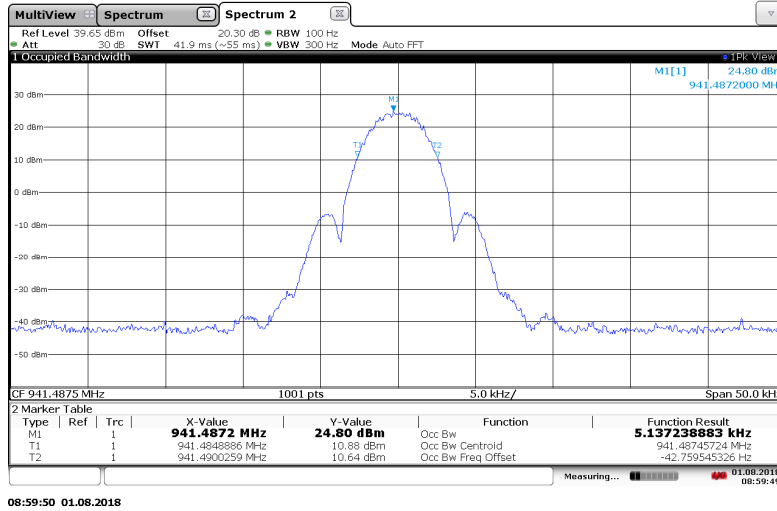
Figure 7.3.2-20: 941.4875 MHz – MPass 5k Mode
