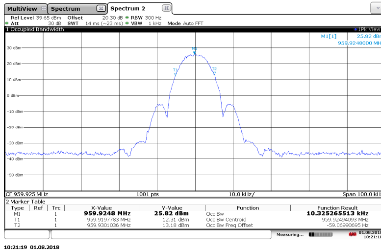
Figure 7.3.2-25: 959.925 MHz– mPass 10k Mode
