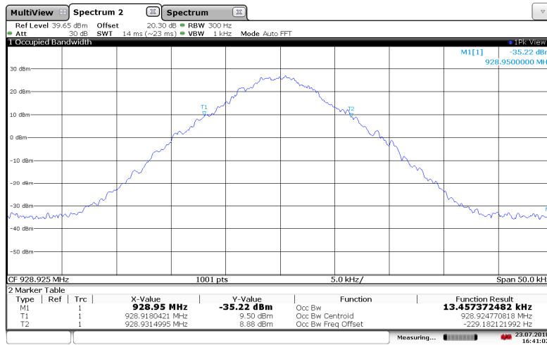
Figure 7.3.2-11: 928.925 MHz – Double Density Mode
