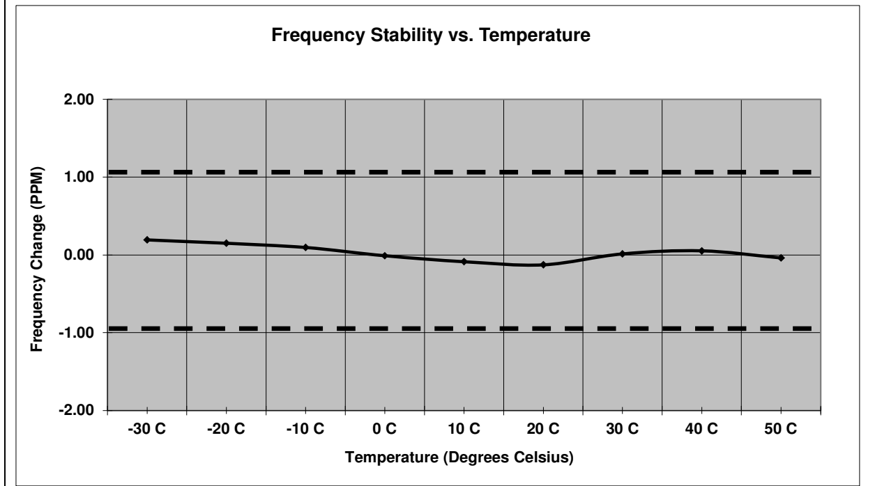
Figure 7.6.2-4: Frequency Stability – 930.5 MHz – TXC
