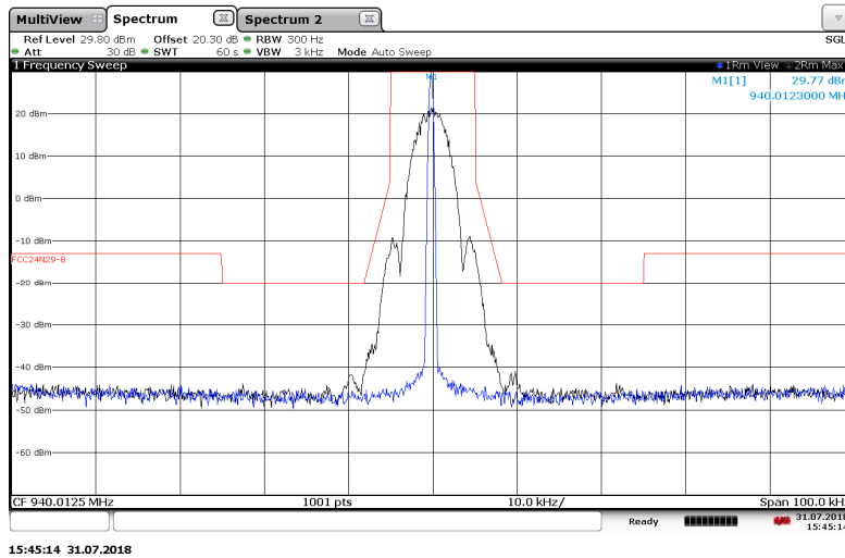
Figure 7.2.2-8: 940.0125 MHz – 12.5 kHz Channel Spacing – mPass 5k Mode
