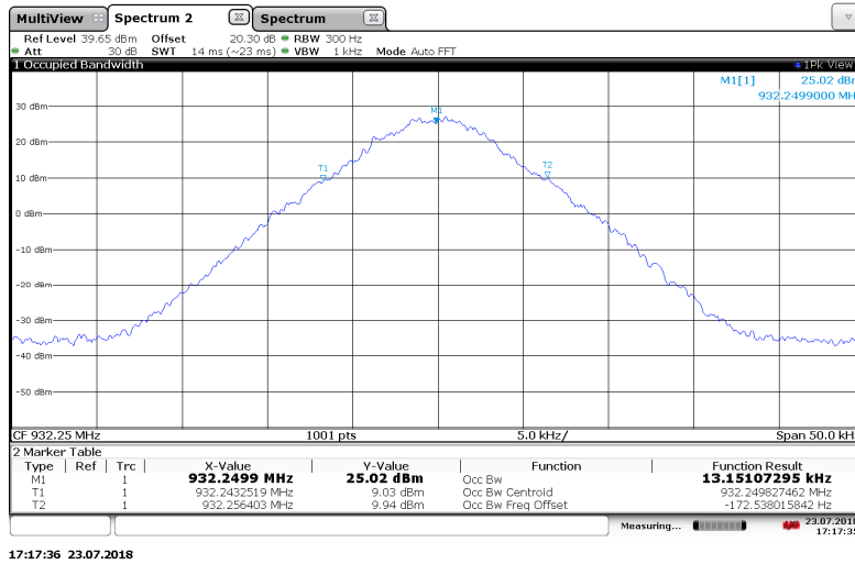
Figure 7.3.2-16: 932.25 MHz – Double Density Mode
