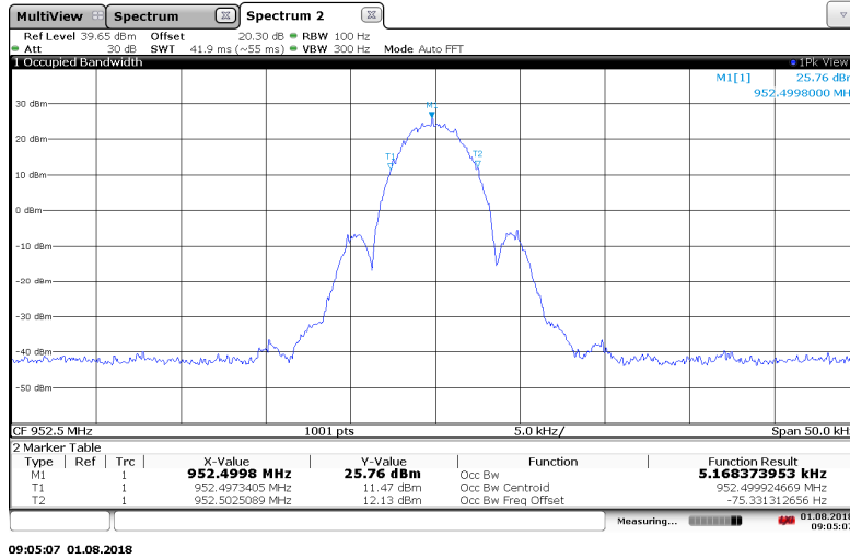
Figure 7.3.2-22: 952.5 MHz – MPass 5k Mode
