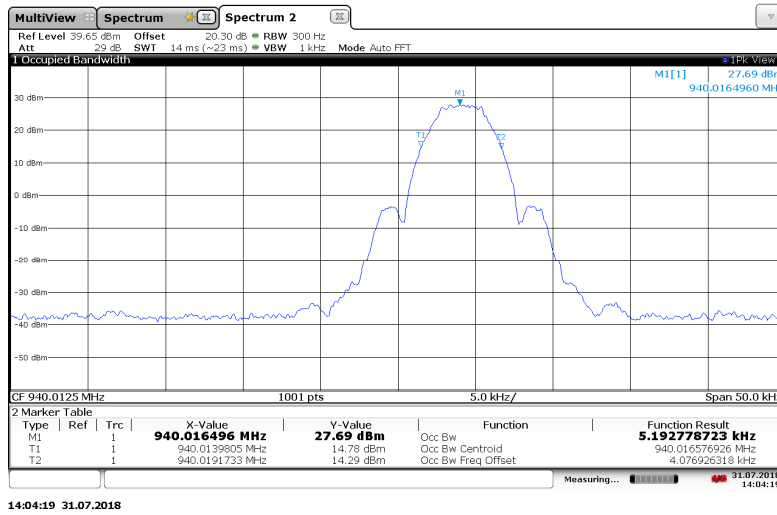
Figure 7.3.2-8: 940.0125 MHz – MPass 5k Mode
