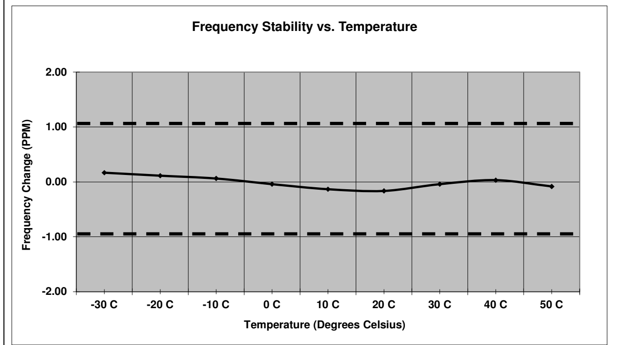
Figure 7.6.2-6: Frequency Stability – 959.925 MHz – TXC
