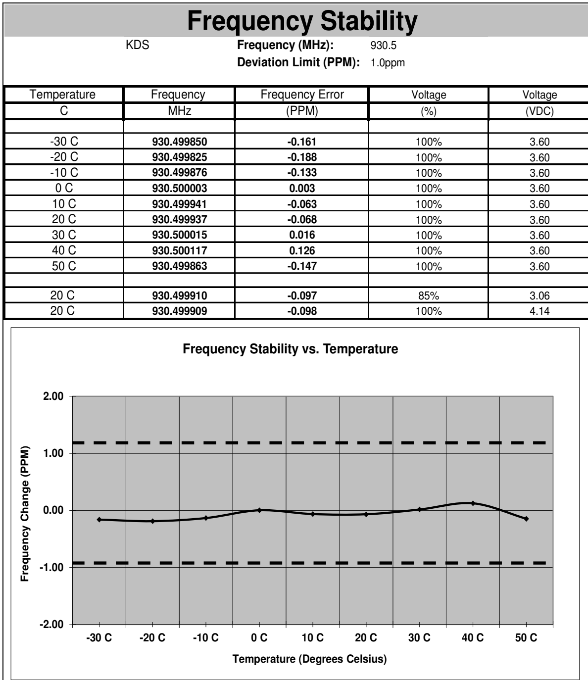
Figure 7.6.2-3: Frequency Stability – 930.5 MHz – KDS
