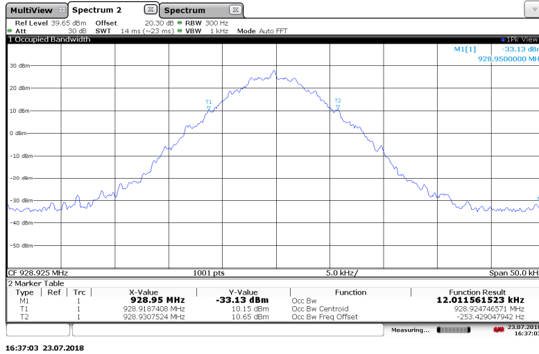
Figure 7.3.2-12: 928.925 MHz – Normal Mode
