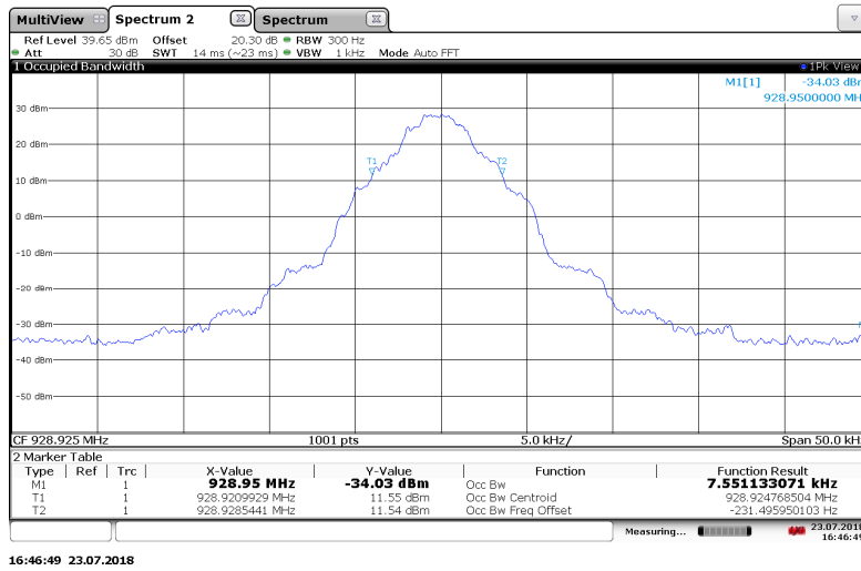
Figure 7.3.2-13: 928.925 MHz – Priority Mode
