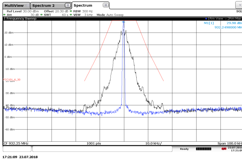
Figure 7.2.2-15: 932.25 MHz – 25 kHz Channel Spacing - C&I Mode
