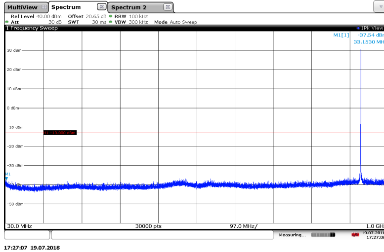
17:27:07 19.07.2018 Figure 7.4.2-3: 930.5 MHz – 30MHz to 1GHz – Mpass5k mode
