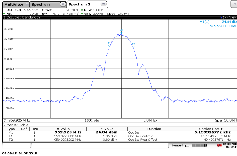
Figure 7.3.2-24: 959.925 MHz– mPass 5k Mode
