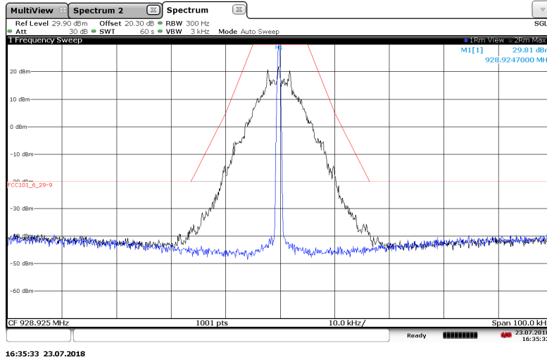
Figure 7.2.2-12: 928.925 MHz – 25 kHz Channel Spacing - Normal Mode
