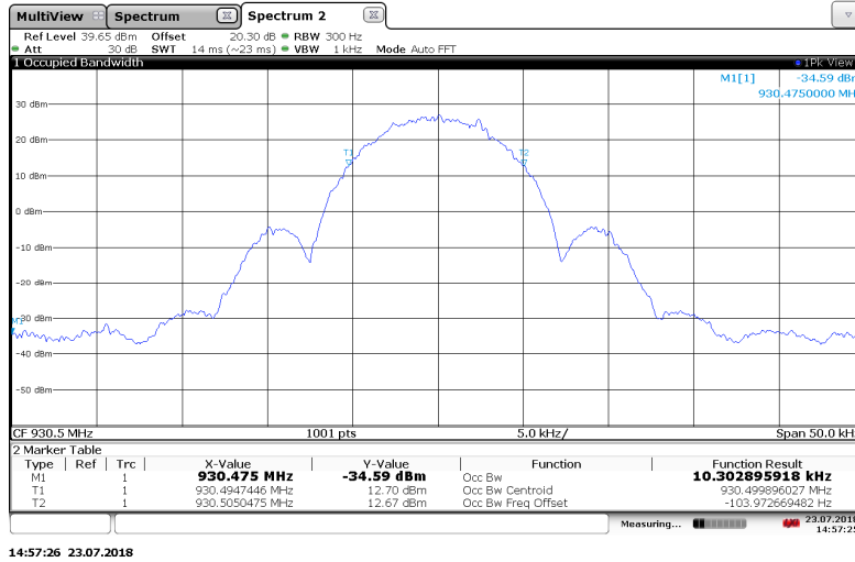
Figure 7.3.2-7: 930.5 MHz – MPass 10k Mode
