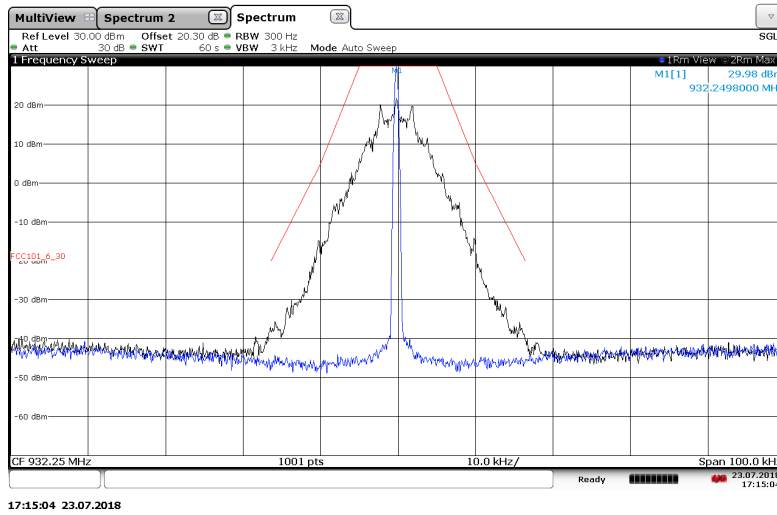
Figure 7.2.2-17: 932.25 MHz – 25 kHz Channel Spacing - Normal Mode
