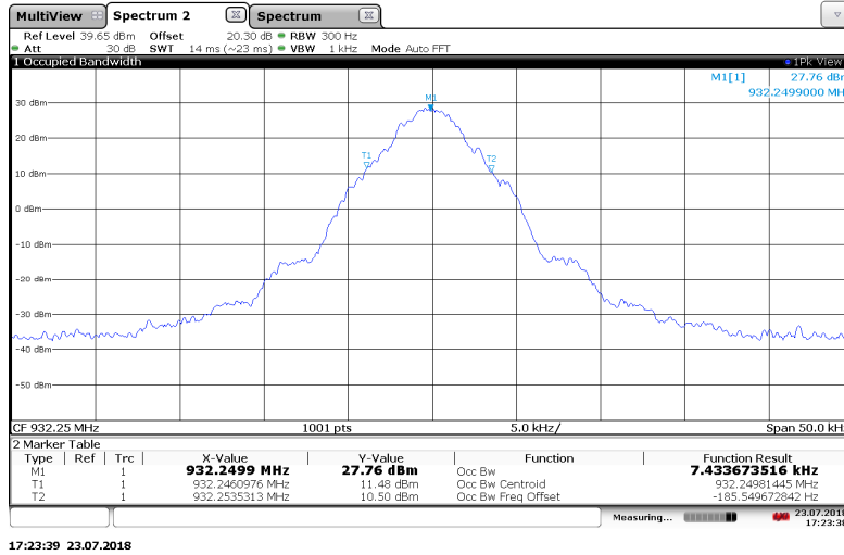
Figure 7.3.2-18: 932.25 MHz — Priority Mode
