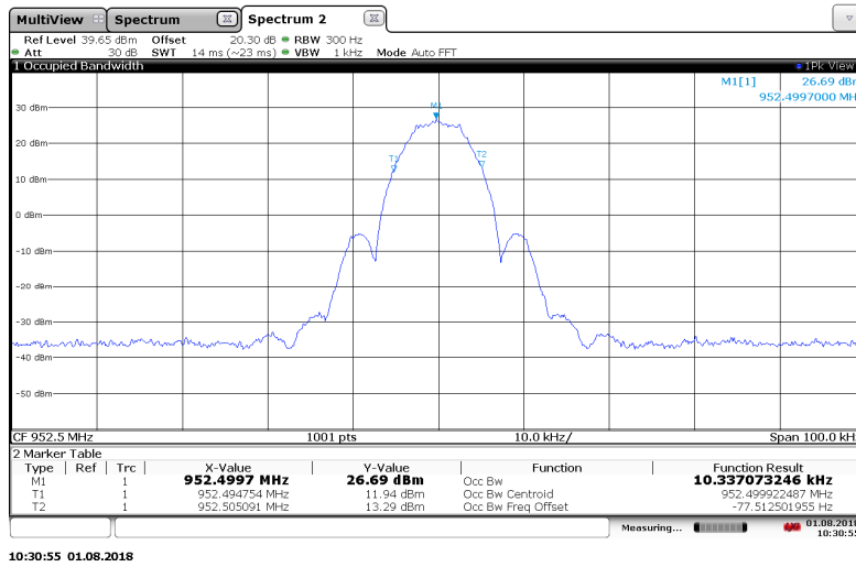
Figure 7.3.2-23: 952.5 MHz – MPass 10k Mode
