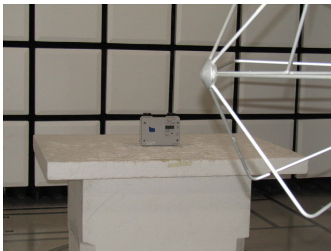
Figure 4: Radiated Emissions – Front – Below 1GHz
