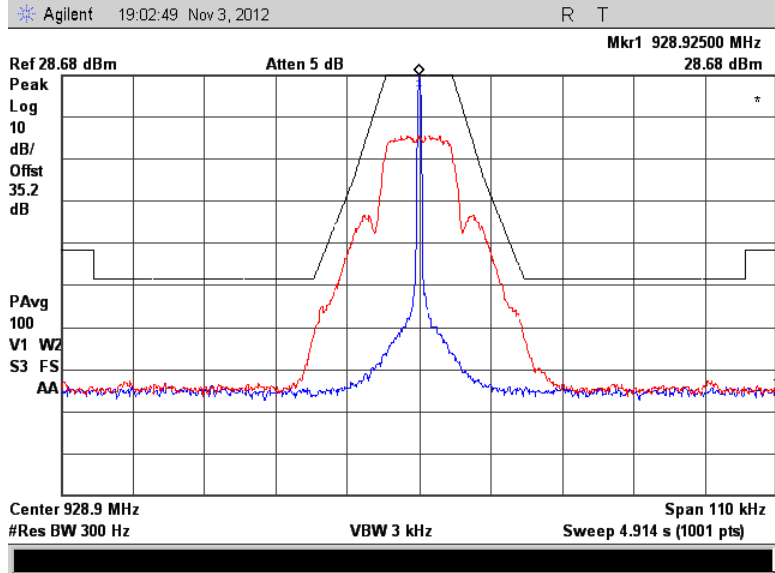
Figure 7.2.2-21: 928.925 MHz – MPass 10k Mode
