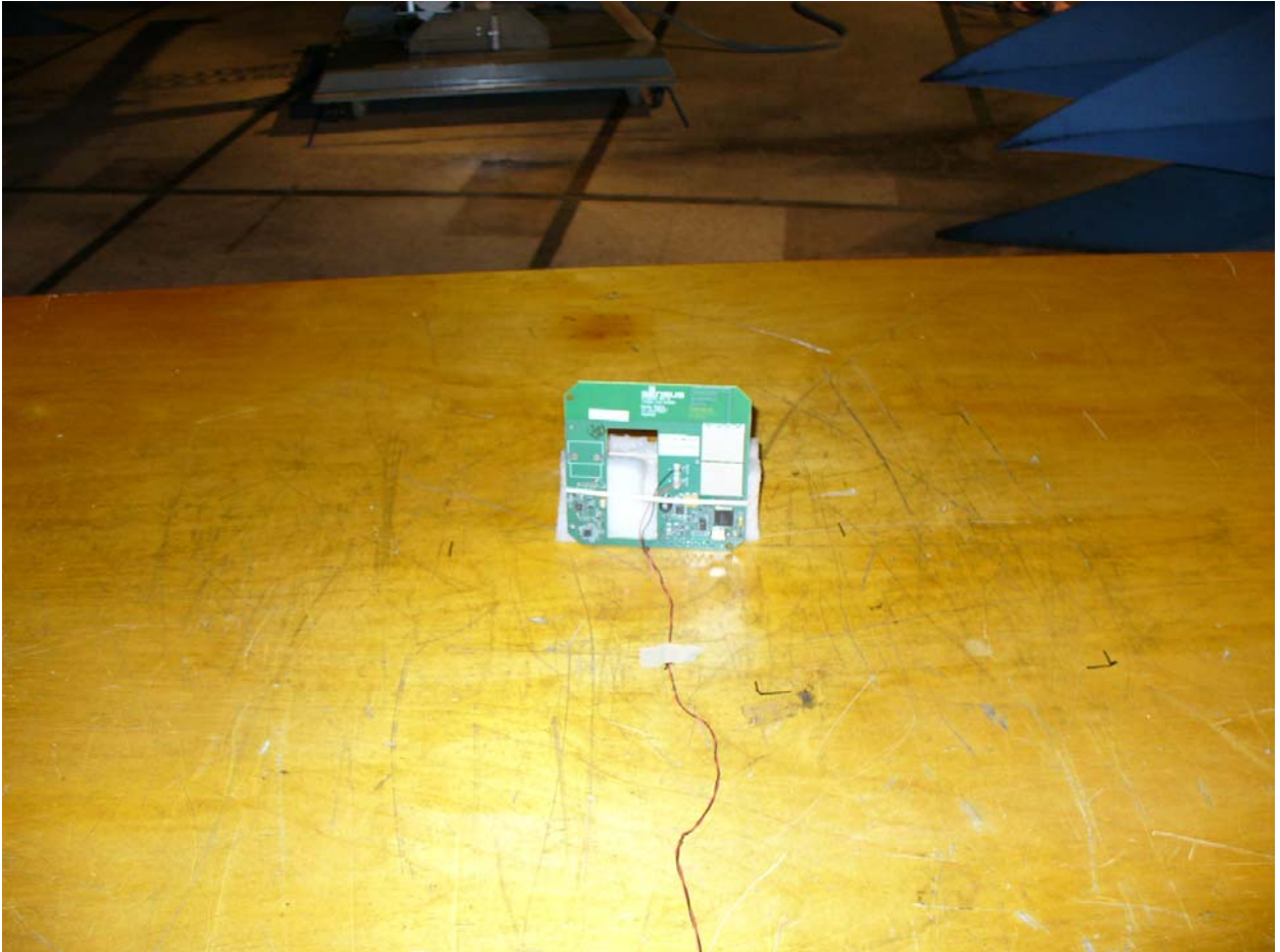
Figure 4: Radiated Emissions – Back View Close Up
