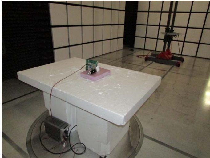
Figure 4: Below 1 GHz
