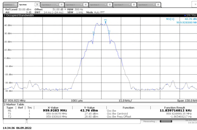
Figure 2.3.6-18: 99% Bandwidth – 959.925 MHz - mPass2 – High Power
