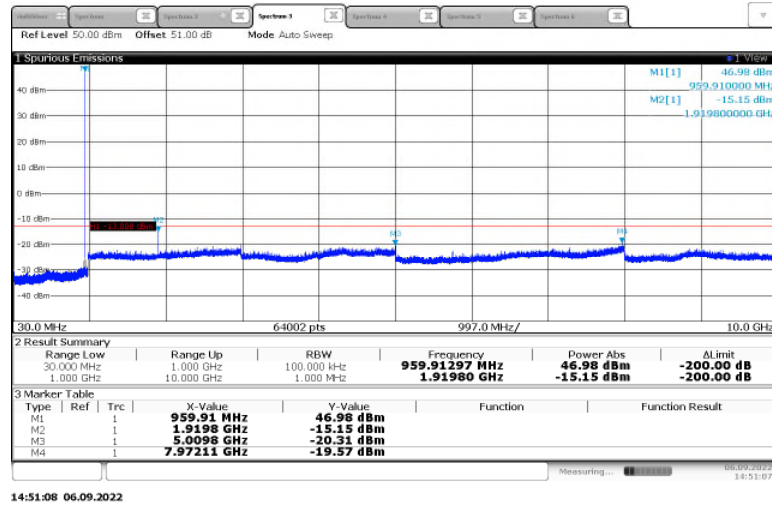
Figure 2.4.6-7: Transmitter Conducted Spurious Emissions – 959.925 MHz - mPass5k Mode – High Power
