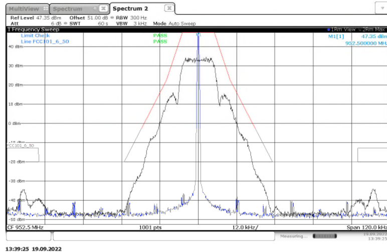
Figure 2.2.6-30: Emissions Mask – 952.5 MHz - 25 kHz Channel Spacing- mPass2 Mode – High Power
