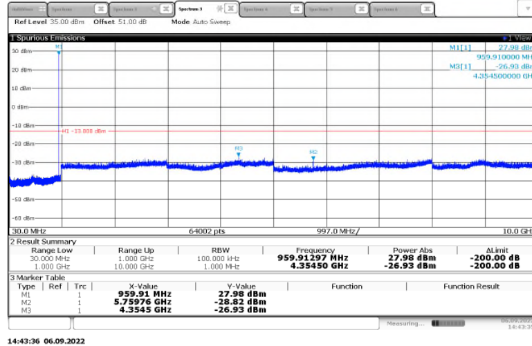
Figure 2.4.6-10: Transmitter Conducted Spurious Emissions – 959.925 MHz - mPass5k Mode – Low Power
