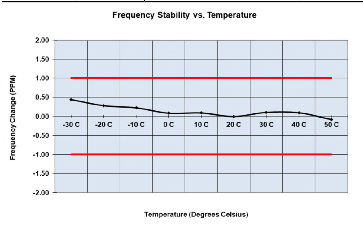
Figure 2.6.6-1: Frequency Stability – 930.5 MHz – High Power
