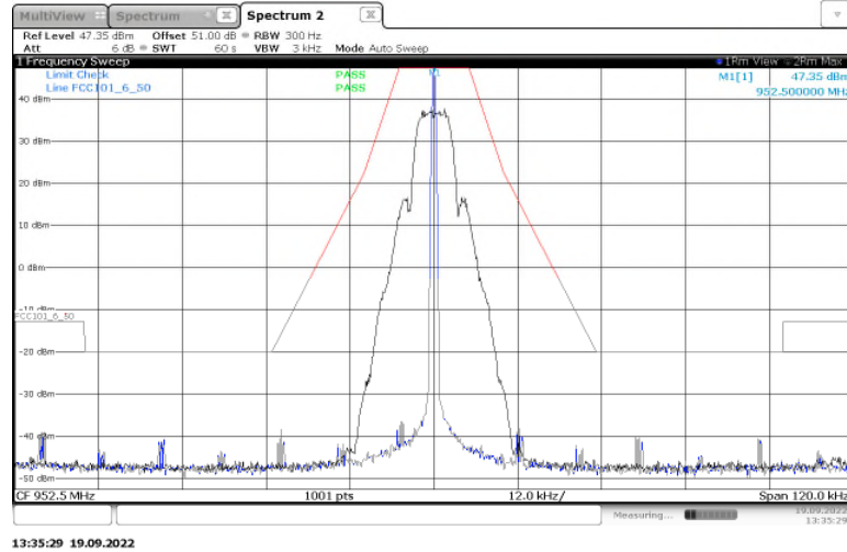
Figure 2.2.6-29: Emissions Mask – 952.5 MHz - 25 kHz Channel Spacing- mPass Mode – High Power
