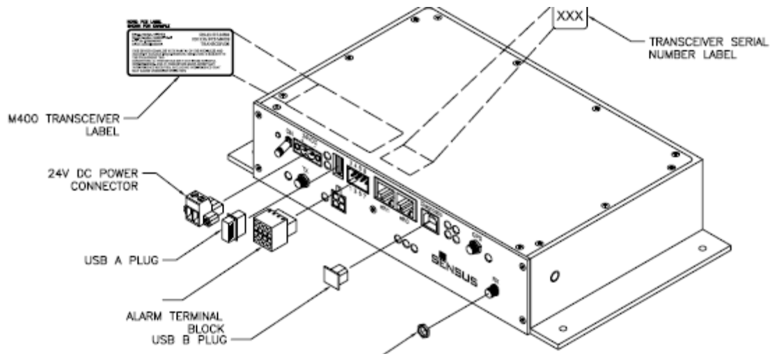
Figure 2: Sample Label Location M400XCVR-01
