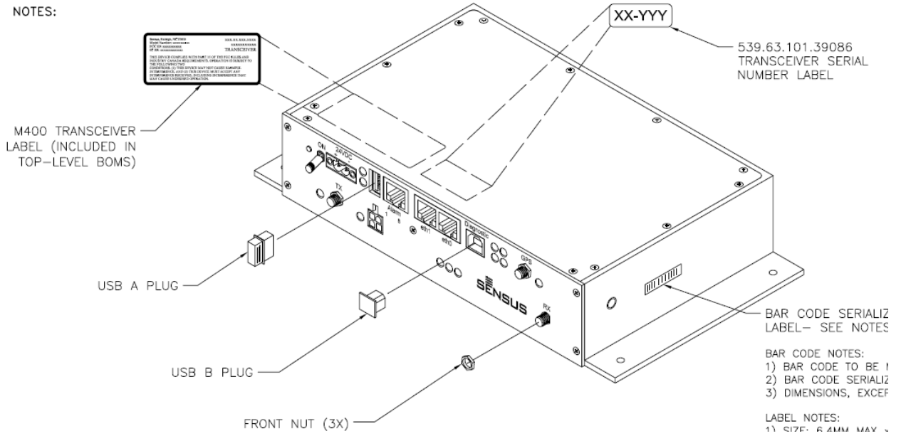
Figure 2: Sample Label Location M400XCVR-00
