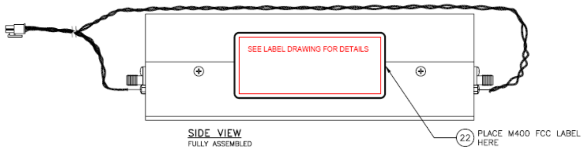
Figure 3: Sample Label Location Power Amplifier
