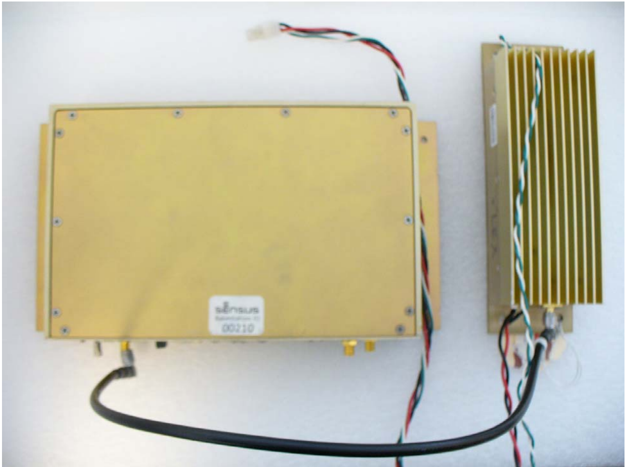
Figure 13: M400XCVR-00 with Power Amplifier (Assembled – Top View)
