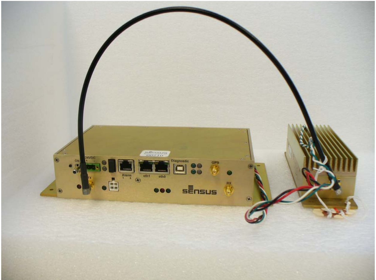
Figure 14: M400XCVR-00 with Power Amplifier (Assembled – Front View)
