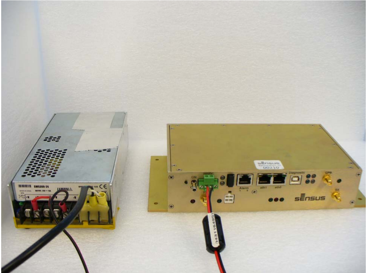
Figure 16: M400XCVR-00 with Ferrite 0431164951 on Power Cord (Assembled – Front View)
