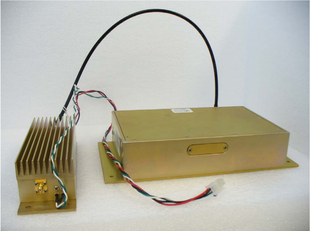
Figure 15: M400XCVR-00 with Power Amplifier (Assembled – Rear View)
