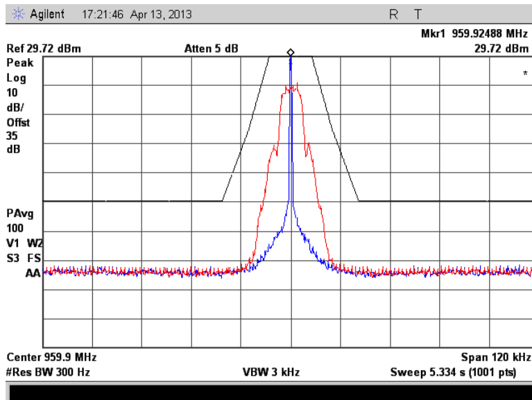
Figure 7.2.2-3: 959.925 MHz – mPass 5k
