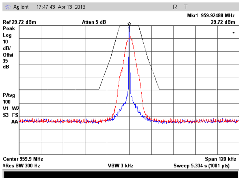
Figure 7.2.2-1: 959.925 MHz – m4Pass 10k
