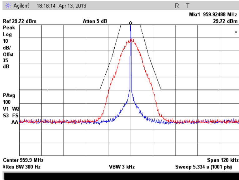
Figure 7.2.2-2: 959.925 MHz – m4Pass 20k
