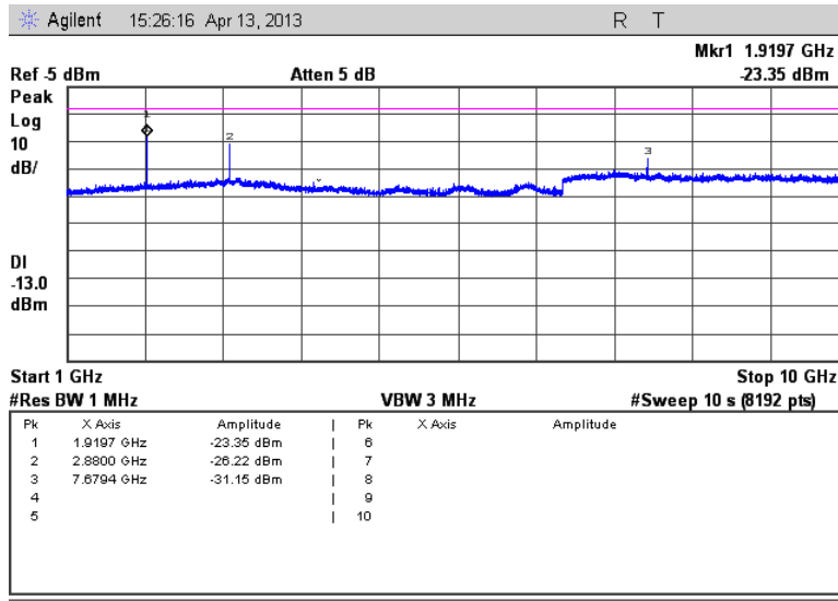
Figure 7.3.2-4: 959.925 MHz – 1GHz to 10GHz
