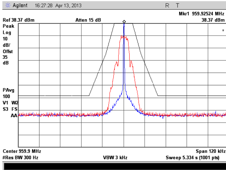
Figure 7.2.2-7: 959.925 MHz – mPass 5k
