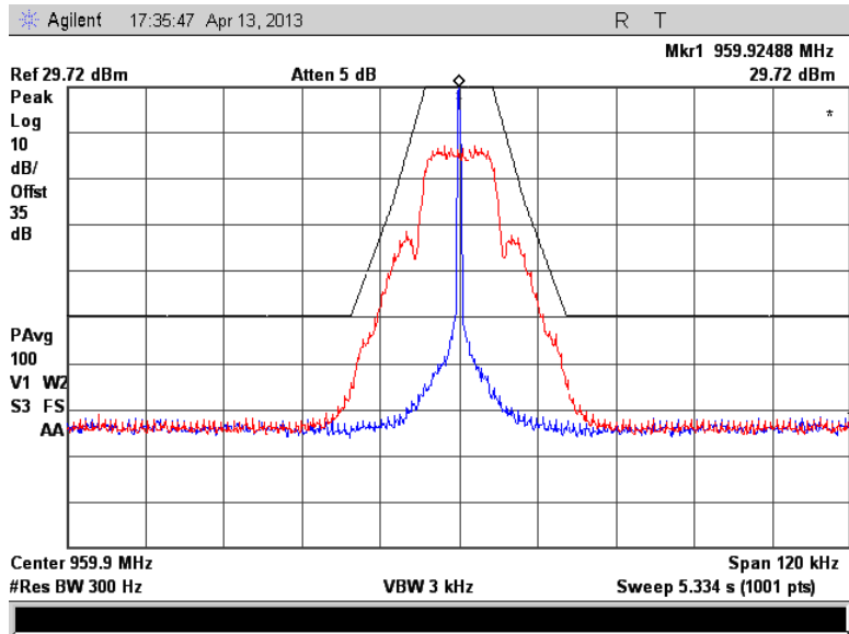
Figure 7.2.2-4: 959.925 MHz – mPass 10k
