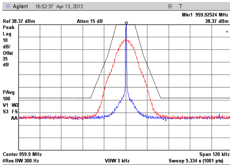
Figure 7.2.2-6: 959.925 MHz – m4Pass 20k
