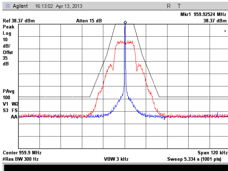
Figure 7.2.2-8: 959.925 MHz – mPass 10k
