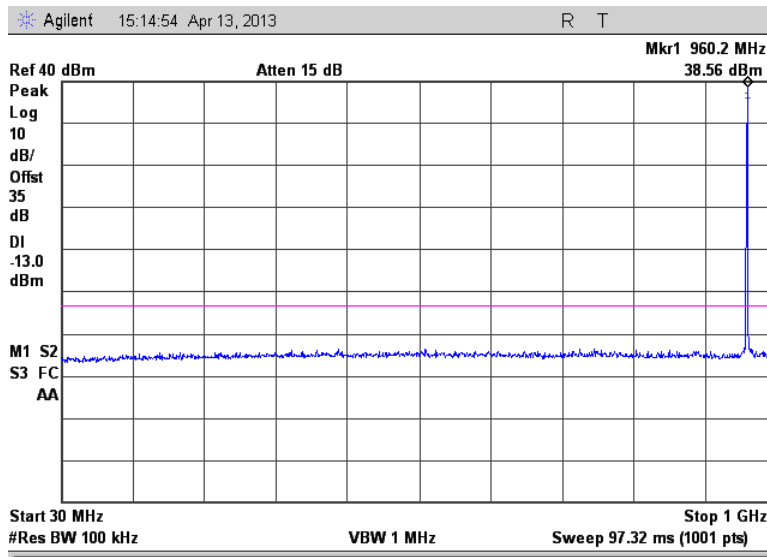
Figure 7.3.2-3: 959.925 MHz – 30MHz to 1GHz
