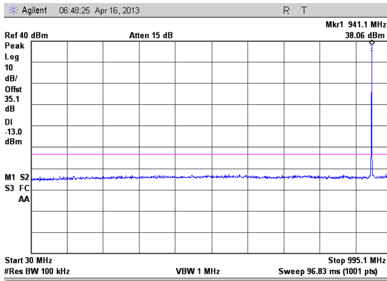
Figure 7.3.2-3: 941.125 MHz – 30MHz to 1GHz
