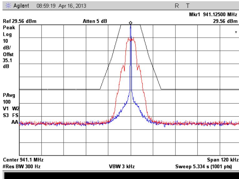
Figure 7.2.2-3: 941.125 MHz – mPass 5k
