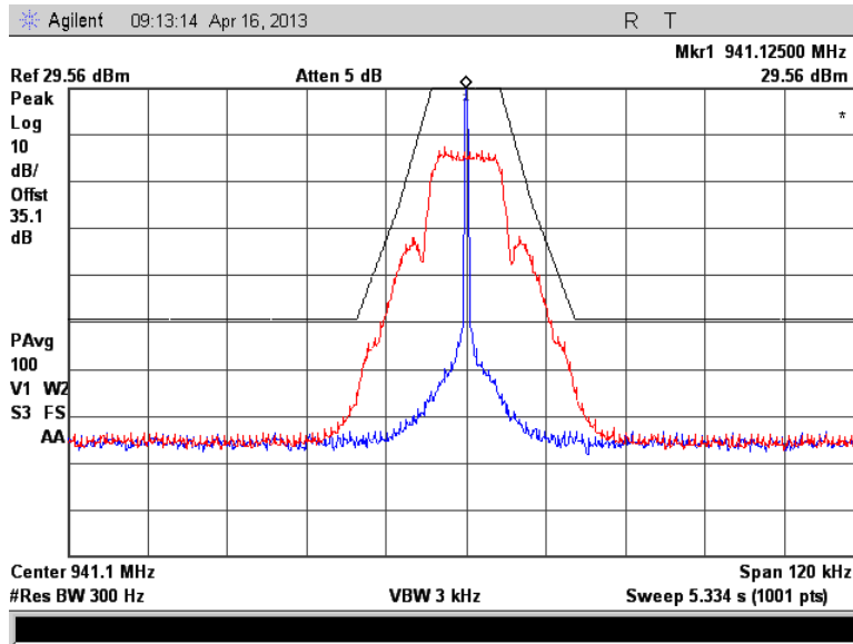
Figure 7.2.2-4: 941.125 MHz – mPass 10k
