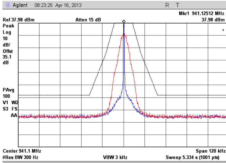
Figure 7.2.2-5: 941.125 MHz – m4Pass 10k
