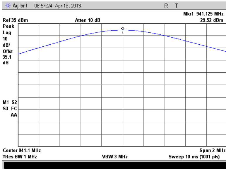
Figure 7.1.2-1: Peak Output Power – 941.125 MHz
