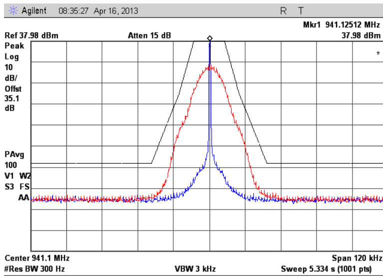
Figure 7.2.2-6: 941.125 MHz – m4Pass 20k
