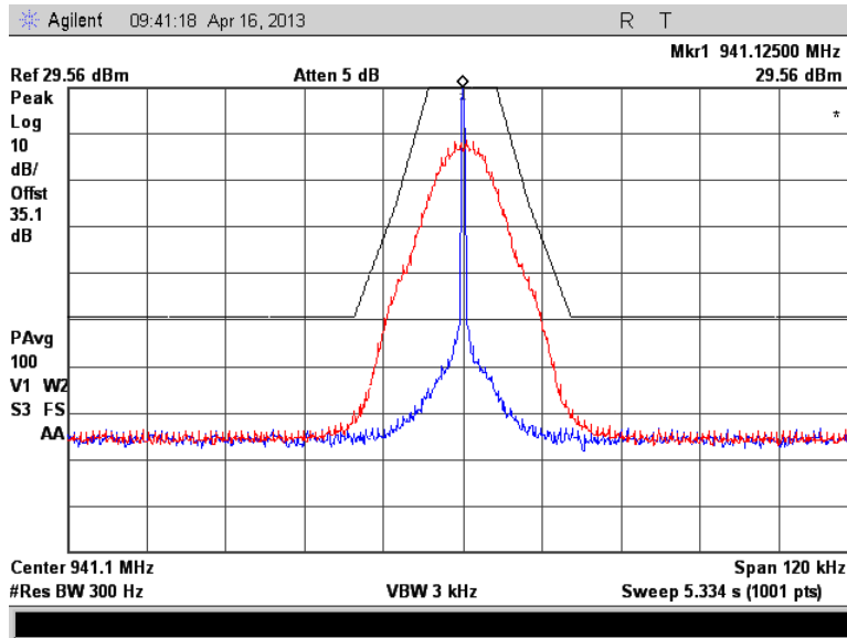
Figure 7.2.2-2: 941.125 MHz – m4Pass 20k
