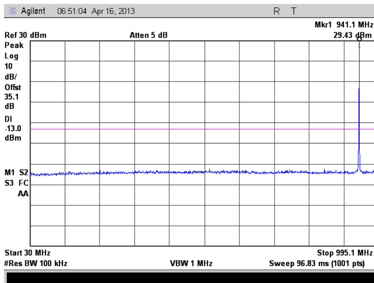
Figure 7.3.2-1: 941.125 MHz – 30MHz to 1GHz
