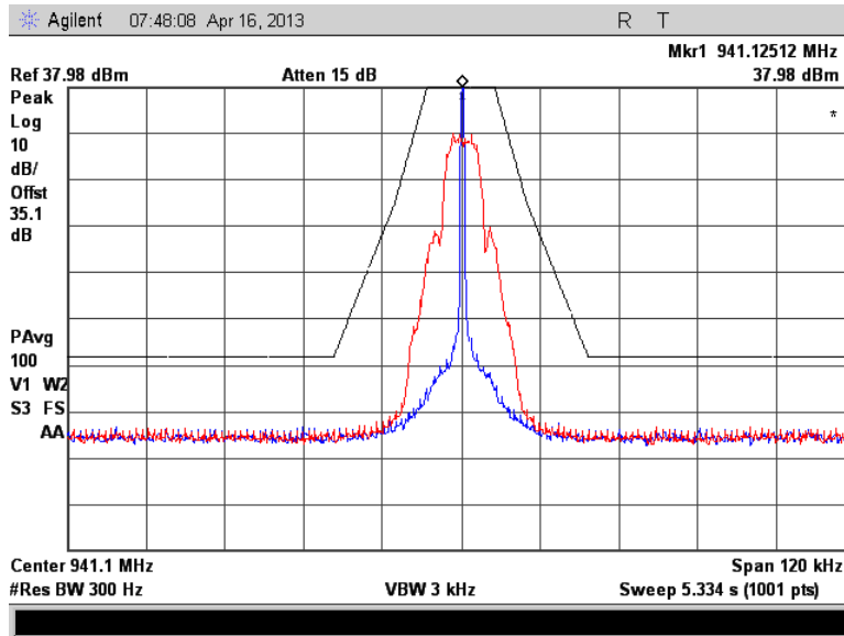
Figure 7.2.2-7: 941.125 MHz – mPass 5k
