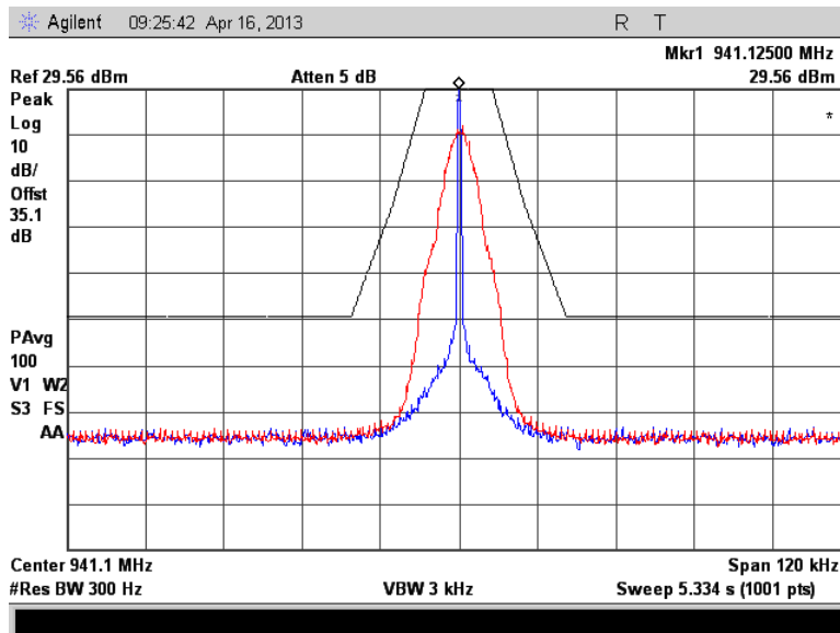
Figure 7.2.2-1: 941.125 MHz – m4Pass 10k
