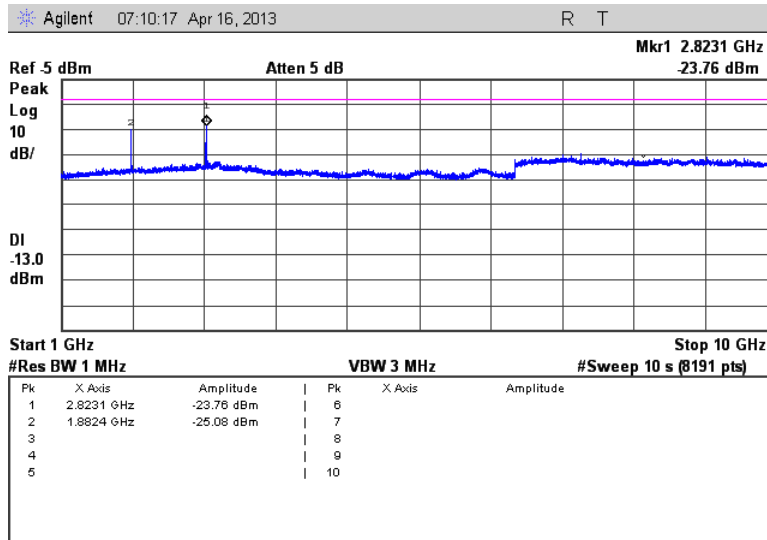
Figure 7.3.2-4: 941.125 MHz – 1GHz to 10GHz
