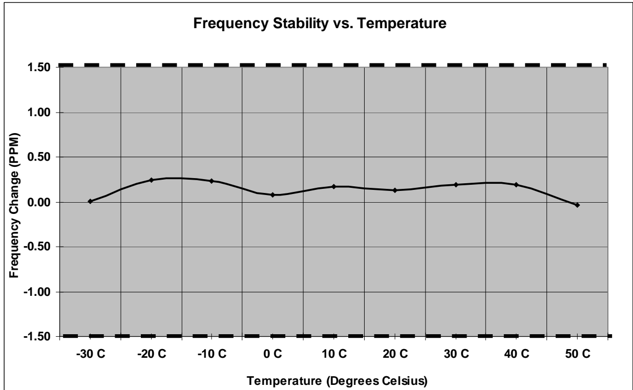
Figure 7.5.2-1: Frequency Stability – 941.125 MHz
