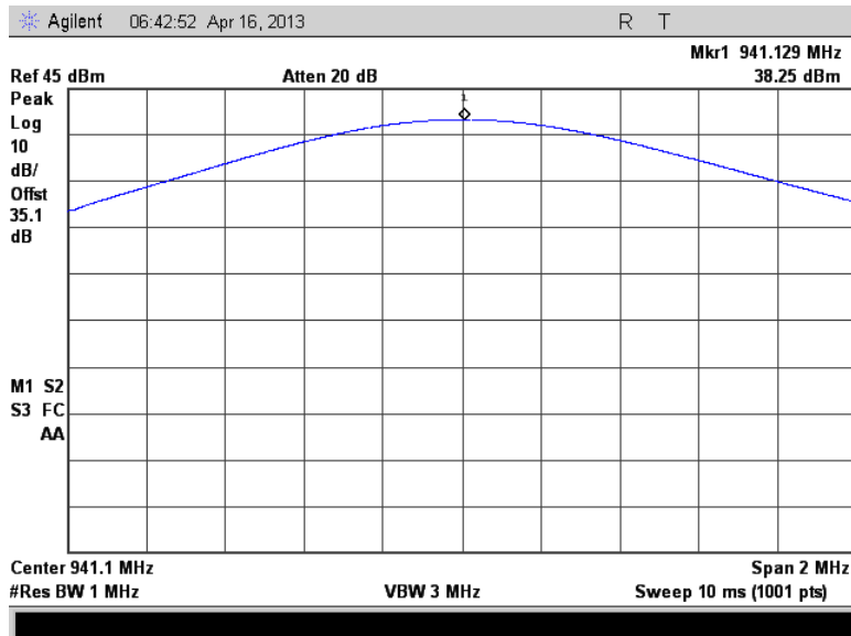
Figure 7.1.2-2: Peak Output Power - 941.125 MHz
