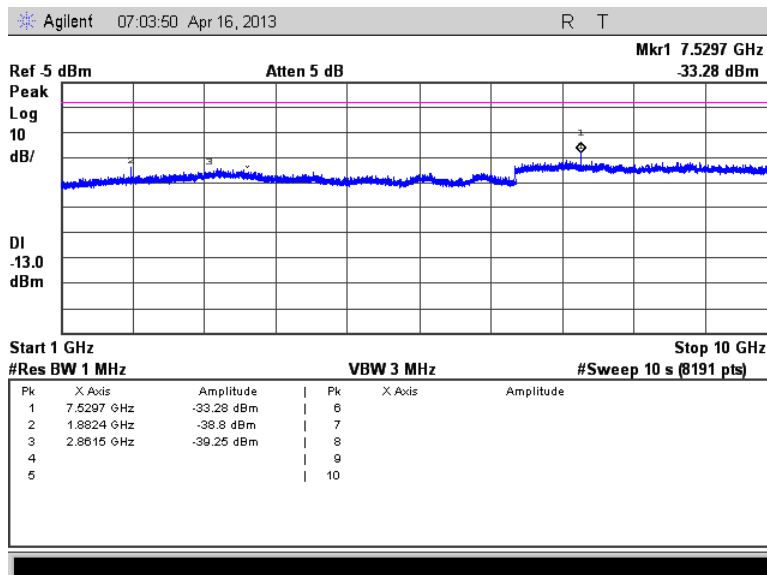
Figure 7.3.2-2: 941.125 MHz – 1GHz to 10GHz
