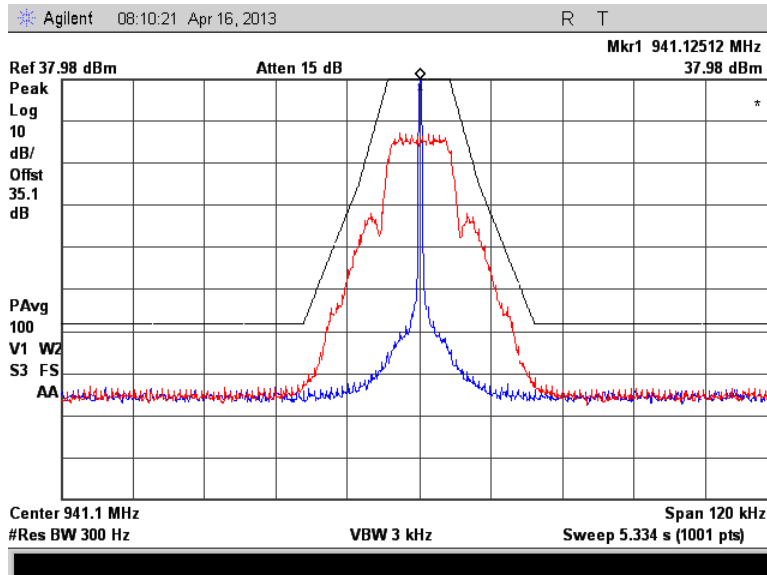
Figure 7.2.2-8: 941.125 MHz – mPass 10k
