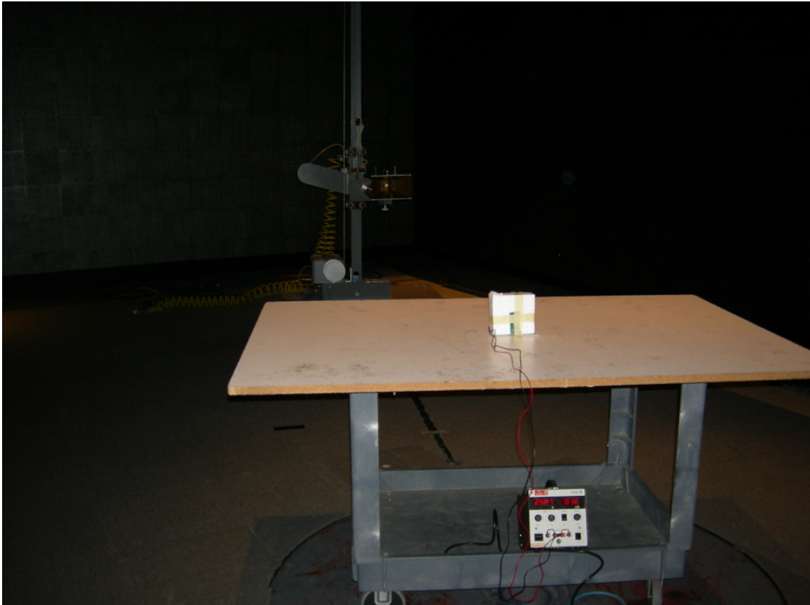
Figure 1: Radiated Emissions
