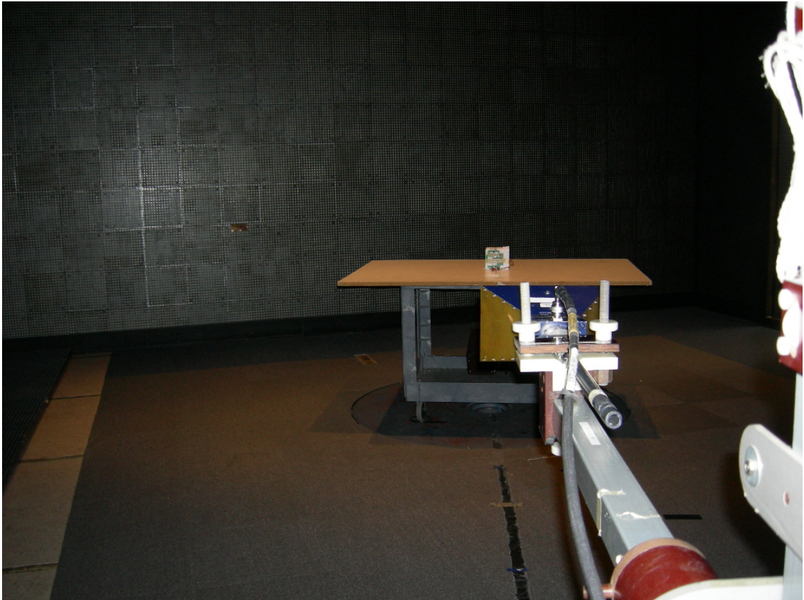
Figure 3: Radiated Emissions
