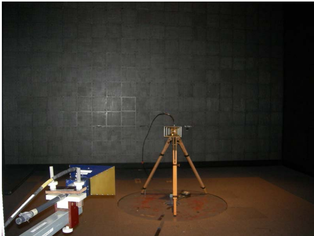
Figure 3: Radiated Emissions - Substitution
