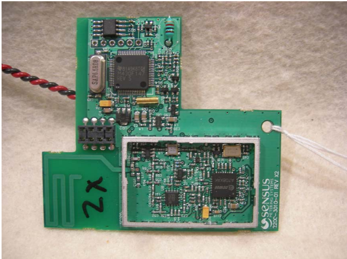
Figure 2: PCB without Shields – Front
