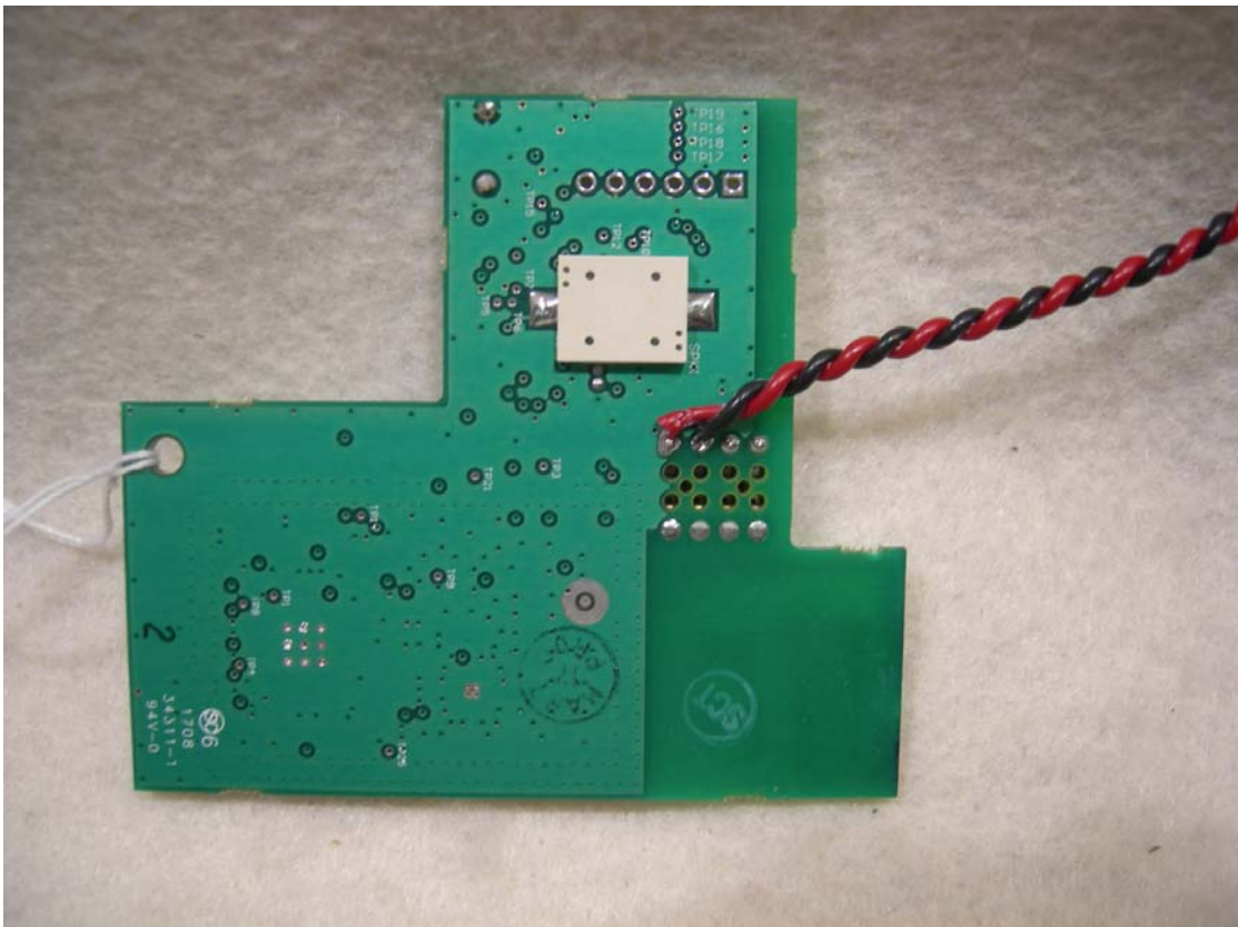
Figure 3: PCB - Back
