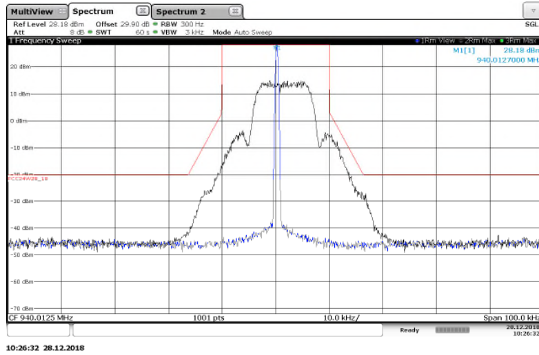
Figure 7.2.2-9: 940.0125 MHz – 25 kHz Channel Spacing – mPass 10k Mode
