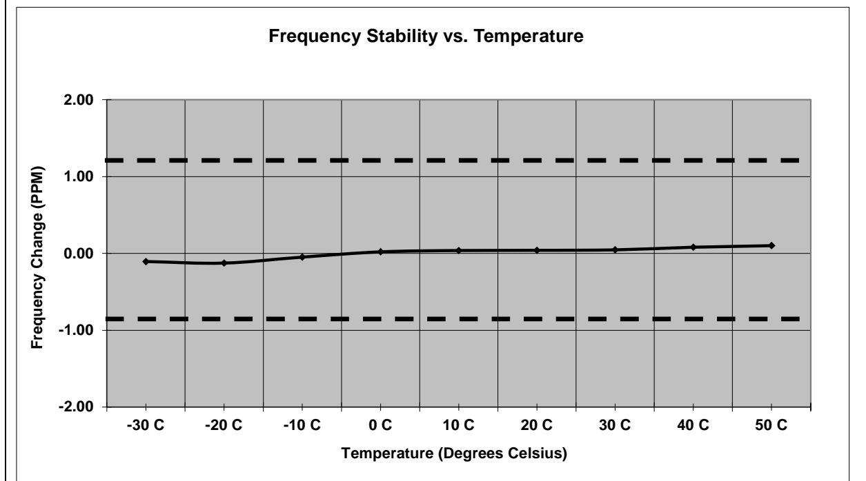
Figure 7.6.2-5: Frequency Stability – 930.5 MHz – ILSI
