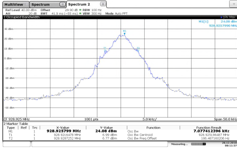
Figure 7.3.2-13: 928.925 MHz – Priority Mode
