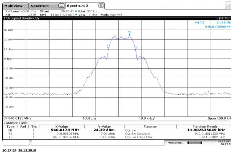
Figure 7.3.2-9: 940.0125 MHz – MPass 10k Mode
