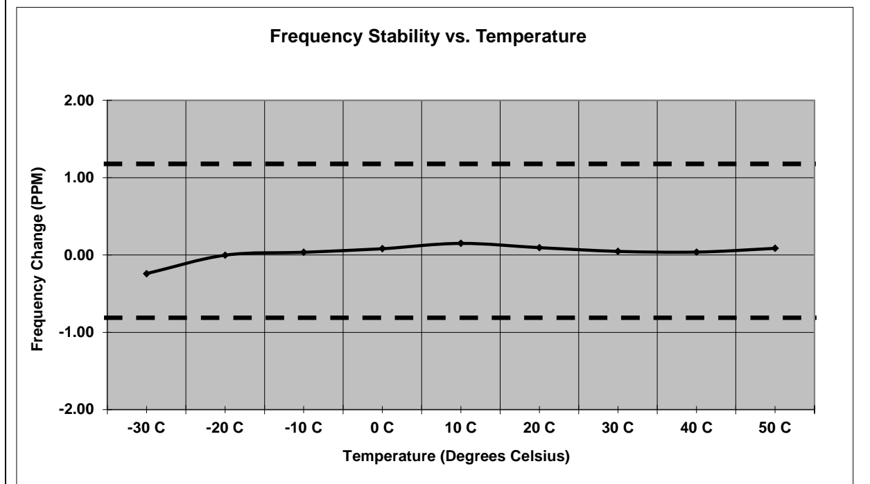
Figure 7.6.2-8: Frequency Stability – 959.925 MHz – ILSI
