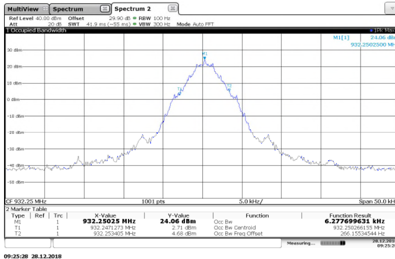
Figure 7.3.2-17: 932.25 MHz – C&I (Half Baud) Mode
