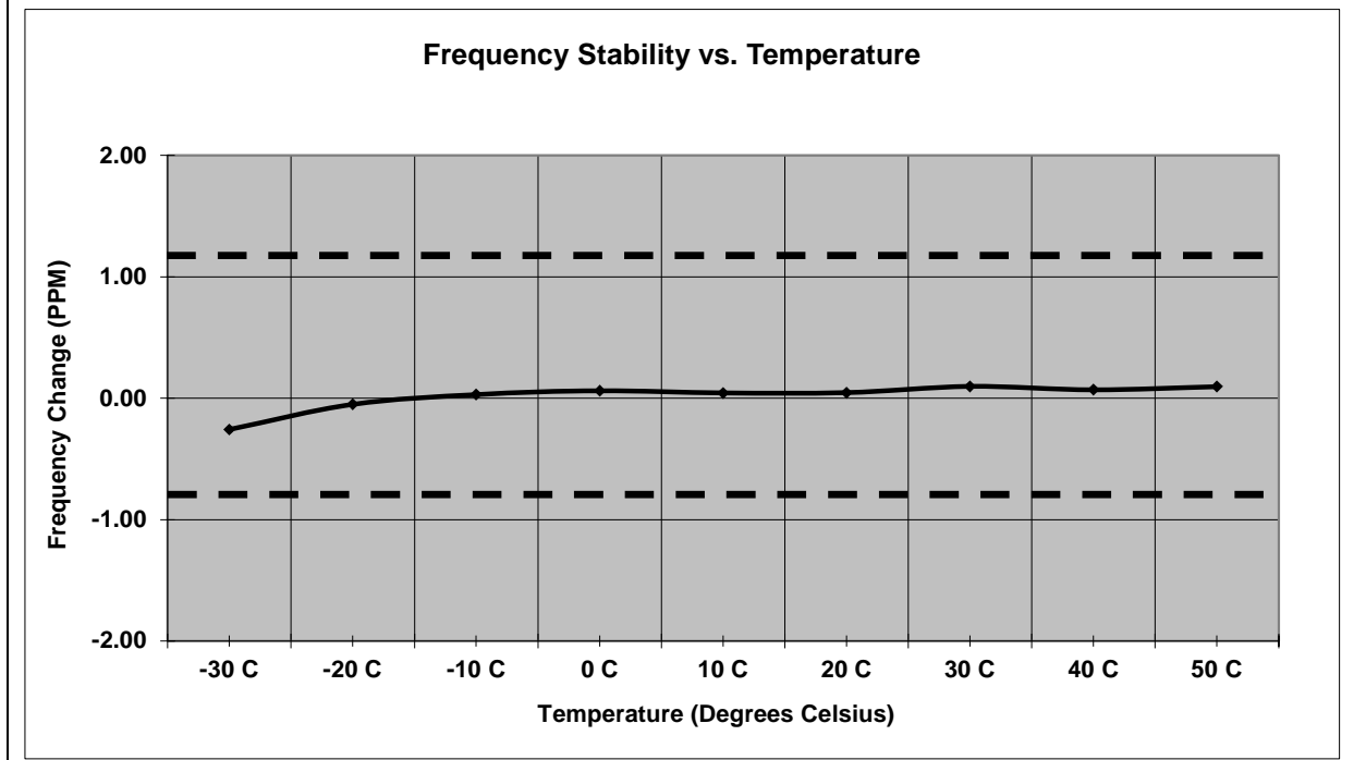
Figure 7.6.2-2: Frequency Stability – 901.5 MHz – ILSI
