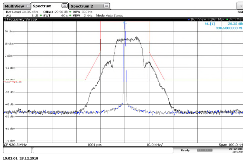
Figure 7.2.2-7: 930.5 MHz –25 kHz Channel Spacing – mPass 10k Mode
