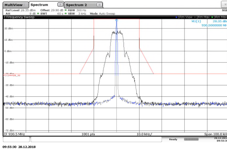
Figure 7.2.2-6: 930.5 MHz – 25 kHz Channel Spacing – mPass 5k Mode
