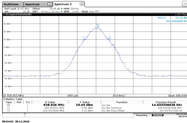
Figure 7.3.2-11: 928.925 MHz – Double Density Mode
