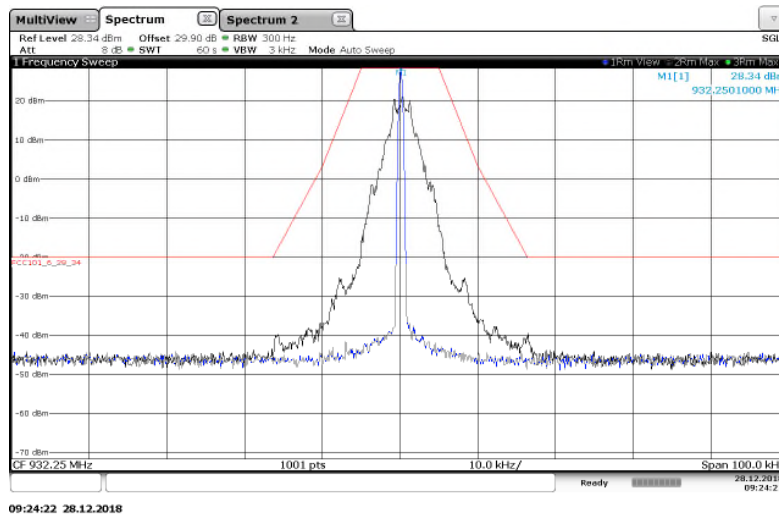
Figure 7.2.2-17: 932.25 MHz – 25 kHz Channel Spacing – C&I (Half Baud) Mode
