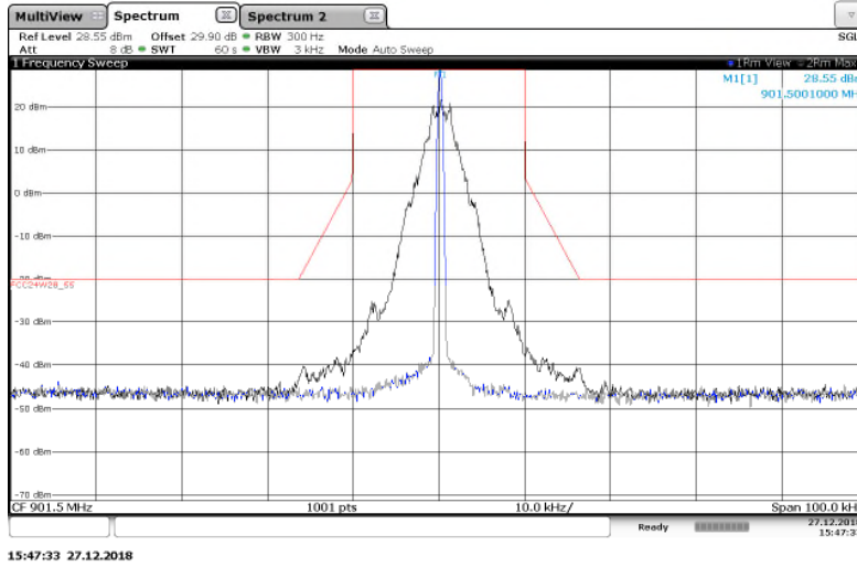
Figure 7.2.2-3: 901.5 MHz – 25 kHz Channel Spacing – C&I (Half Baud) Mode
