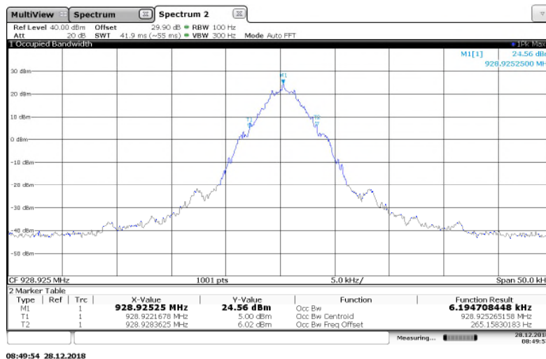
Figure 7.3.2-12: 928.925 MHz – C&I (Half Baud) Mode
