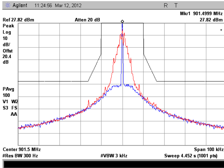
Figure 7.2.2-4: 901.5 MHz – 25 kHz Channel Spacing – C&I Mode
