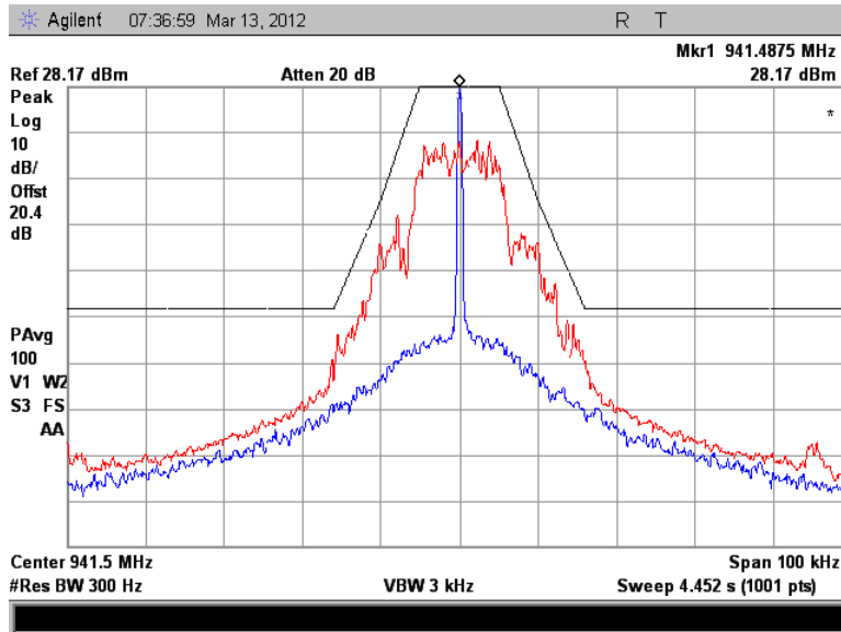
Figure 7.2.2-26: 941.4875 MHz – MPass 10k Mode
