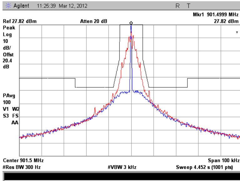
Figure 7.2.2-3: 901.5 MHz – 12.5 kHz Channel Spacing – C&I Mode
