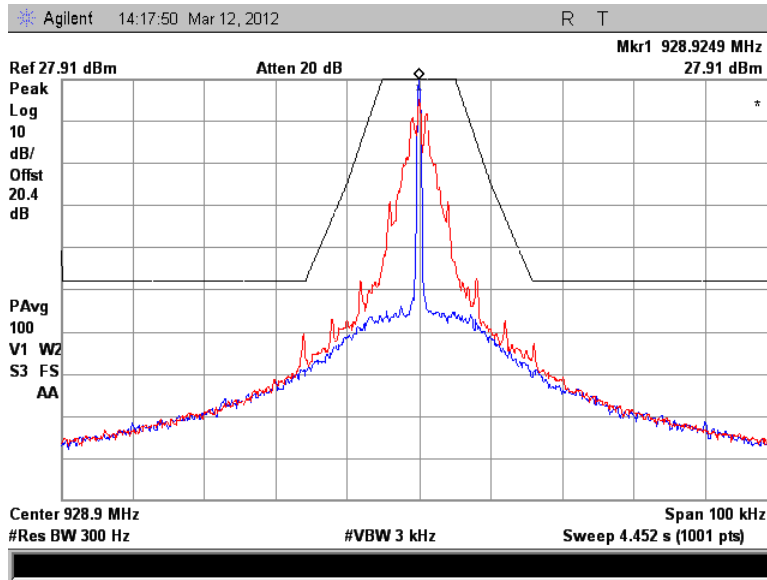
Figure 7.2.2-16: 928.925 MHz – C&I Mode
