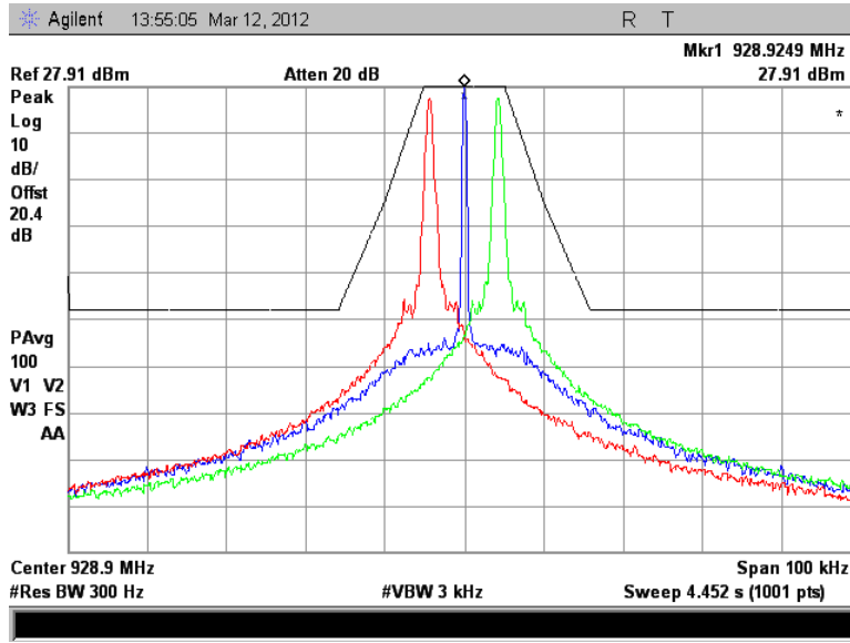
Figure 7.2.2-15: 928.925 MHz – Boost Mode Offset Channel of +/- 7 (+/- 4200 Hz)
