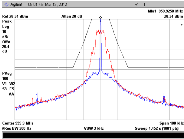
Figure 7.2.2-27: 959.925 MHz – MPass 5k Mode
