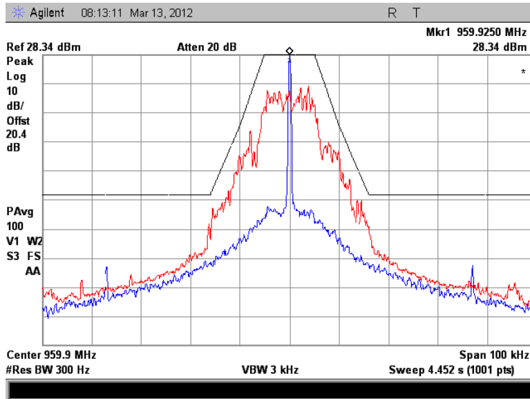
Figure 7.2.2-28: 959.925 MHz – MPass 10k Mode
