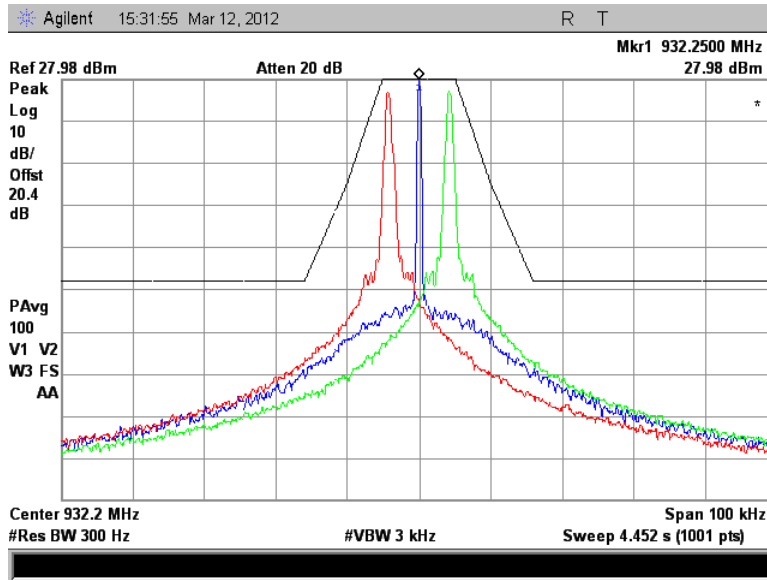
Figure 7.2.2-20: 932.25 MHz – Boost Mode Offset Channel of +/- 7 (+/- 4200 Hz)
