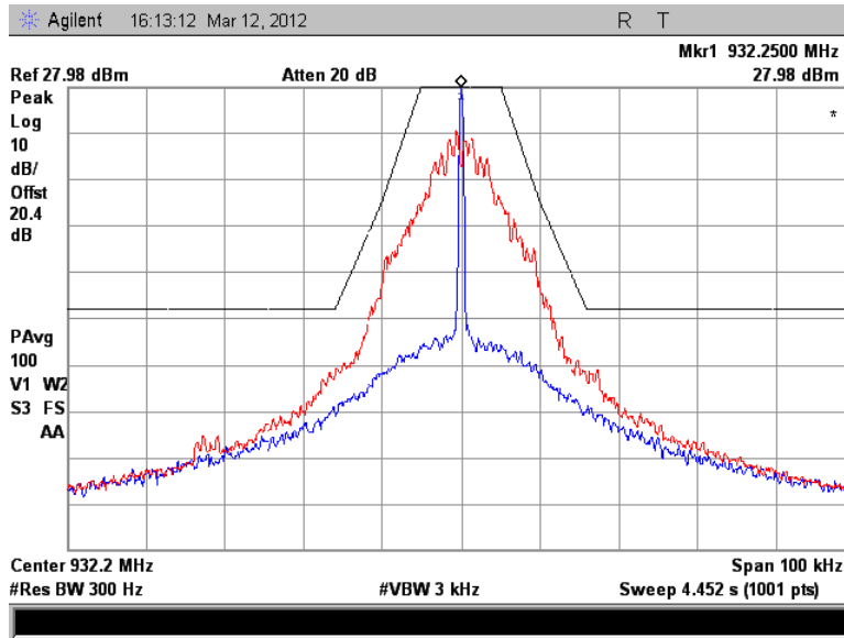
Figure 7.2.2-22: 932.25 MHz – Double Density Mode
