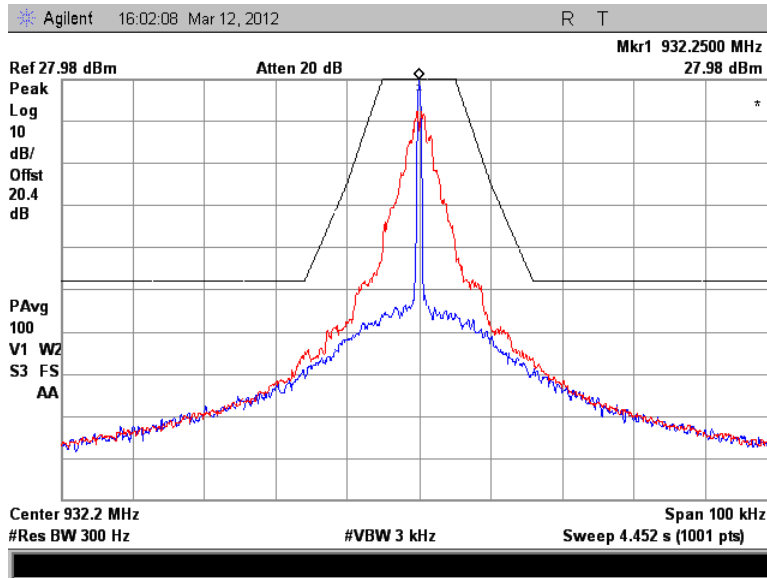
Figure 7.2.2-24: 932.25 MHz — Priority Mode
