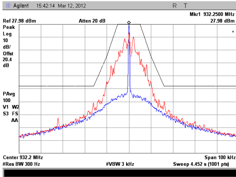
Figure 7.2.2-23: 932.25 MHz – Normal Mode
