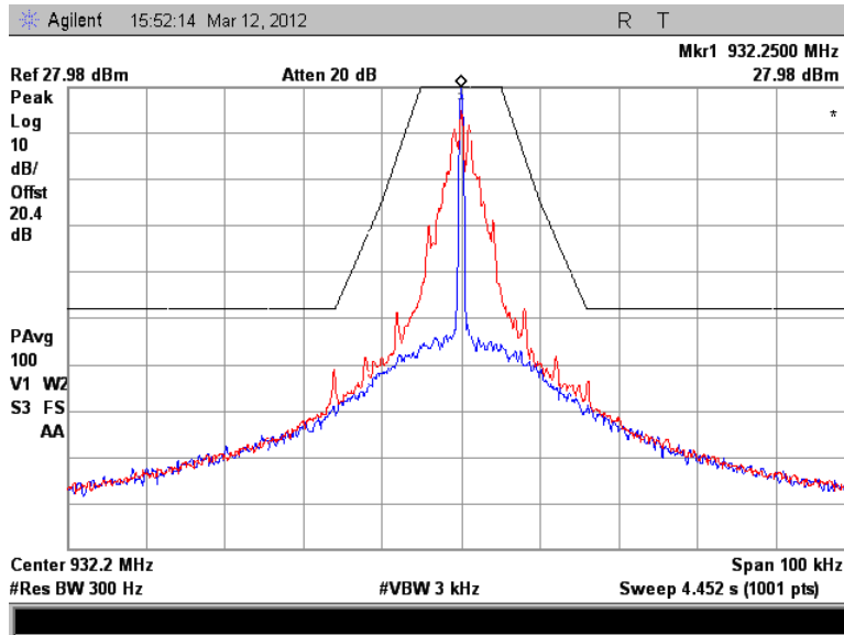
Figure 7.2.2-21: 932.25 MHz – C&I Mode
