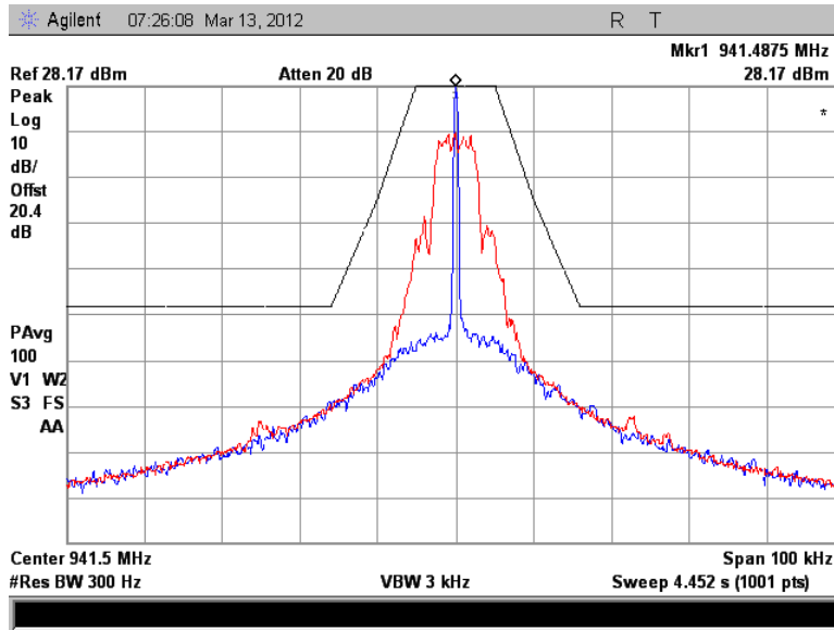
Figure 7.2.2-25: 941.4875 MHz – MPass 5k Mode
