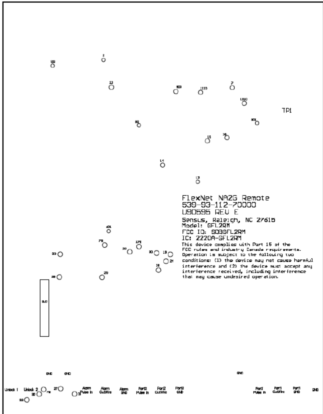
Figure 2: Sample Label/Location (Bottom PCB)
