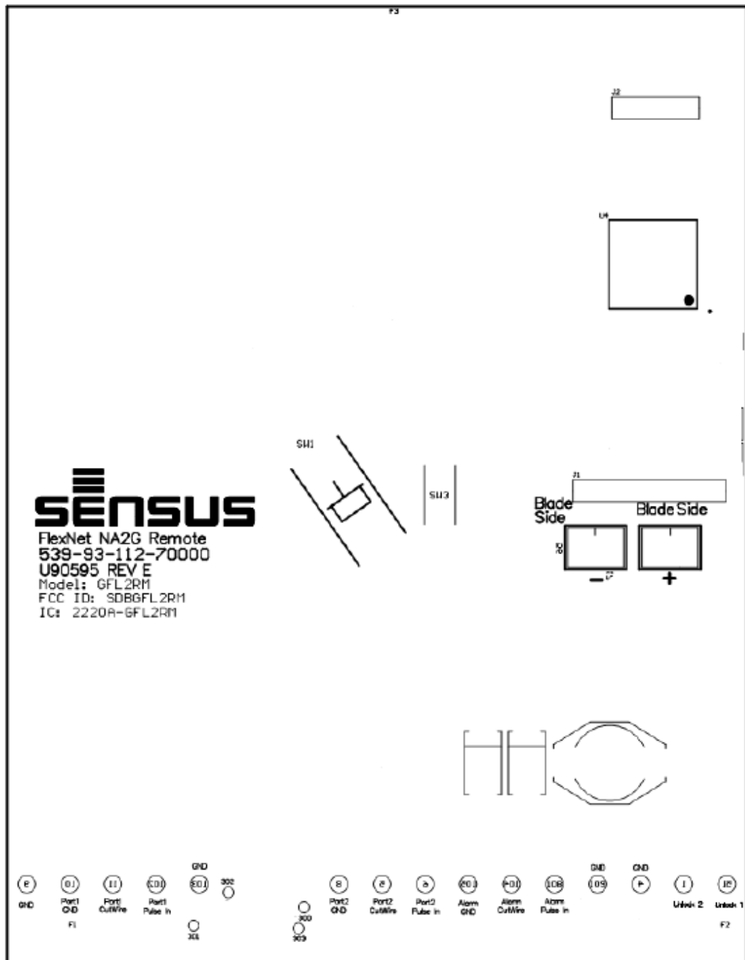
Figure 1: Sample Label/Location (Top PCB)
